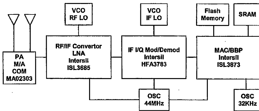
IEEE802.11b WLAN PCMCIA Card WN3301F/G Block Diagram
