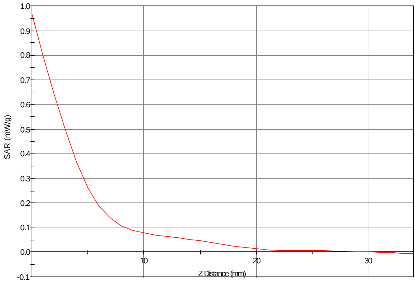
SAR - Z Axis at Hotspot x:-40.0 y:0.0
