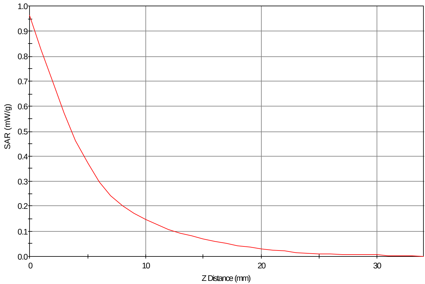
SAR - Z Axis at Hotspot x:53.0 y:-4.0
