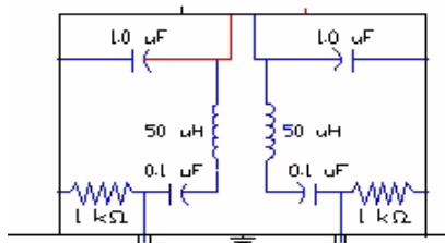
Figure 7. LISN Schematic Diagram
