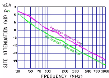
Figure 6. Normalized Site Attenuation Curves (H&V)
