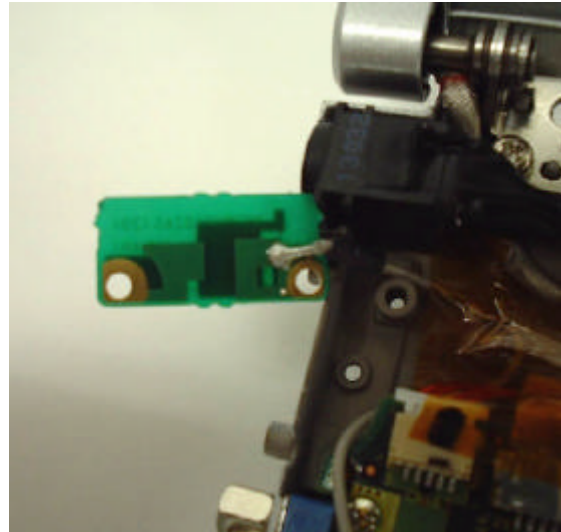
Left Antenna Bottom View
