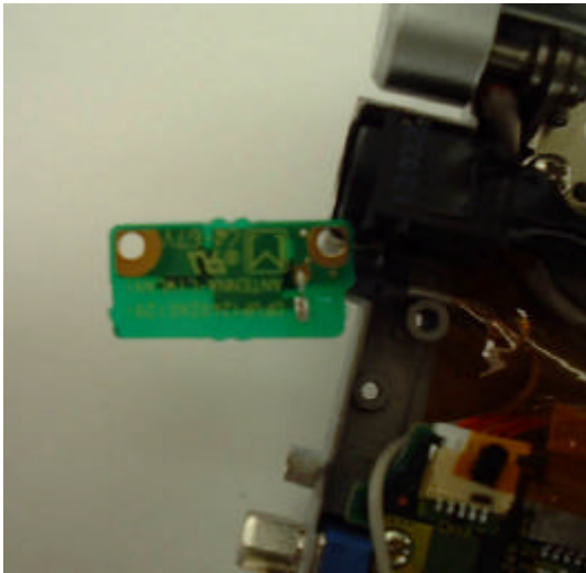
Left Antenna Top View
