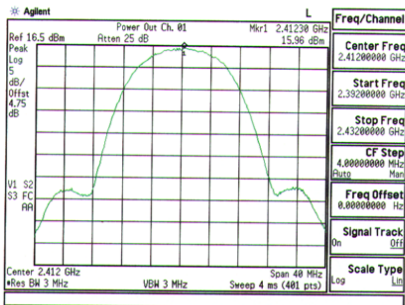
Plot A-4. FCC ID: ACJ9TGCF-T21 Max. Peak Output Power Plot – Ch. 01
