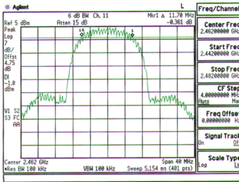
Plot A-3. FCC ID: ACJ9TGCF-T21 6dB Bandwidth Plot – Ch. 11
