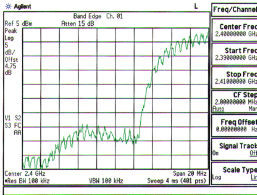
Plot A-10. FCC ID: ACJ9TGCF-T21 Occupied Band Edge Plot – Ch. 01
