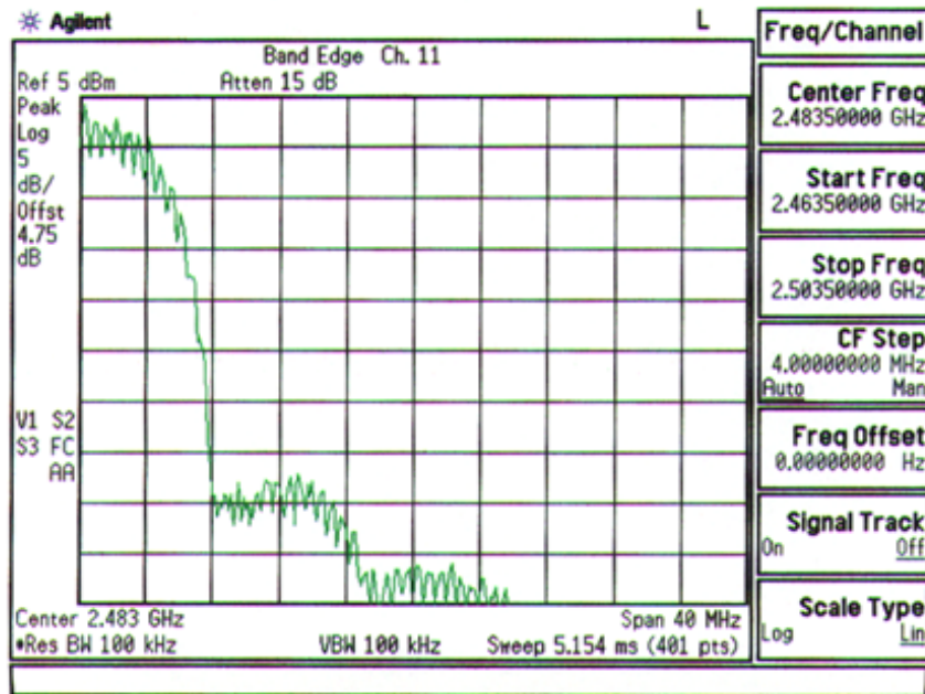
Plot A-11. FCC ID: ACJ9TGCF-T21 Occupied Band Edge Plot – Ch. 11
