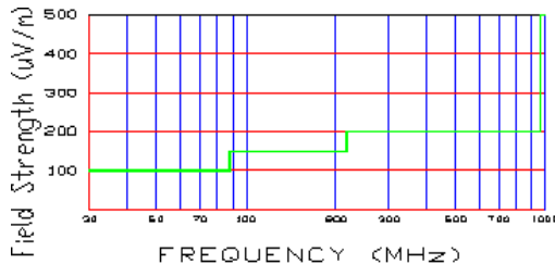
Figure A-16. Radiated limits at 3 meters.
