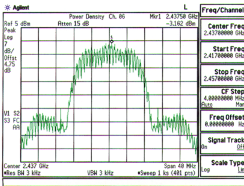
Plot A-8. FCC ID: ACJ9TGCF-T21 Max. Power Density Plot – Ch. 06
