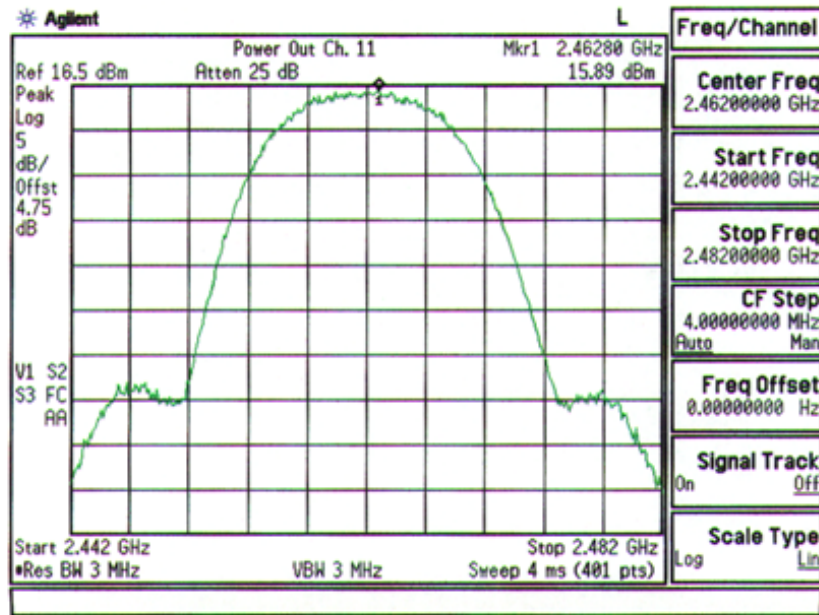
Plot A-6. FCC ID: ACJ9TGCF-T21 Max. Peak Output Power Plot – Ch. 11
