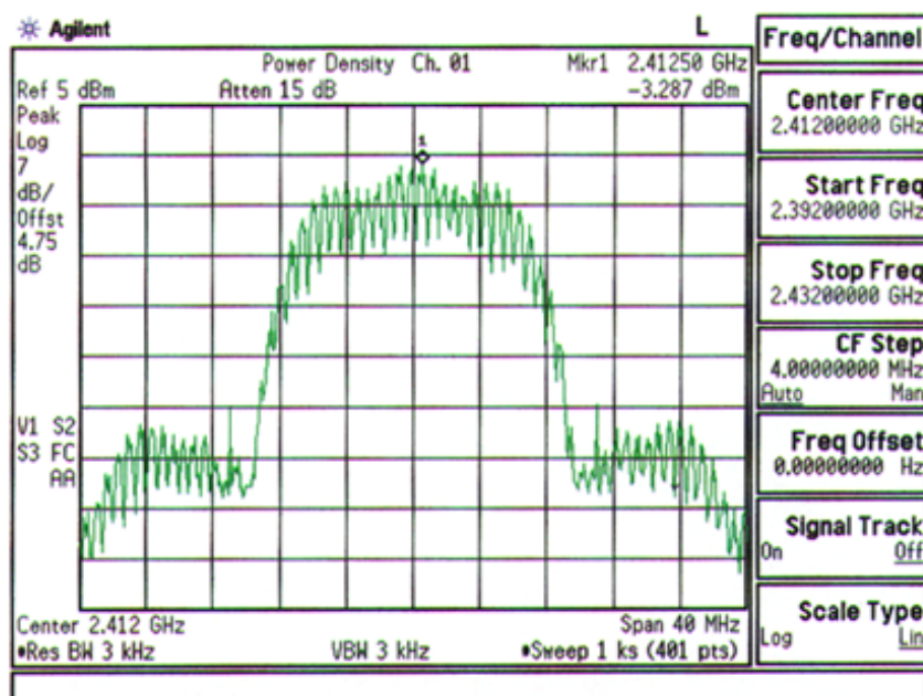
Plot A-7. FCC ID: ACJ9TGCF-T21 Max. Power Density Plot – Ch. 01
