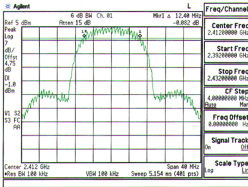
Plot A-1. FCC ID: ACJ9TGCF-T216dB Bandwidth Plot – Ch. 01
