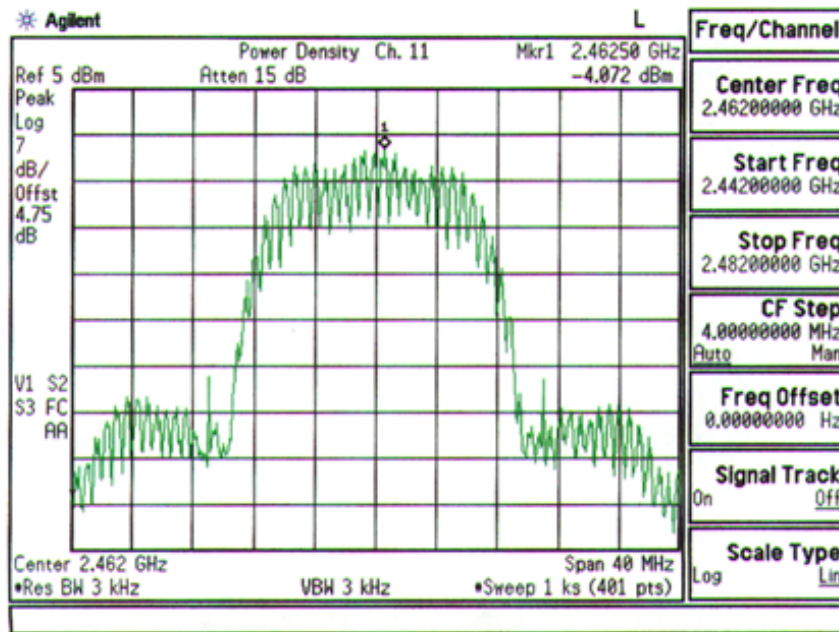
Plot A-9. FCC ID: ACJ9TGCF-T21 Max. Power Density Plot – Ch. 11
