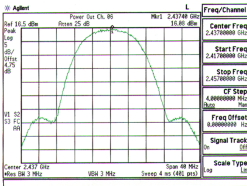
Plot A-5. FCC ID: ACJ9TGCF-T21 Max. Peak Output Power Plot – Ch. 06
