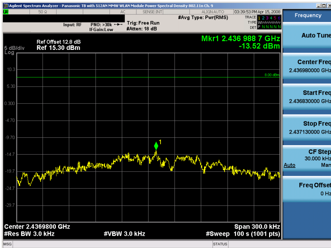
Plot 6-26. Power Spectral Density Plot (802.11n (2.4GHz) – Ch. 9)
