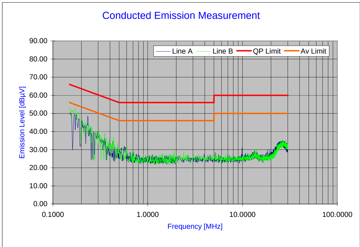
Plot 6-54. Line Conducted Plot with 802.11n
