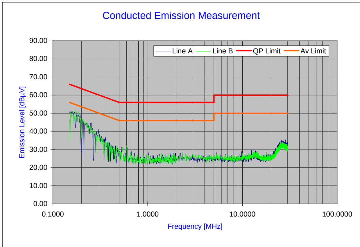
Plot 6-53. Line Conducted Plot with 802.11a
