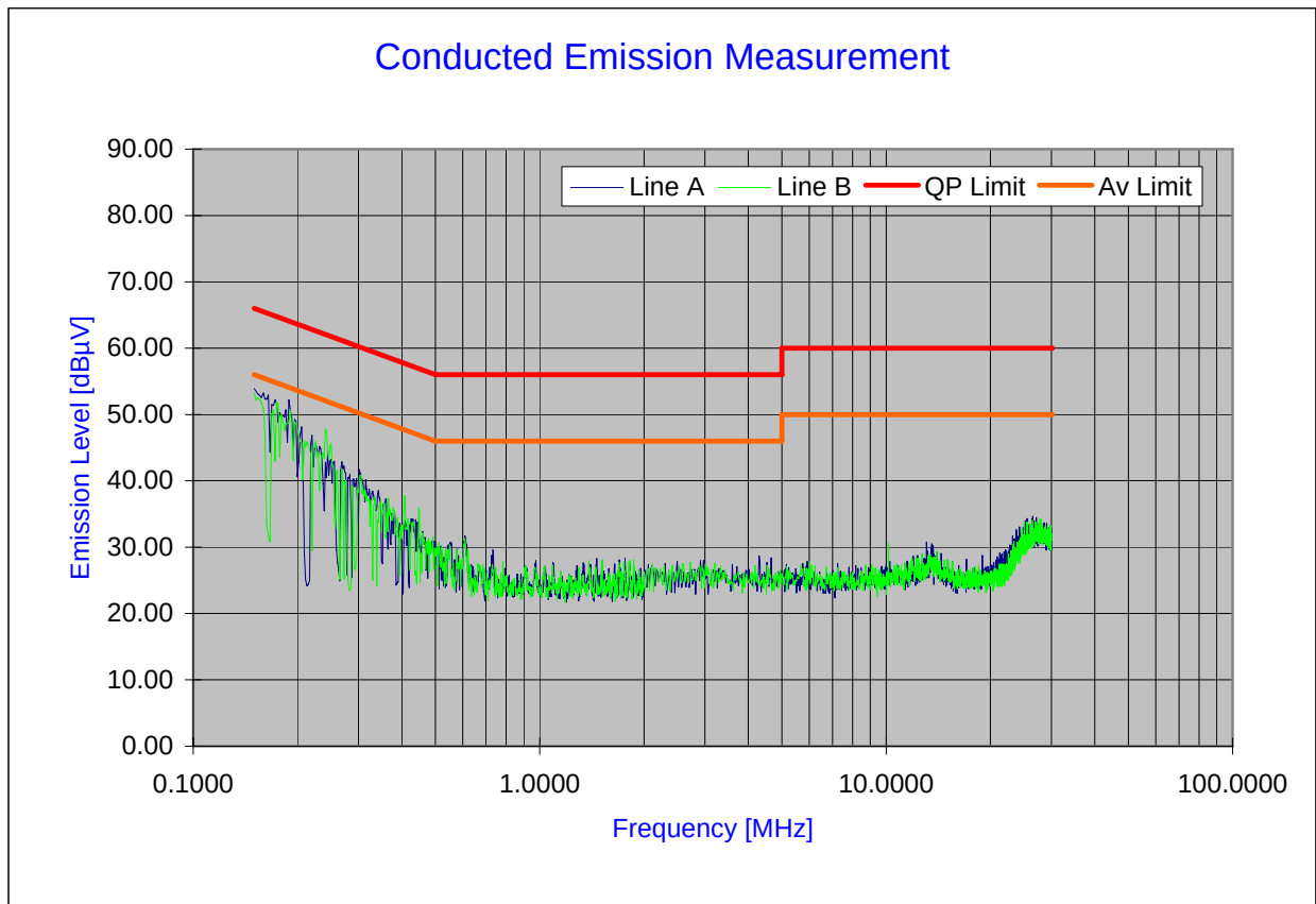
Plot 6-51. Line Conducted Plot with 802.11b
