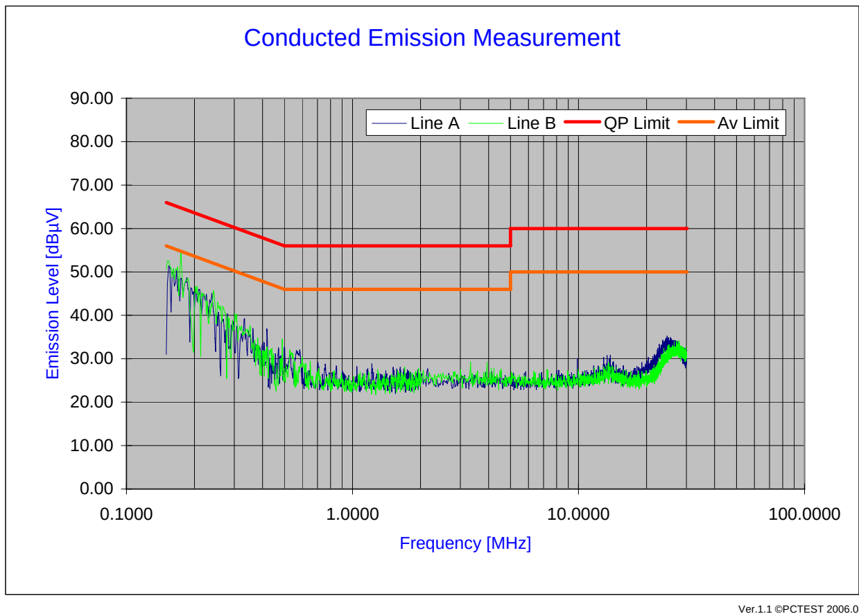
Plot 6-52. Line Conducted Plot with 802.11g
