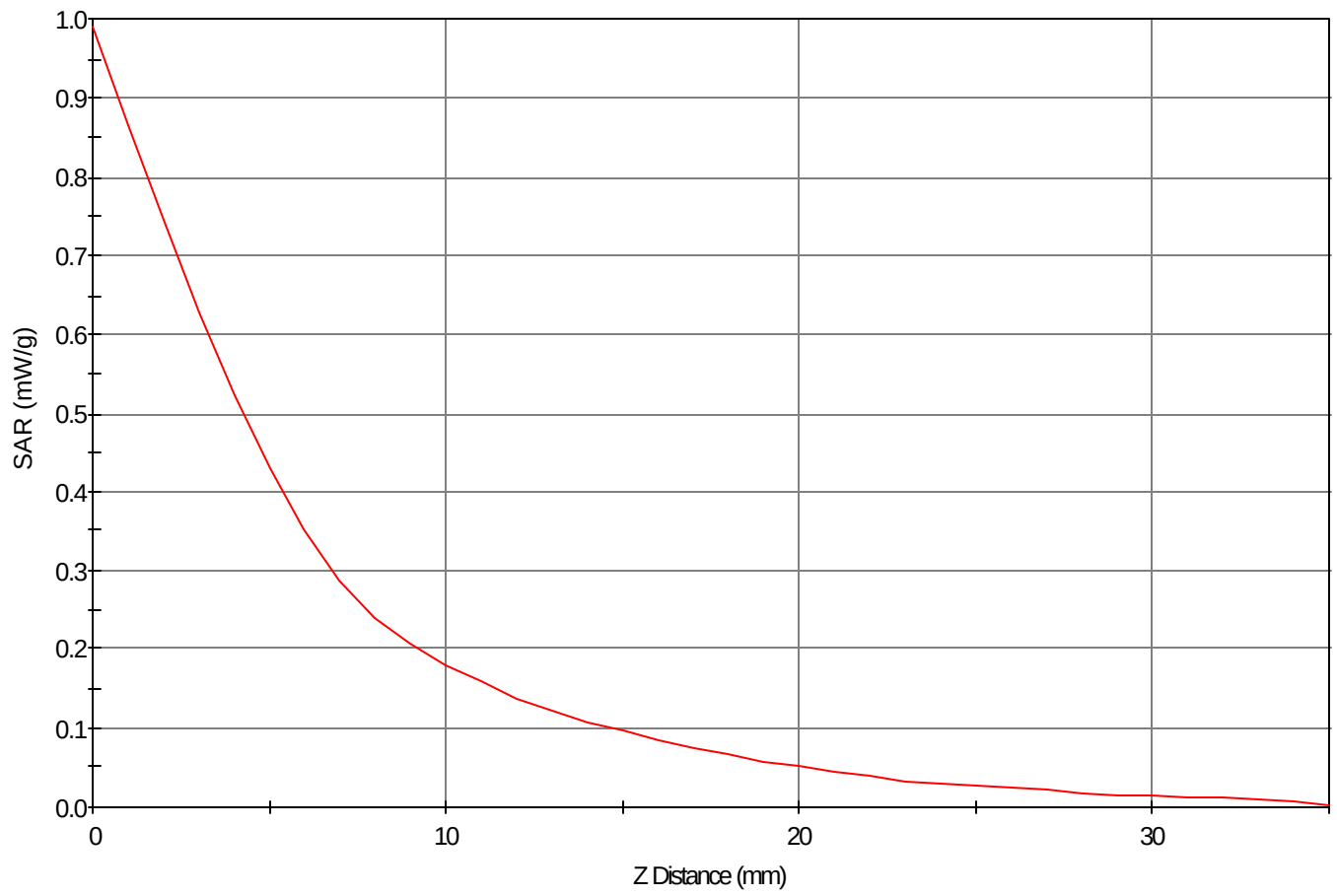
SAR - Z Axis at Hotspot x:26.0 y:44.0
