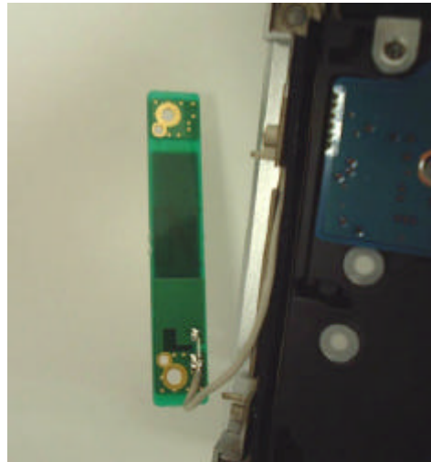
Right Antenna Bottom View
