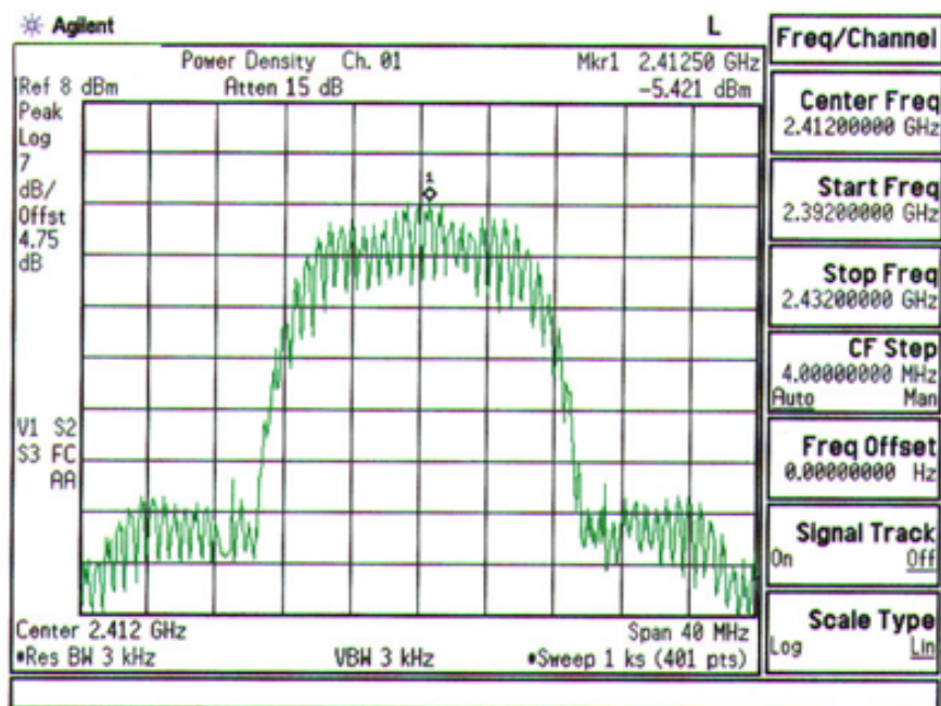
Plot A-7. FCC ID: ACJ9TGCF-W21 Max. Power Density Plot – Ch.1
