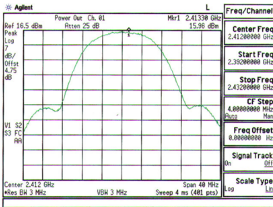
Plot A-4. FCC ID: ACJ9TGCF-W21 Max. Peak Output Power Plot – Ch.1
