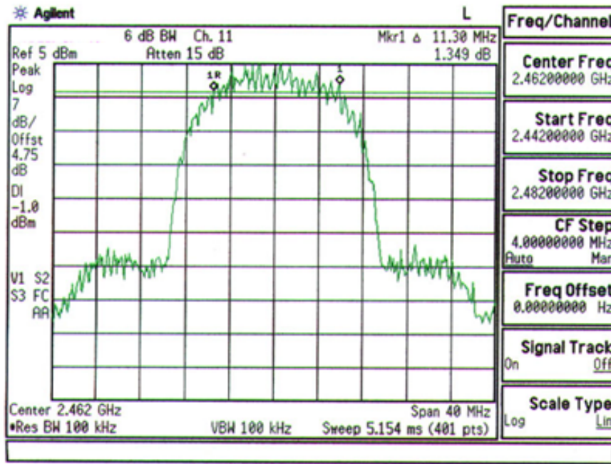
Plot A-3. FCC ID: ACJ9TGCF-W21 6dB Bandwidth Plot – Ch.11
