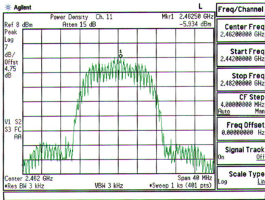
Plot A-9. FCC ID: ACJ9TGCF-W21 Max. Power Density Plot – Ch.11
