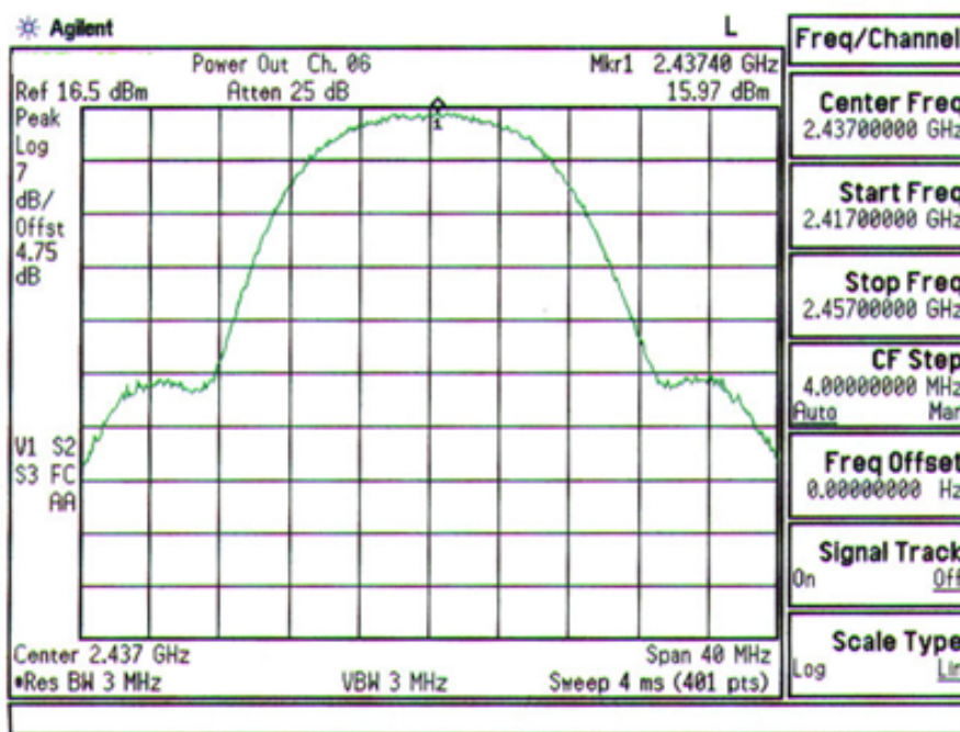
Plot A-5. FCC ID: ACJ9TGCF-W21 Max. Peak Output Power Plot – Ch.6
