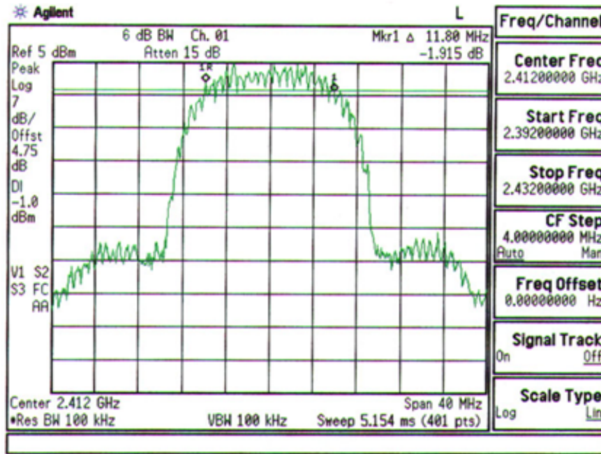
Plot A-1. FCC ID: ACJ9TGCF-W21 6dB Bandwidth Plot – Ch.1
