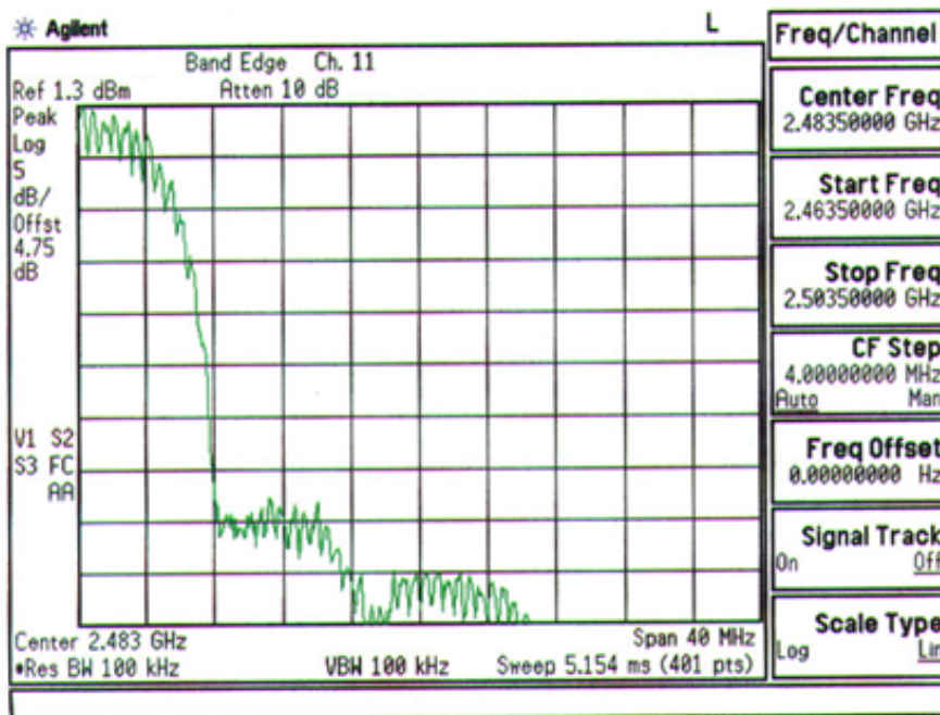
Plot A-12. FCC ID: ACJ9TGCF-W21 BandEdge Plot – Ch.11
