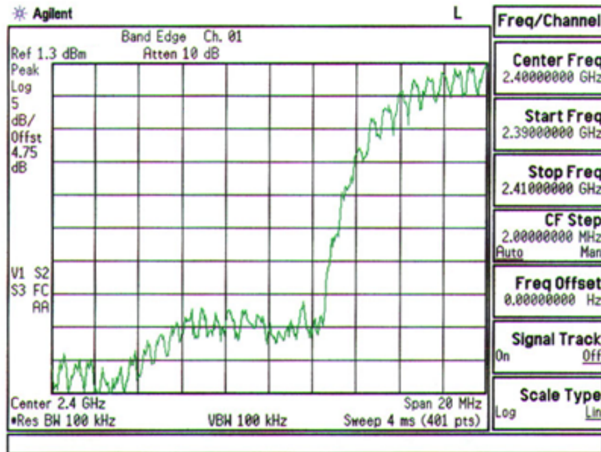
Plot A-10. FCC ID: ACJ9TGCF-W21 BandEdge Plot – Ch.1
