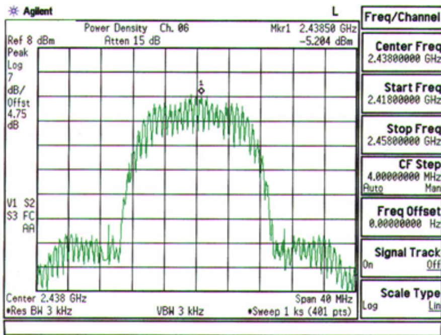
Plot A-8. FCC ID: ACJ9TGCF-W21 Max. Power Density Plot – Ch.6
