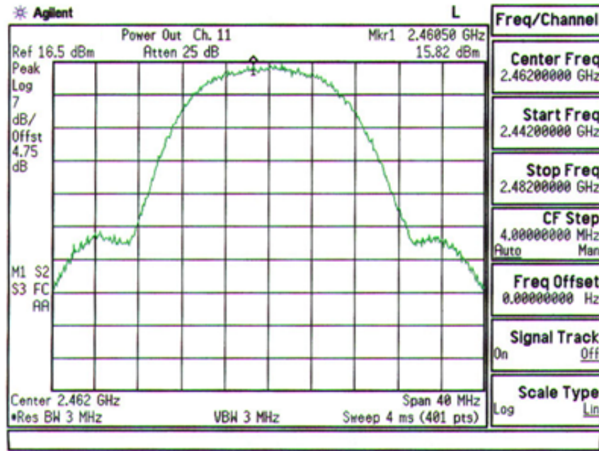
Plot A-6. FCC ID: ACJ9TGCF-W21 Max. Peak Output Power Plot – Ch.11
