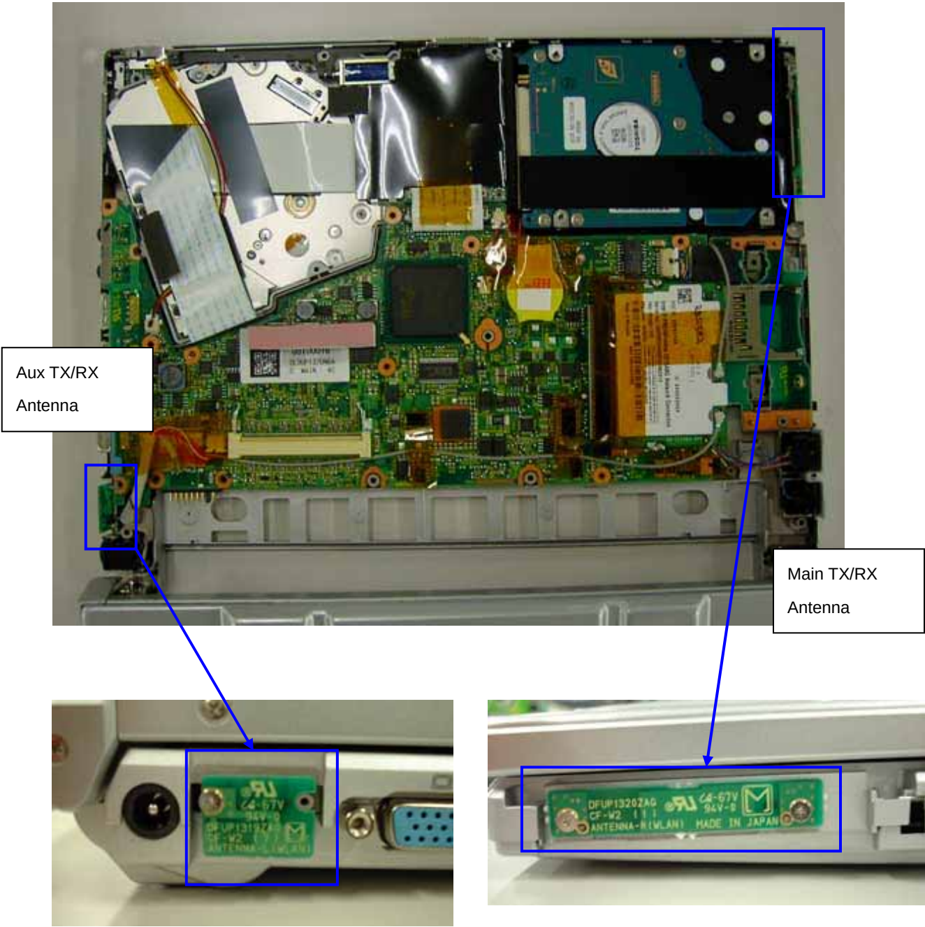
Aux TX/RX Antenna Magnified View
