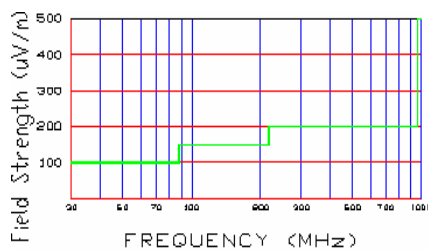
Figure A-10. Radiated limits at 3 meters.
