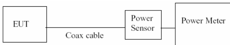
Figure A-4. Test Instrument & Measurement Setup
