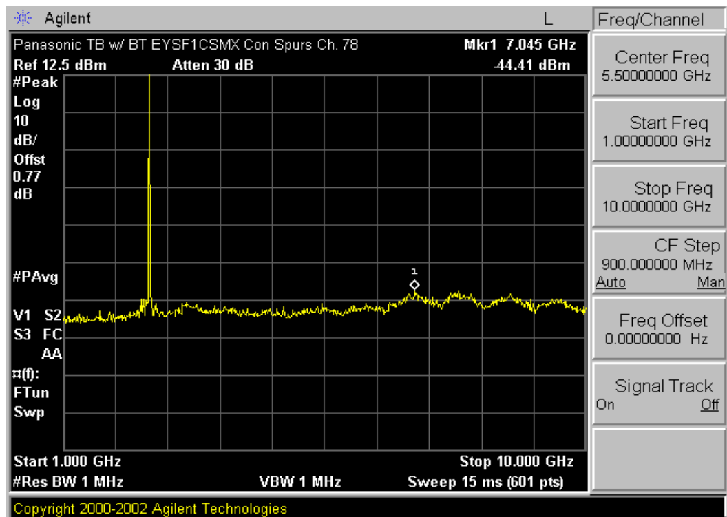
Plot 6-14. Conducted Spurious Plot (Bluetooth – Ch. 78)
