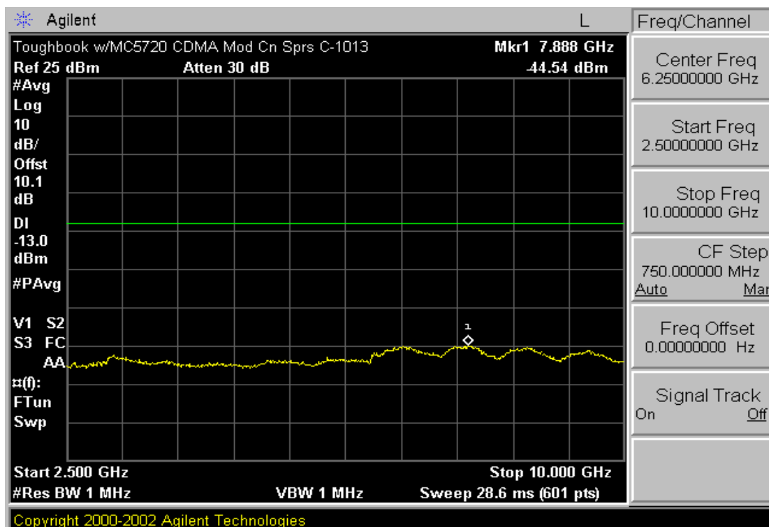
Plot A-2. Conducted Spurious Plot (Cellular CDMA EvDO Mode – Ch. 1013)
