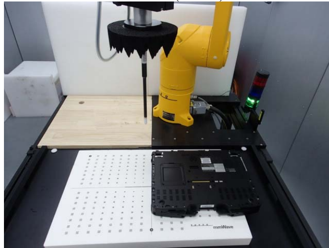
Module #1 (Bottom)
