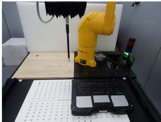
Module #2 (Keyboard)
