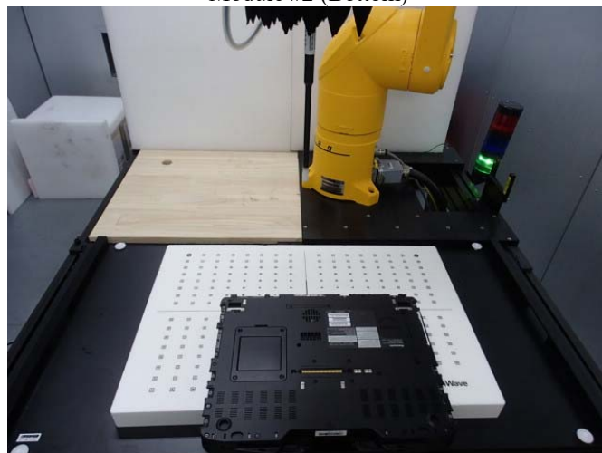
Module #2 (Bottom)
