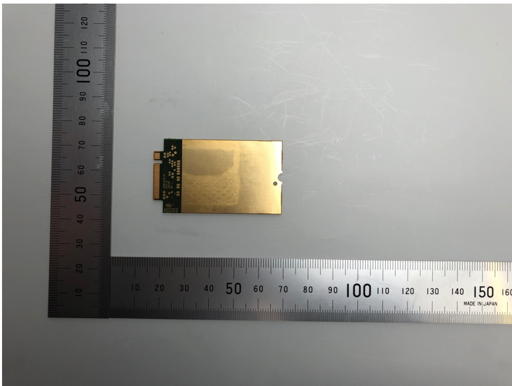
3G/4G/5G Sub6 WWAN module - Back
