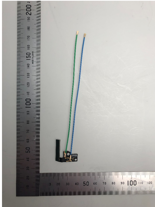
mmWave #2 Antenna - Back
