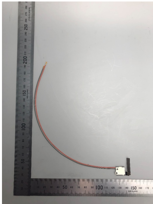
mmWave #1 Antenna - Back
