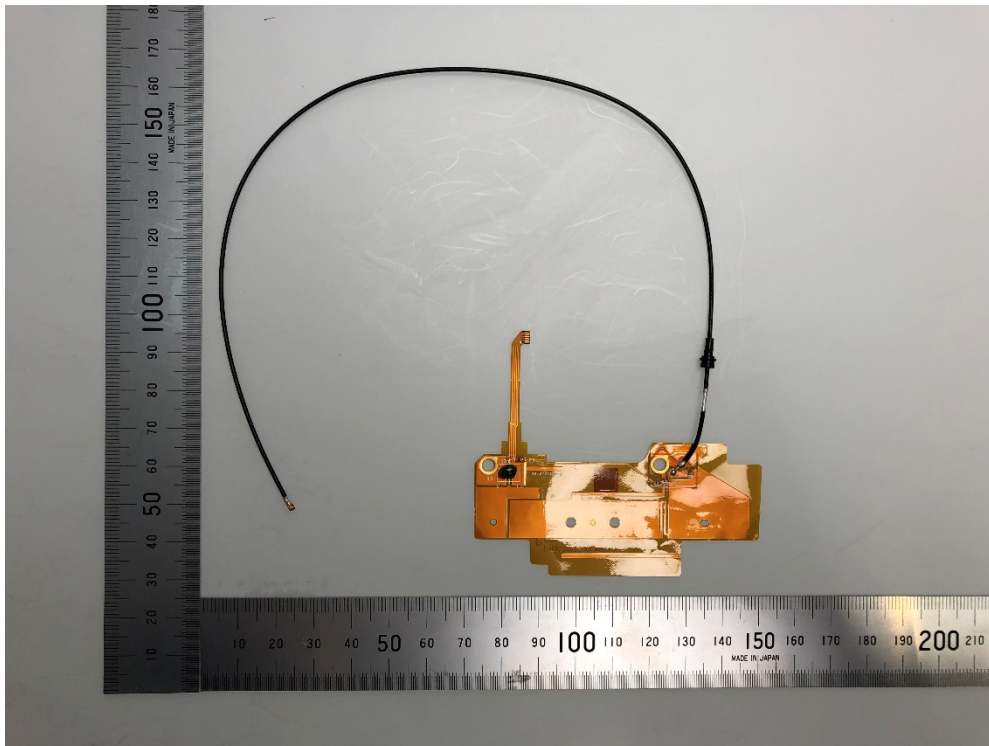
WWAN #1 TX/RX Antenna - Back
