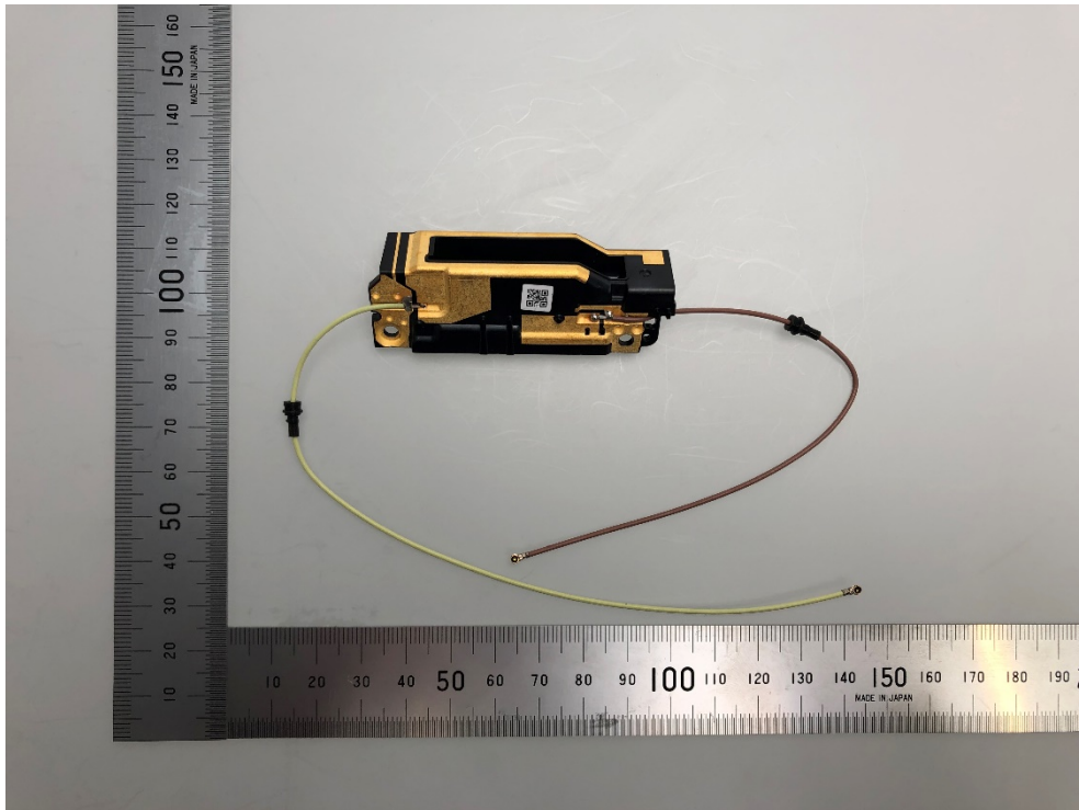
WLAN #2 and Bluetooth TX/RX Antenna - Back
