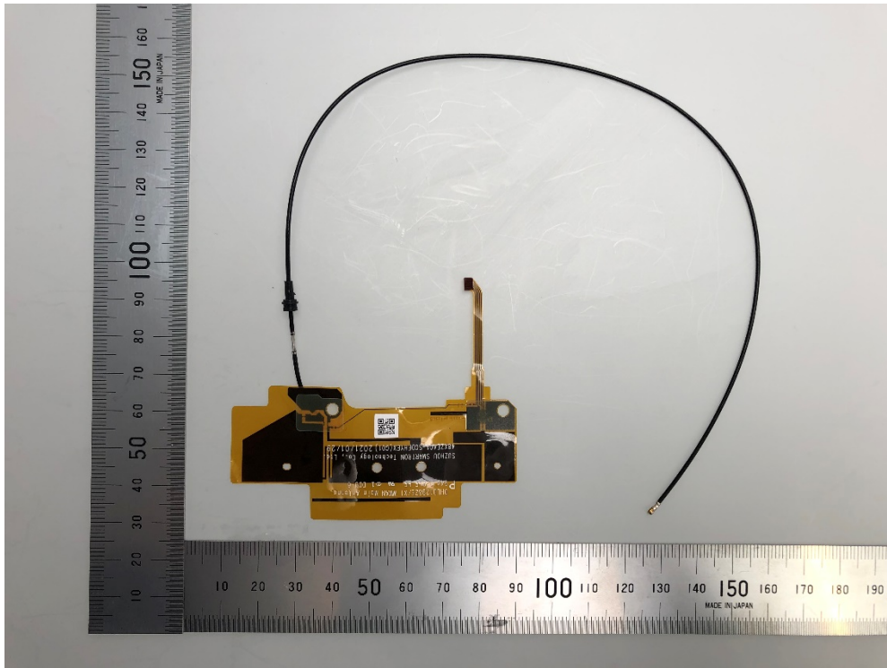
WWAN #1 TX/RX Antenna - Front
