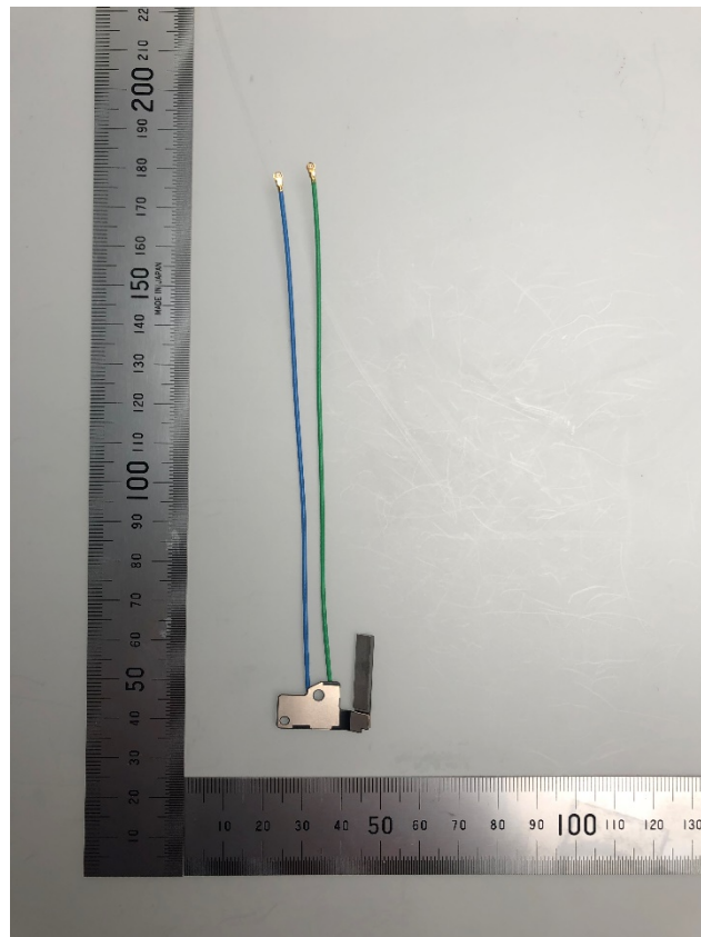
mmWave #2 Antenna - Back
