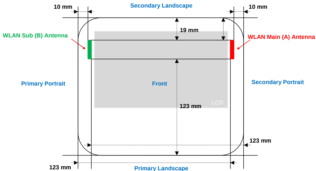
Front View
