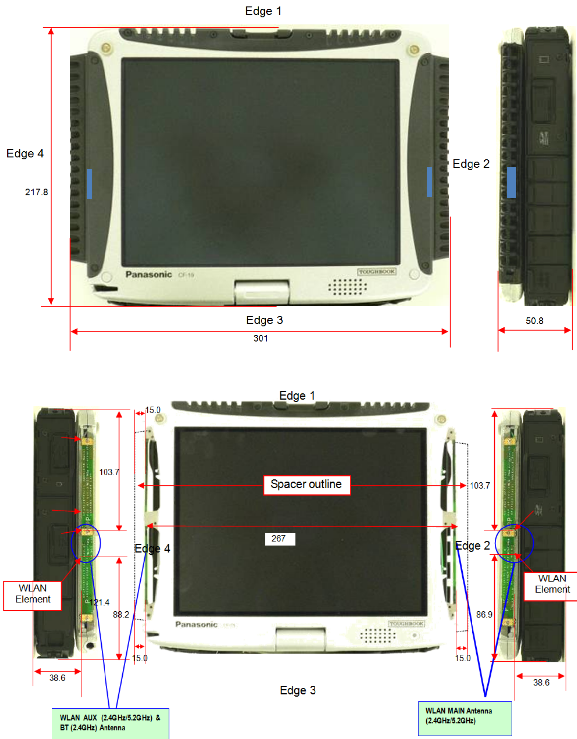
Antenna Locations
