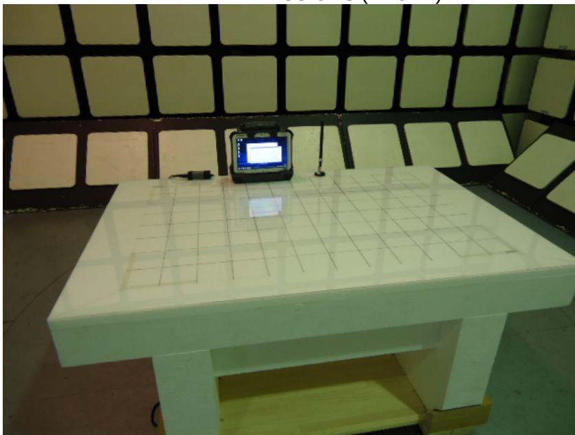
RADIATED EMISSIONS (FRONT)
