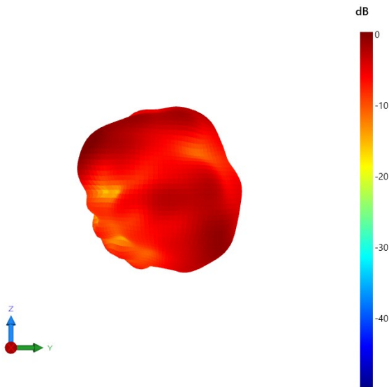
Max Antenna 3D Radiation Pattern 5150-5250 MHz
