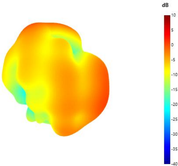
Max Antenna 3D Radiation Pattern 5150-5250 MHz
