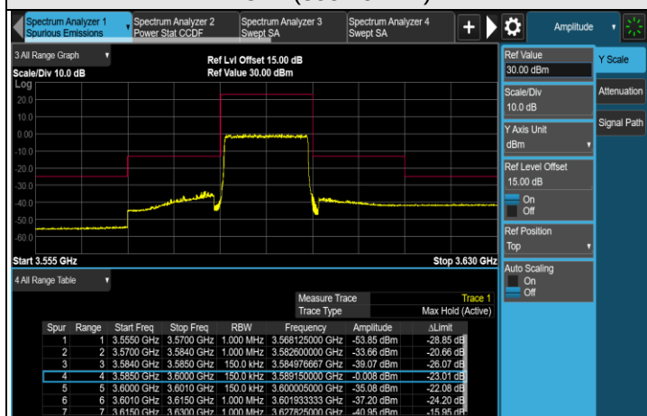
FULL (3592.5MHz)
