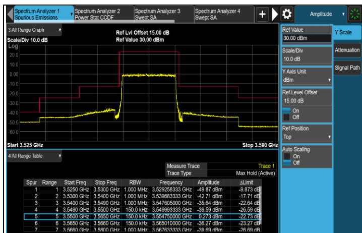
FULL (3557.5MHz)
