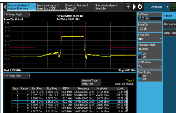
FULL (3575MHz)
