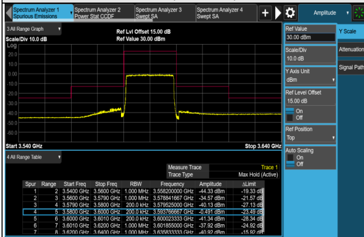
FULL (3590MHz)
