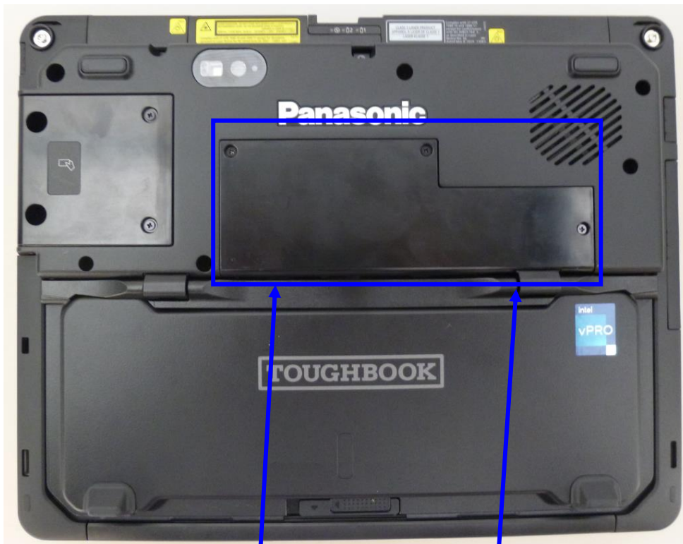
Fig. 2-4. Antenna Location
