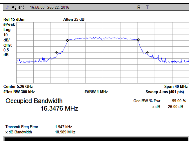
5250-5350MHz Bandwidth - Low CH 5260
