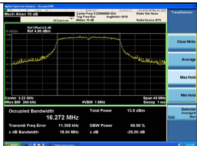
5150-5250MHz Bandwidth - Middle CH 5220
