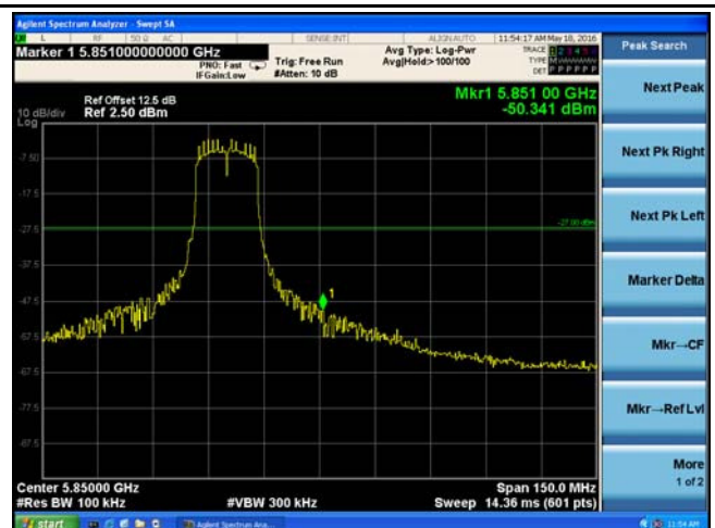
5725-5850MHz Band Edge - High CH 5825
