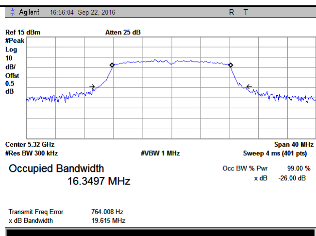
5250-5350MHz Bandwidth - High CH 5320
