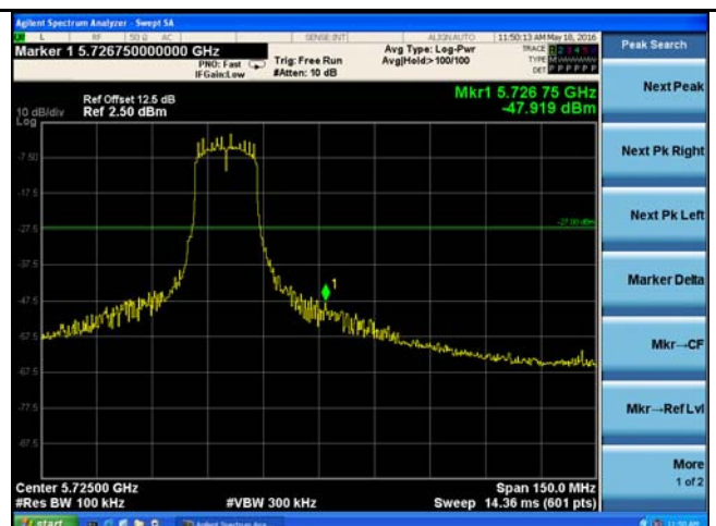
5470-5725MHz Band Edge - High CH 5700
