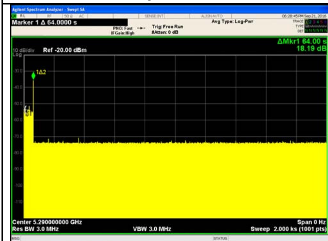
Non-occupancy period –ac80 – 5290MHz
