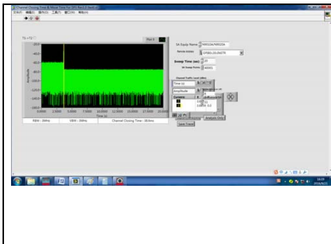
Channel Closing Time – ac80 – 5290MHz
