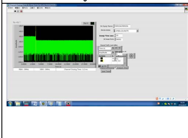
Channel Closing Time –ac80 – 5530MHz
