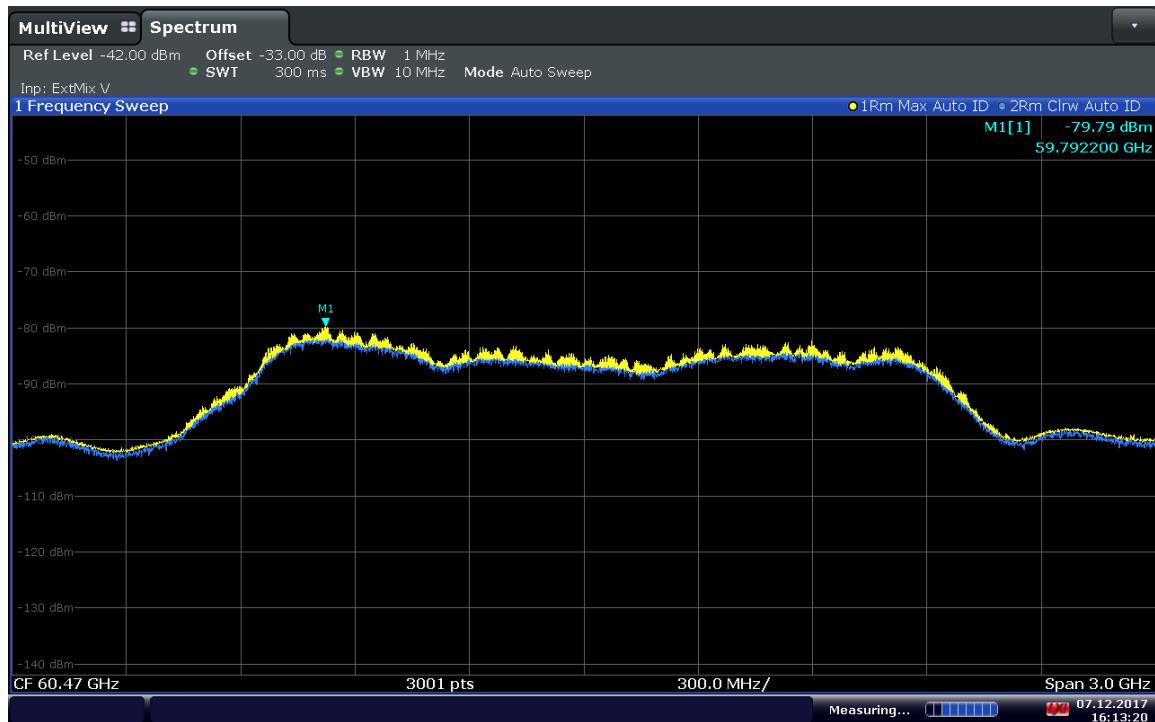
MCS6 Average
