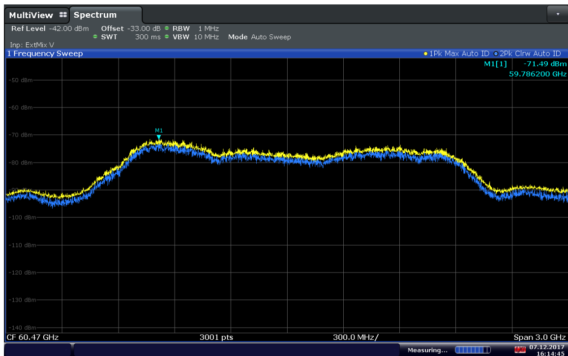
MCS6 Peak
