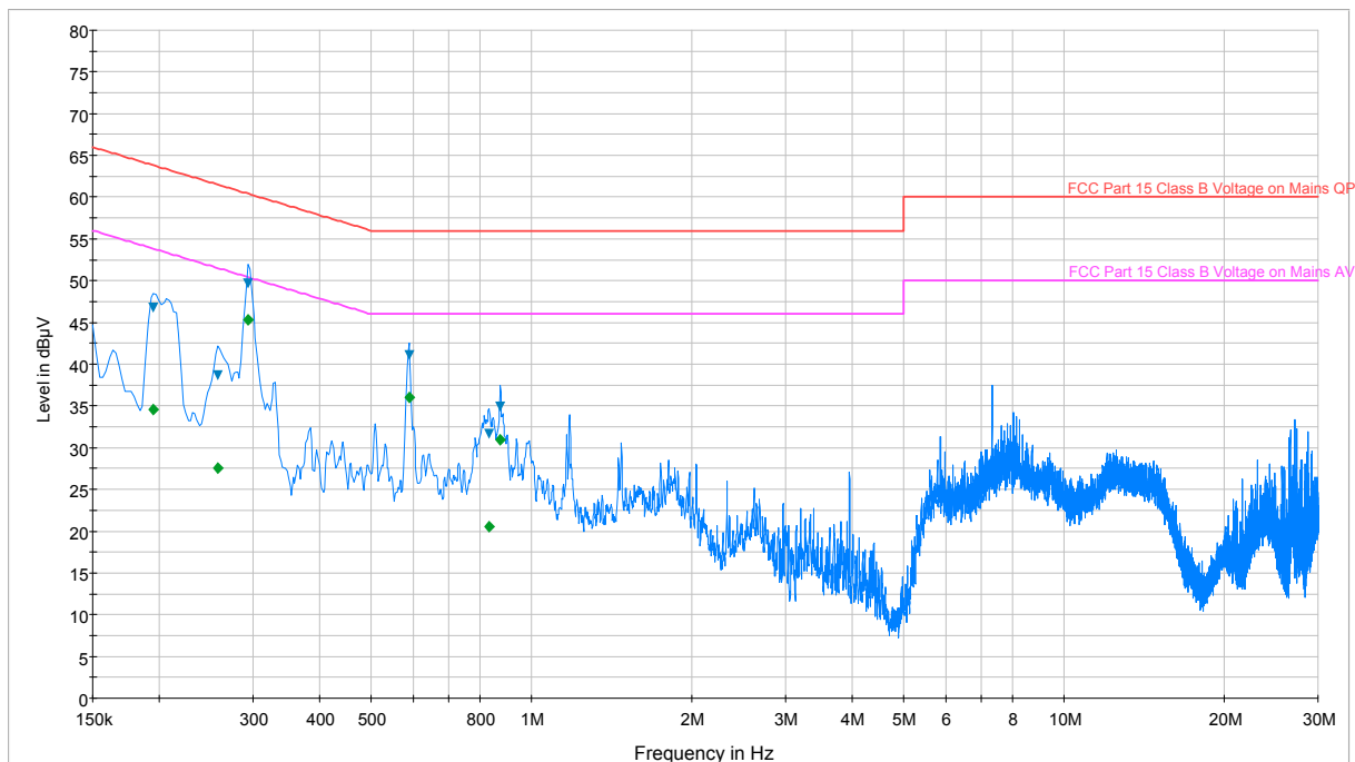
Plot 6-19. Line Conducted Plot with Bluetooth LE (N)
