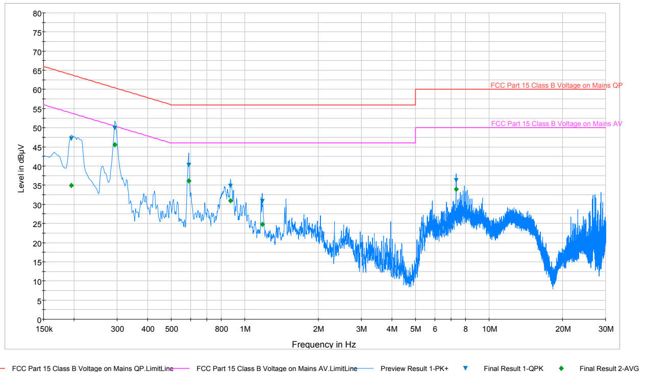
Plot 6-18. Line Conducted Plot with Bluetooth LE (L1)
