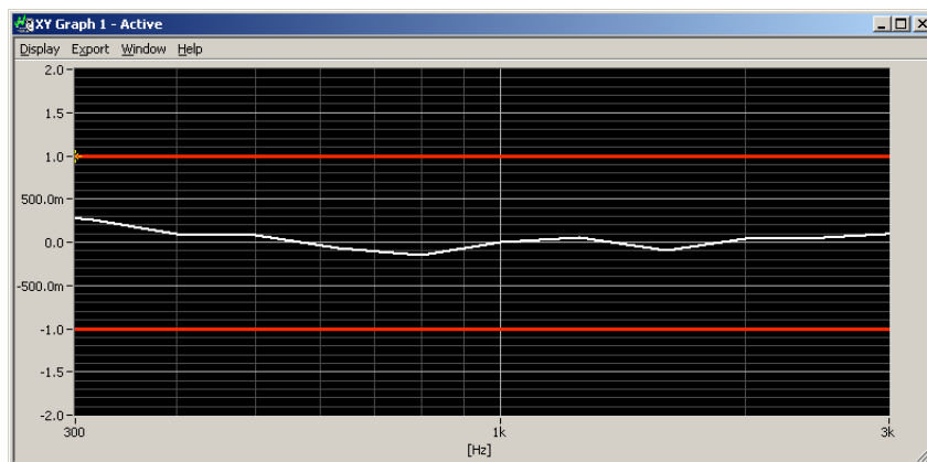
Figure 6-5 Helmholtz Coil Validation for Frequency Response
