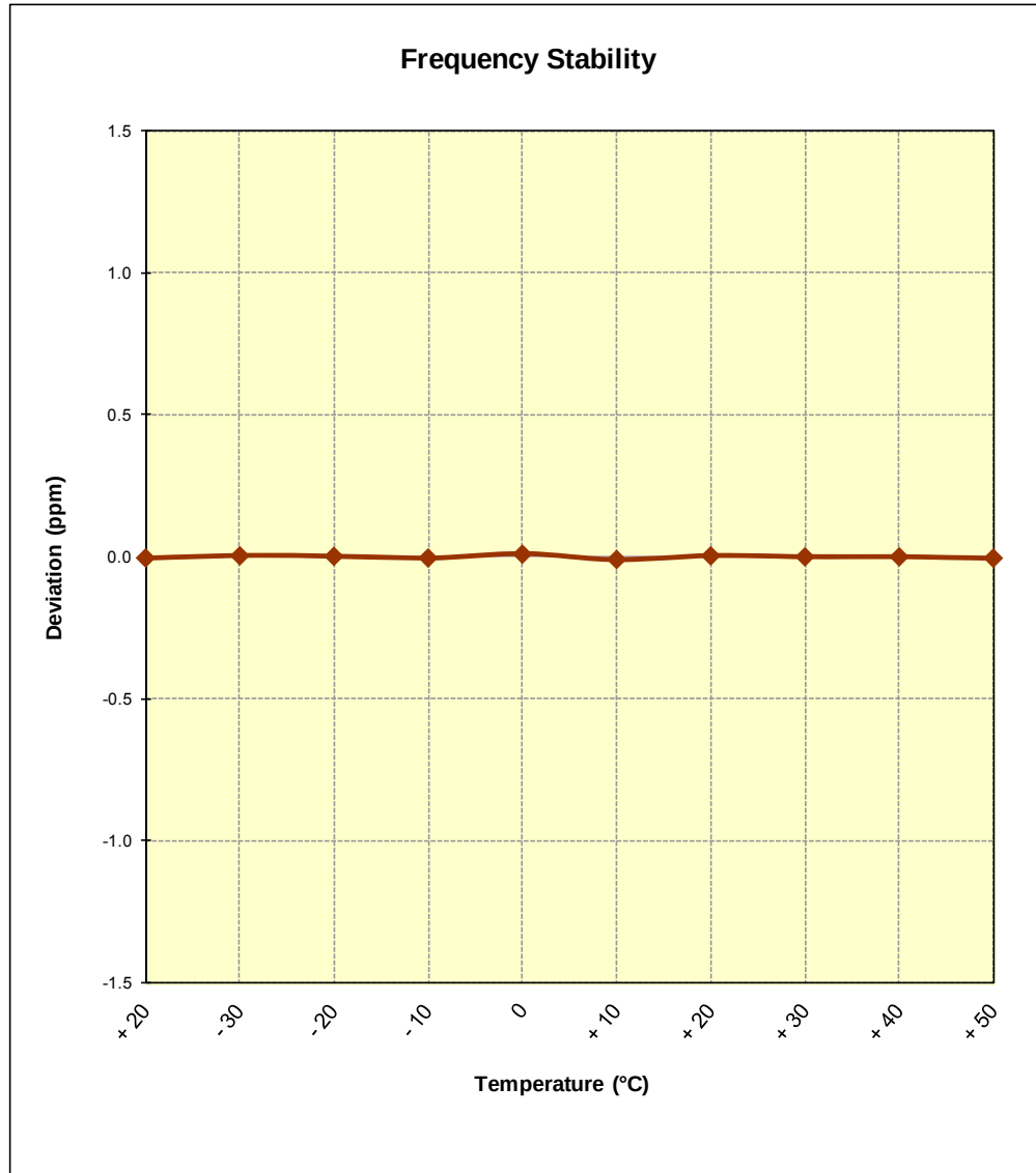
Figure 6-12. Frequency Stability Graph (PCS WCDMA Mode – Ch. 9400)
