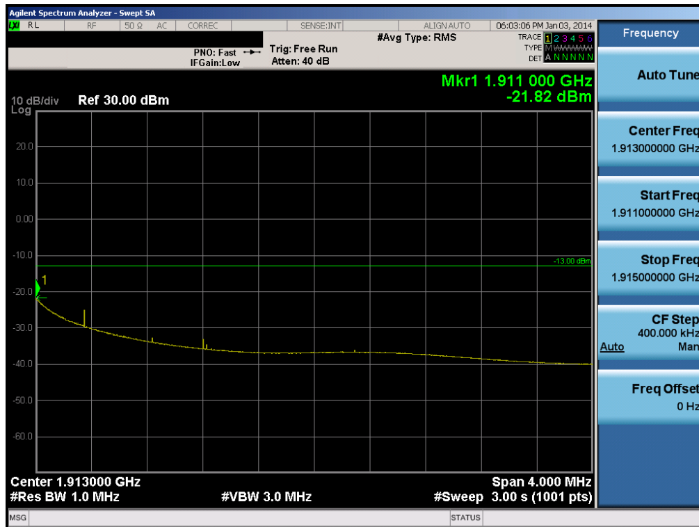
Plot 6-59. 4MHz Span Plot (PCS CDMA Mode – Ch. 1175)
