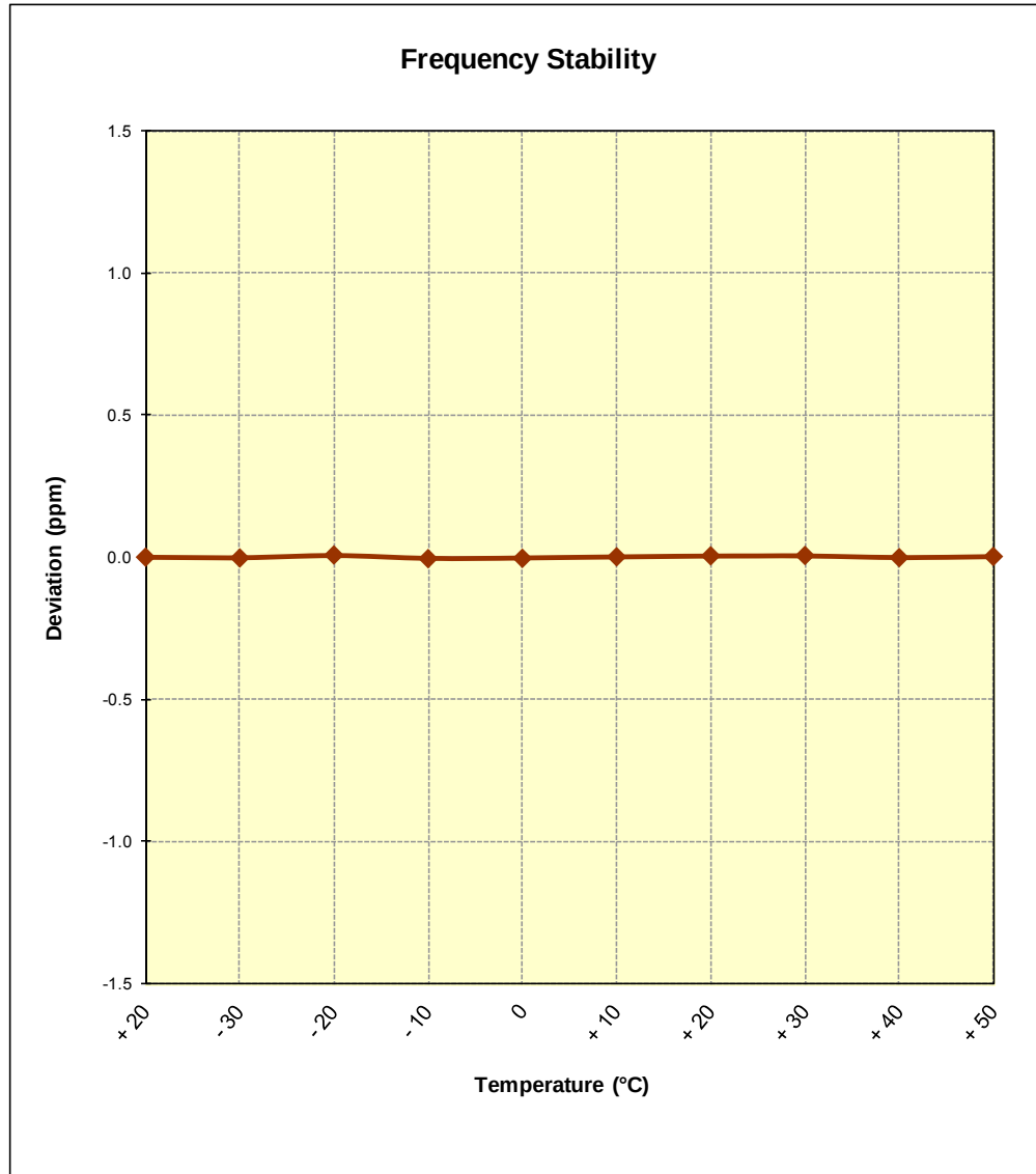
Figure 6-10. Frequency Stability Graph (PCS GSM Mode – Ch. 661)
