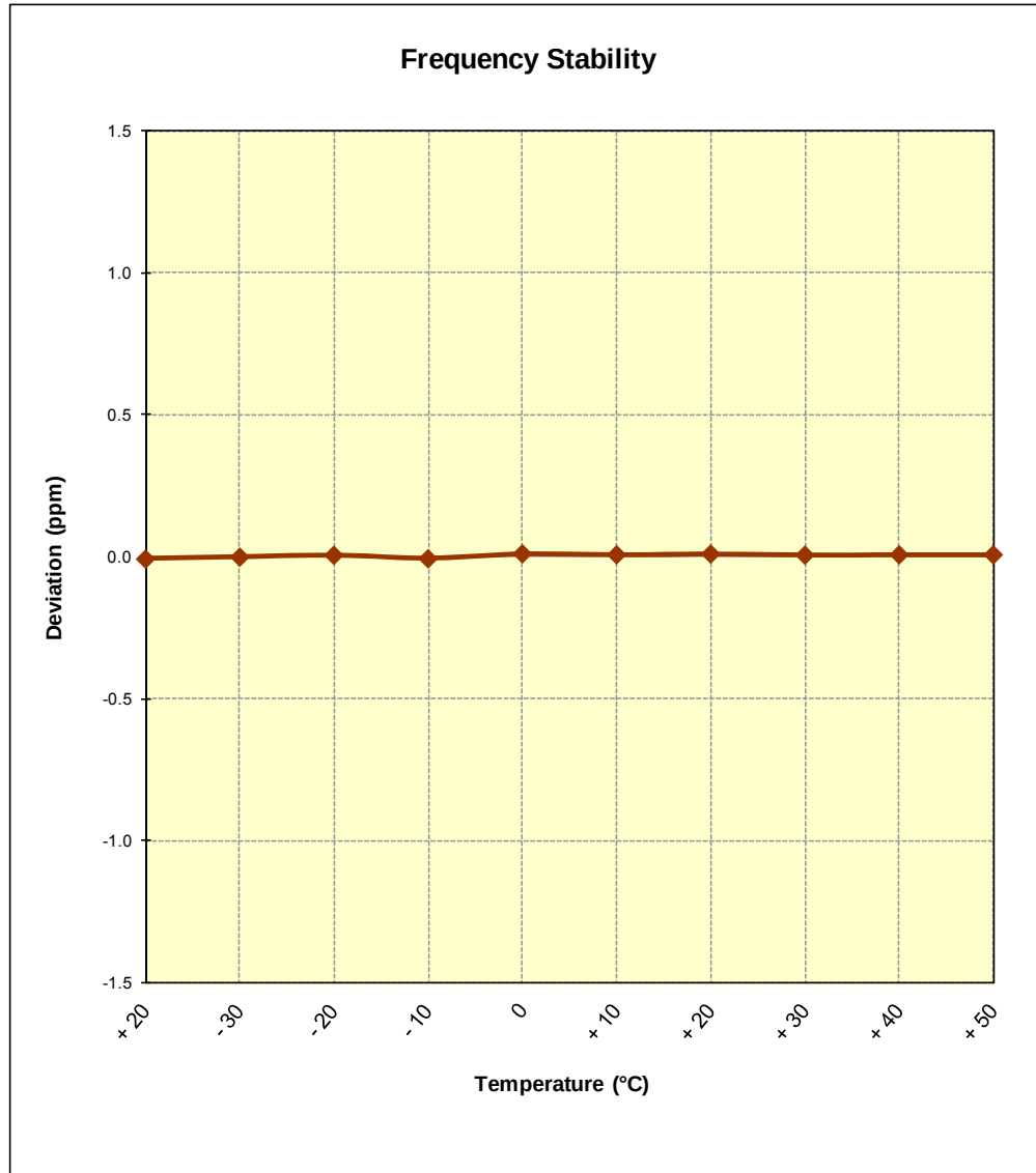
Figure 6-11. Frequency Stability Graph (PCS CDMA Mode – Ch. 600)
