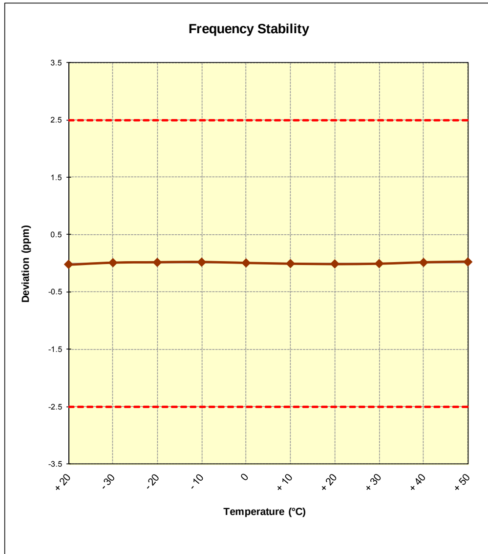
Figure 6-8. Frequency Stability Graph (Cellular CDMA Mode – Ch. 384)
