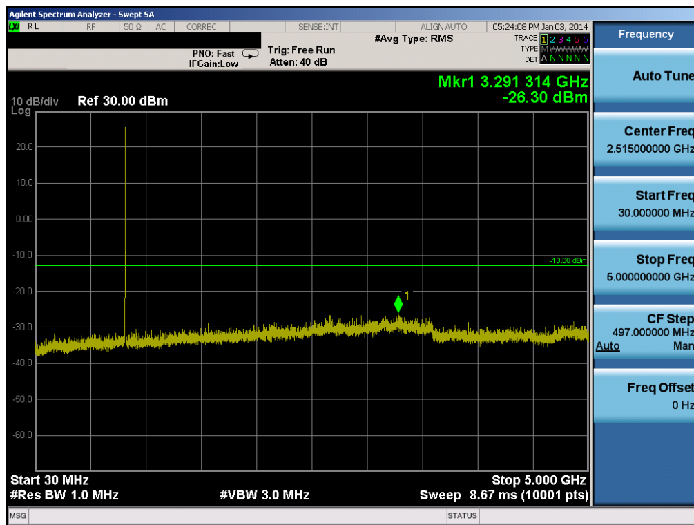
Plot 6-26. Conducted Spurious Plot (Cellular CDMA Mode – Ch. 384)
