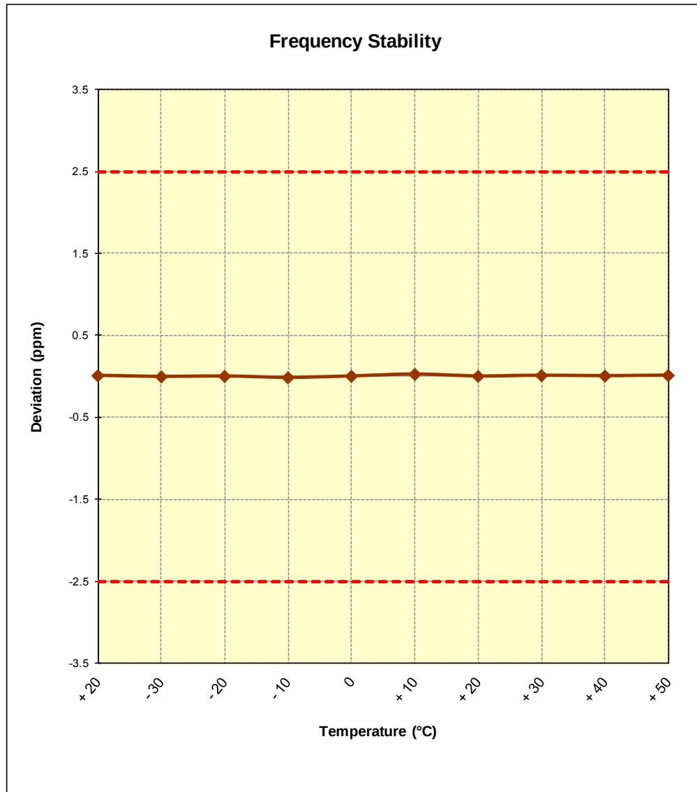
Figure 6-9. Frequency Stability Graph (Cellular WCDMA Mode – Ch. 4183)
