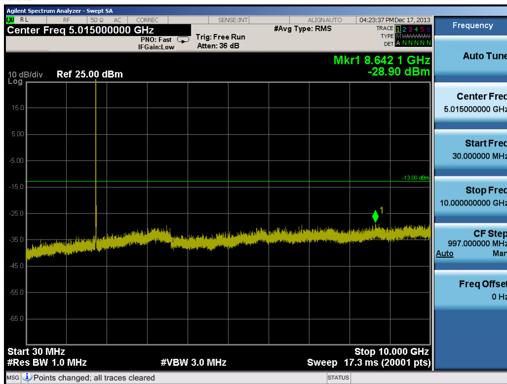
Plot 9-8. Conducted Spurious Plot (5.0MHz QPSK – RB Size 1, RB Offset 0 – High Channel)
