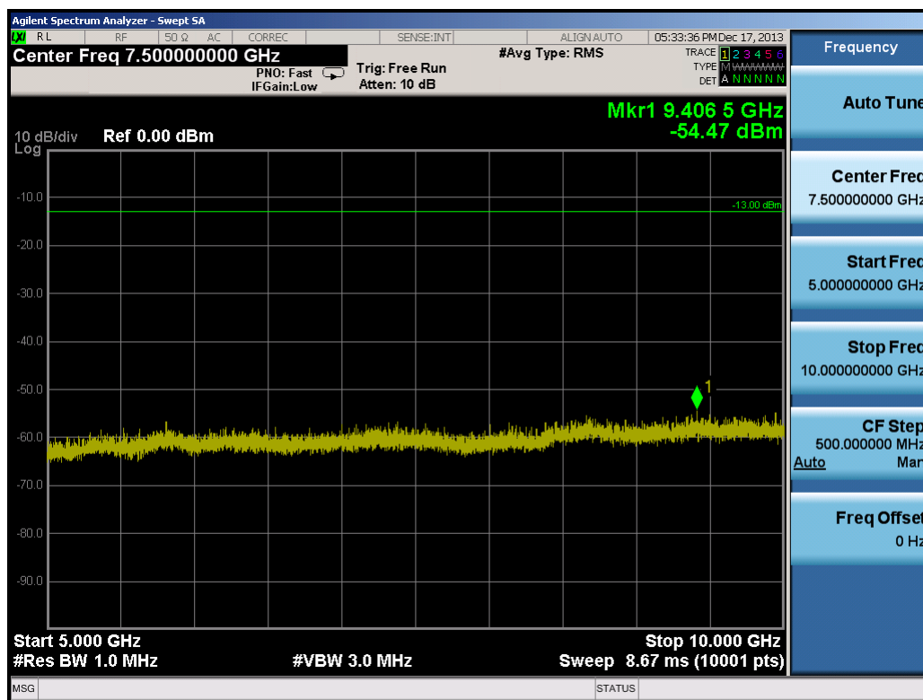
Plot 8-6. Conducted Spurious Plot (10.0MHz QPSK – RB Size 1, RB Offset 0)
