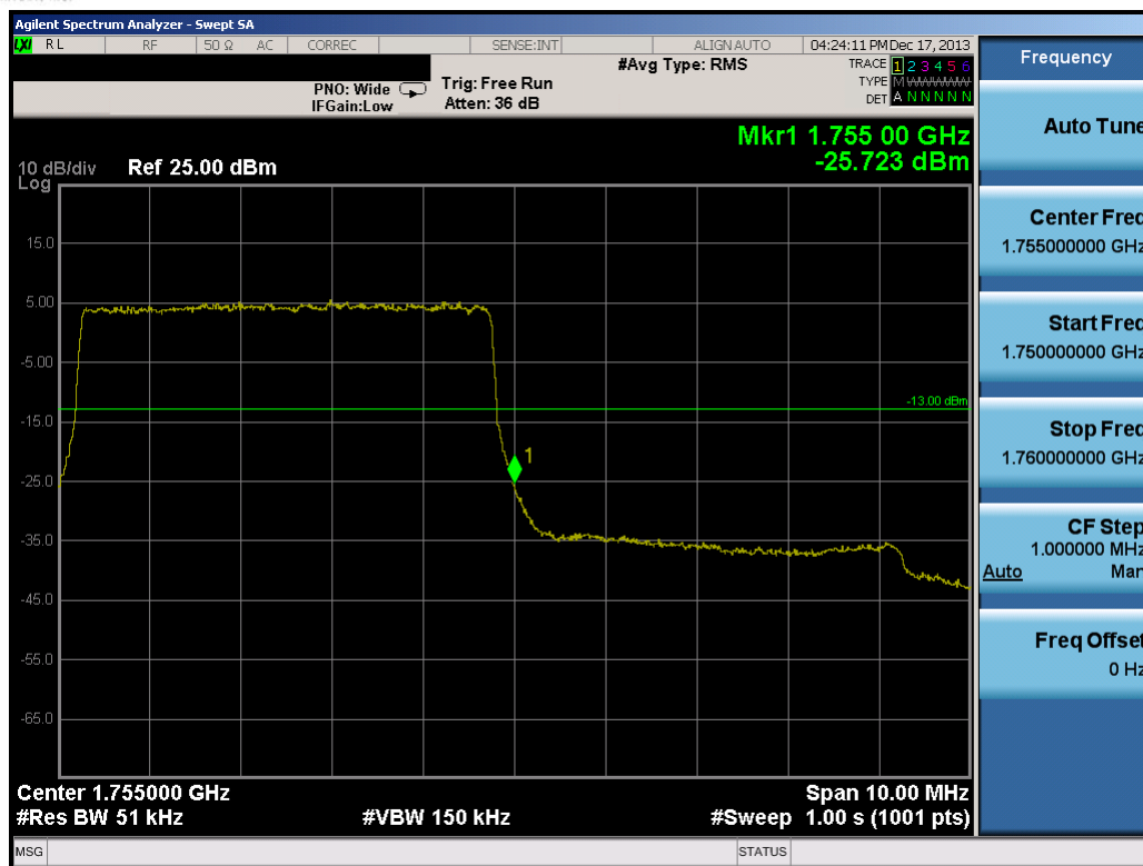
Plot 9-10. Upper Band Edge Plot (5.0MHz QPSK – RB Size 25)
