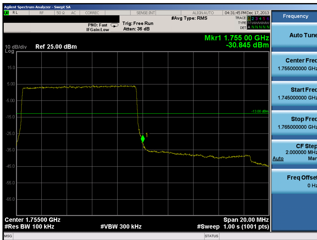
Plot 9-22. Upper Band Edge Plot (10.0MHz QPSK – RB Size 50)
