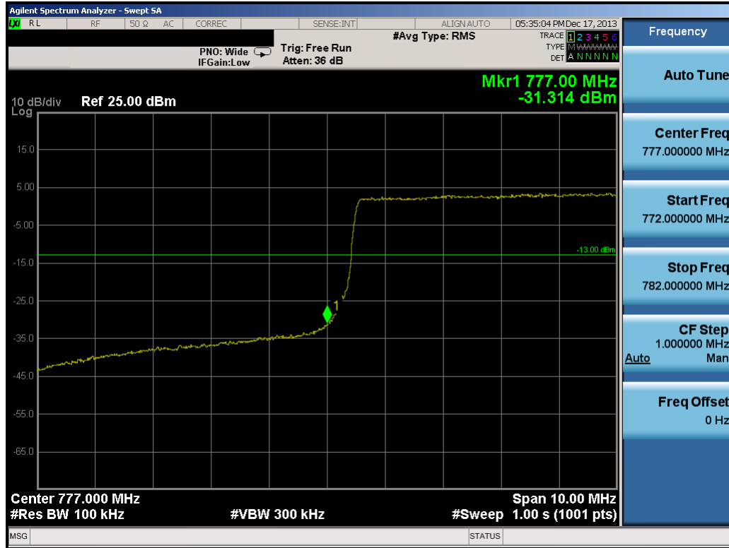
Plot 8-1. Lower Band Edge Plot (10.0MHz QPSK – RB Size 50)
