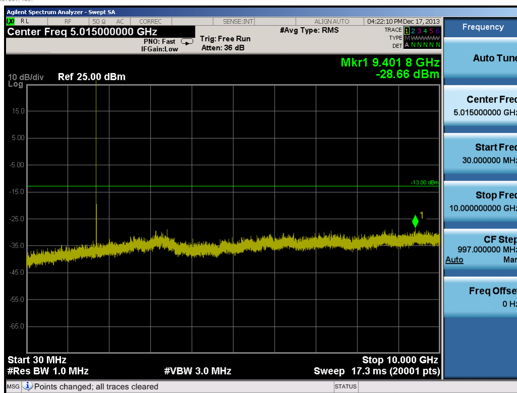
Plot 9-4. Conducted Spurious Plot (5.0MHz QPSK – RB Size 1, RB Offset 0 – Low Channel)
