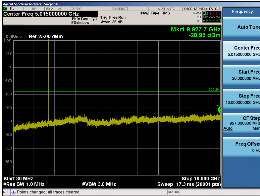
Plot 9-6. Conducted Spurious Plot (5.0MHz QPSK – RB Size 1, RB Offset 0 – Mid Channel)
