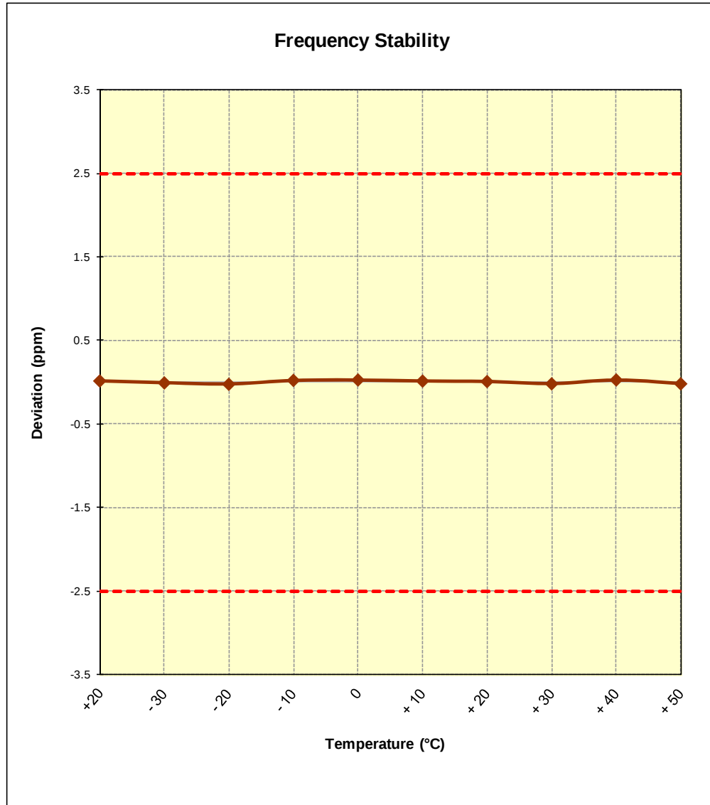
Figure 6-2. Frequency Stability Graph (Band 13)
