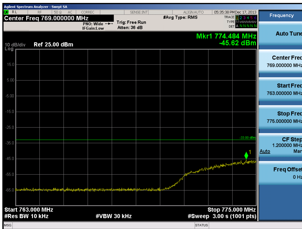
Plot 8-2. Lower Emission Mask Plot (10.0MHz QPSK – RB Size 50)
