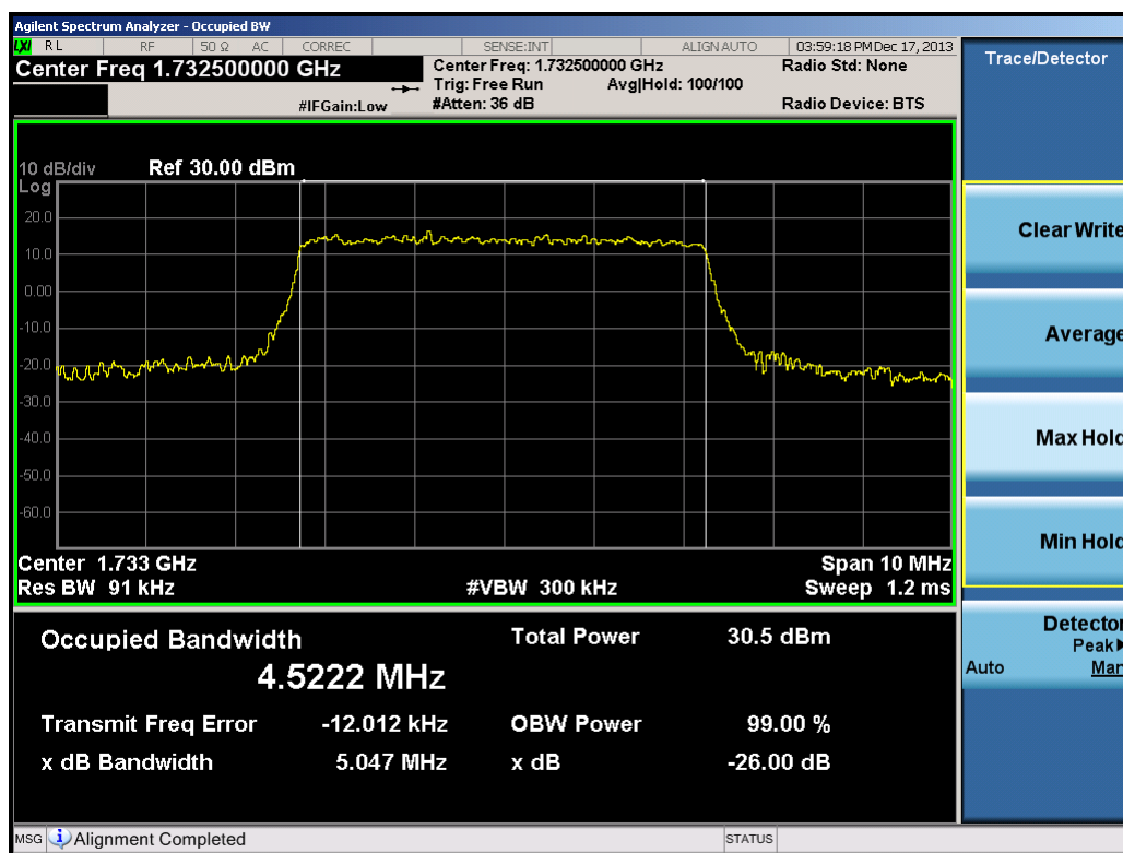
Plot 9-3. Occupied Bandwidth Plot (5.0MHz 16-QAM – RB Size 25)
