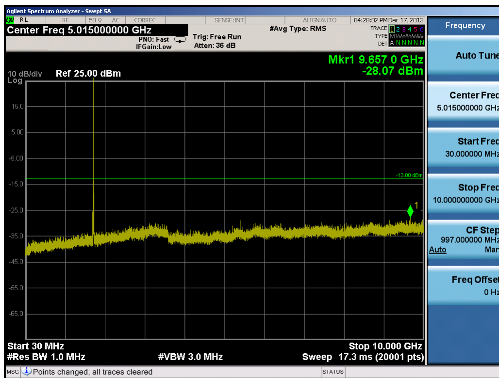
Plot 9-18. Conducted Spurious Plot (10.0MHz QPSK – RB Size 1, RB Offset 0 – Mid Channel)
