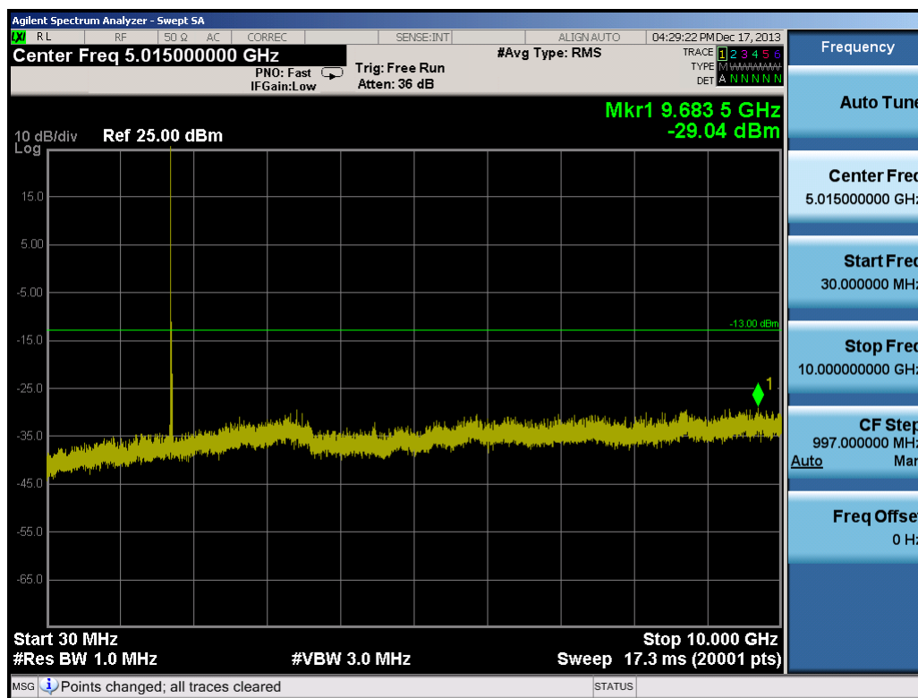
Plot 9-16. Conducted Spurious Plot (10.0MHz QPSK – RB Size 1, RB Offset 0– Low Channel)
