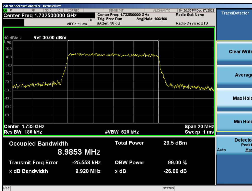
Plot 9-15. Occupied Bandwidth Plot (10.0MHz 16-QAM – RB Size 50)
