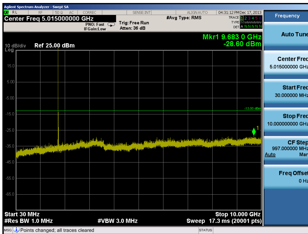
Plot 9-20. Conducted Spurious Plot (10.0MHz QPSK – RB Size 1, RB Offset 0 – High Channel)
