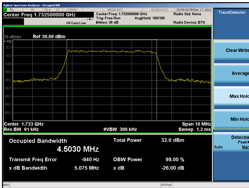
Plot 9-2. Occupied Bandwidth Plot (5.0MHz QPSK – RB Size 25)
