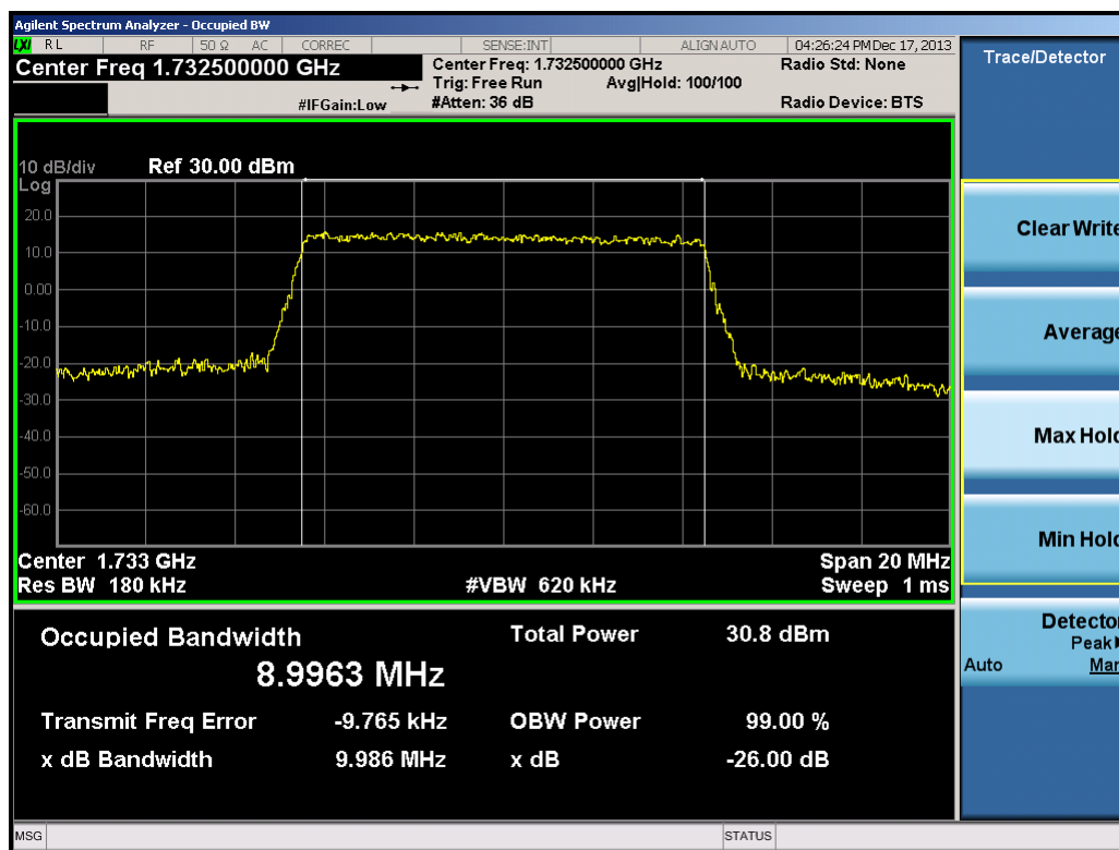
Plot 9-14. Occupied Bandwidth Plot (10.0MHz QPSK – RB Size 50)
