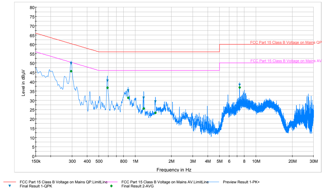
Plot 6-44. Line-Conducted Test Plot (L1)
