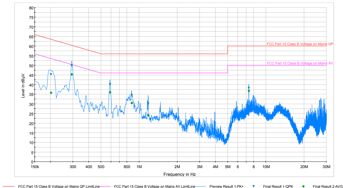
Plot 6-45. Line-Conducted Test Plot (N)
