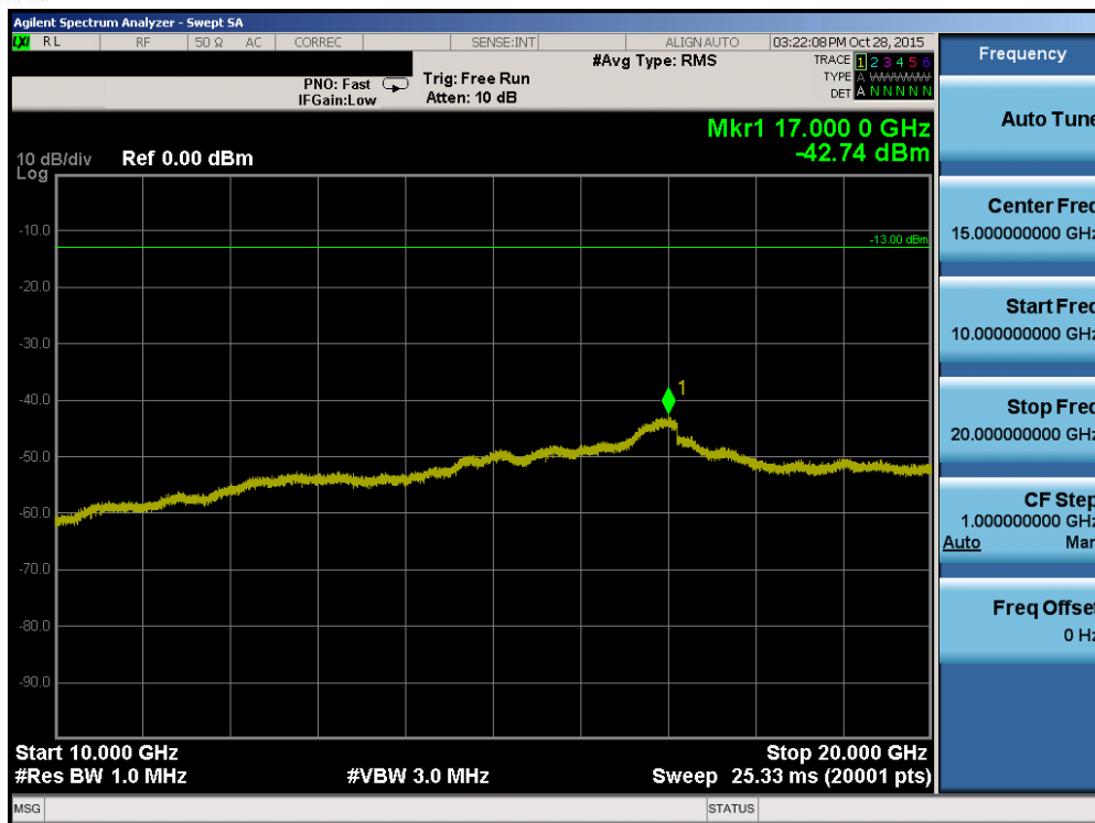
Plot 7-13. Conducted Spurious Plot (Band 4 – 15.0MHz QPSK – RB Size 1, RB Offset 0 – High Channel)
