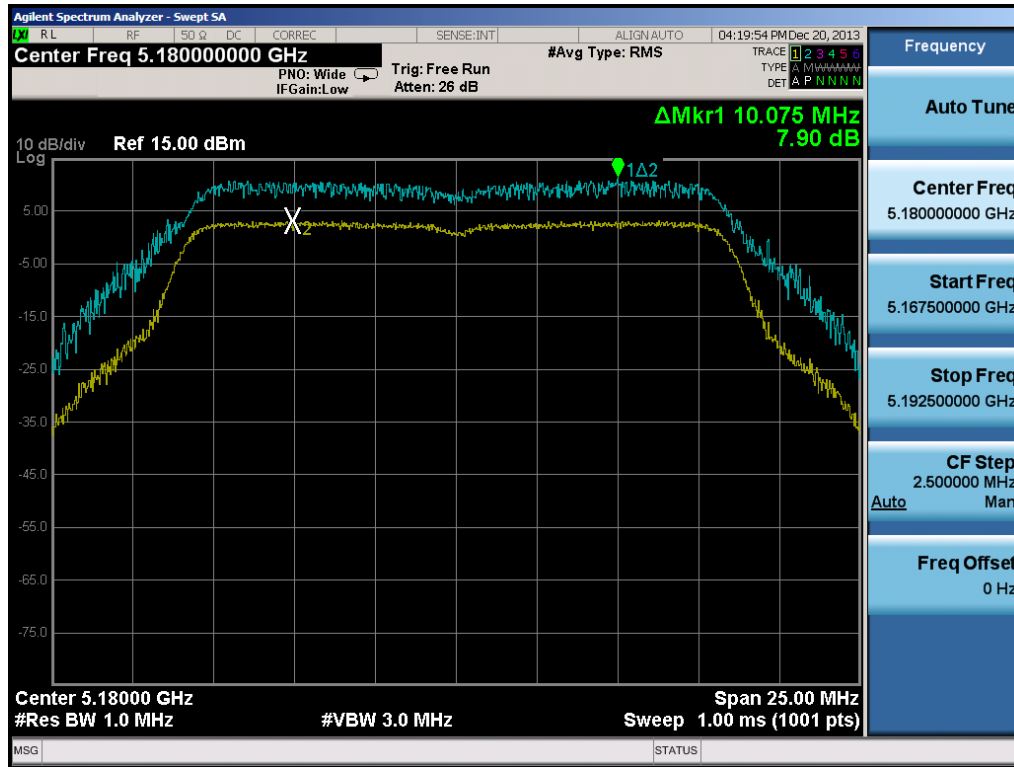
Plot 6-64. Peak Excursion Ratio Plot (802.11a)
