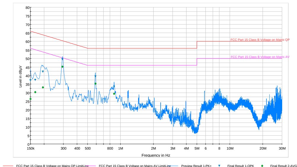
Plot 6-100. Line Conducted Plot with 802.11a UNII Band 2C (N)
