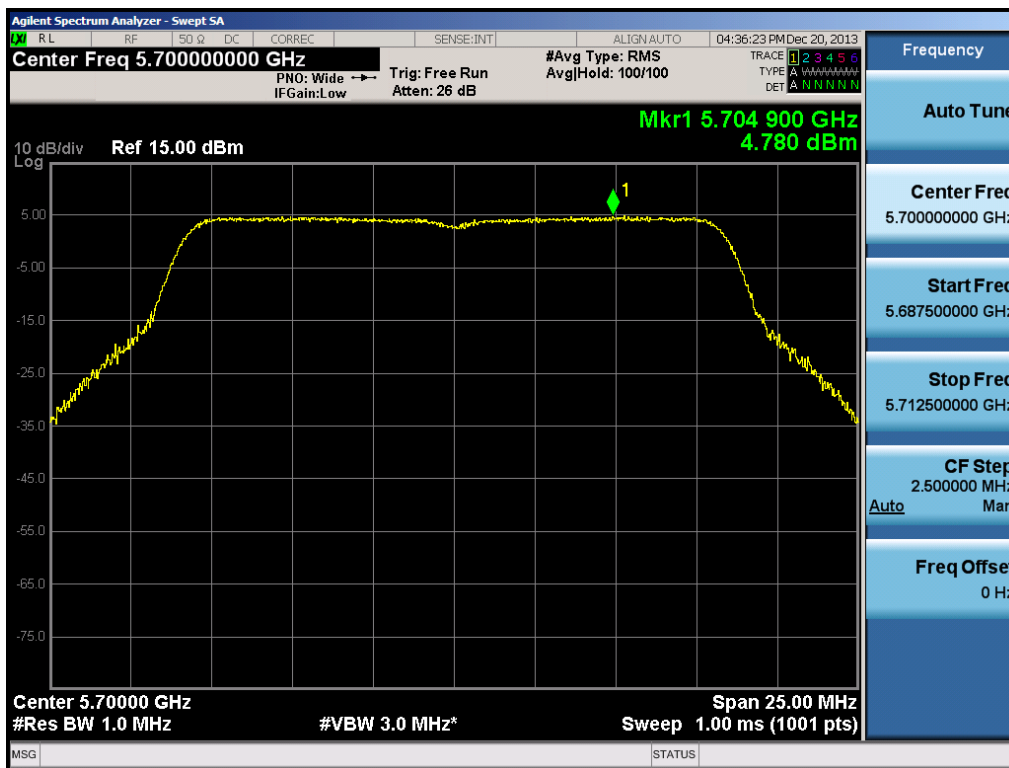
Plot 6-56. Peak Power Spectral Density Plot (802.11a (UNII Band 2C) – Ch. 140)
