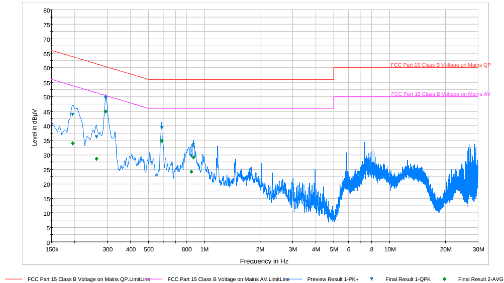
Plot 6-98. Line Conducted Plot with 802.11a UNII Band 2A (N)
