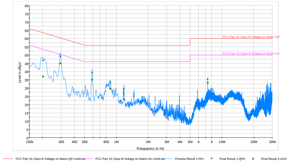
Plot 6-95. Line Conducted Plot with 802.11a UNII Band 1 (L1)
