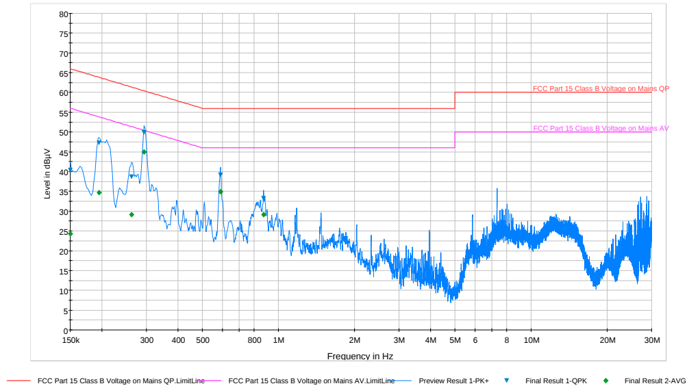
Plot 6-96. Line Conducted Plot with 802.11a UNII Band 1 (N)
