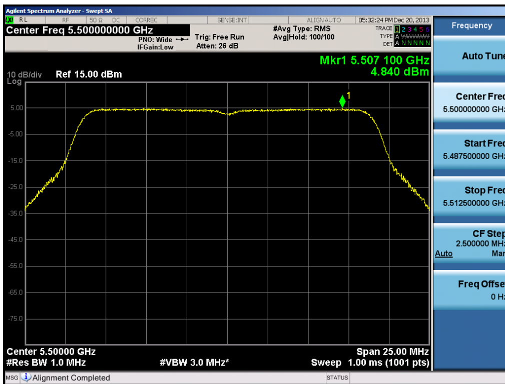
Plot 6-57. Peak Power Spectral Density Plot (20MHz BW 802.11n (UNII Band 2C) – Ch. 100)
