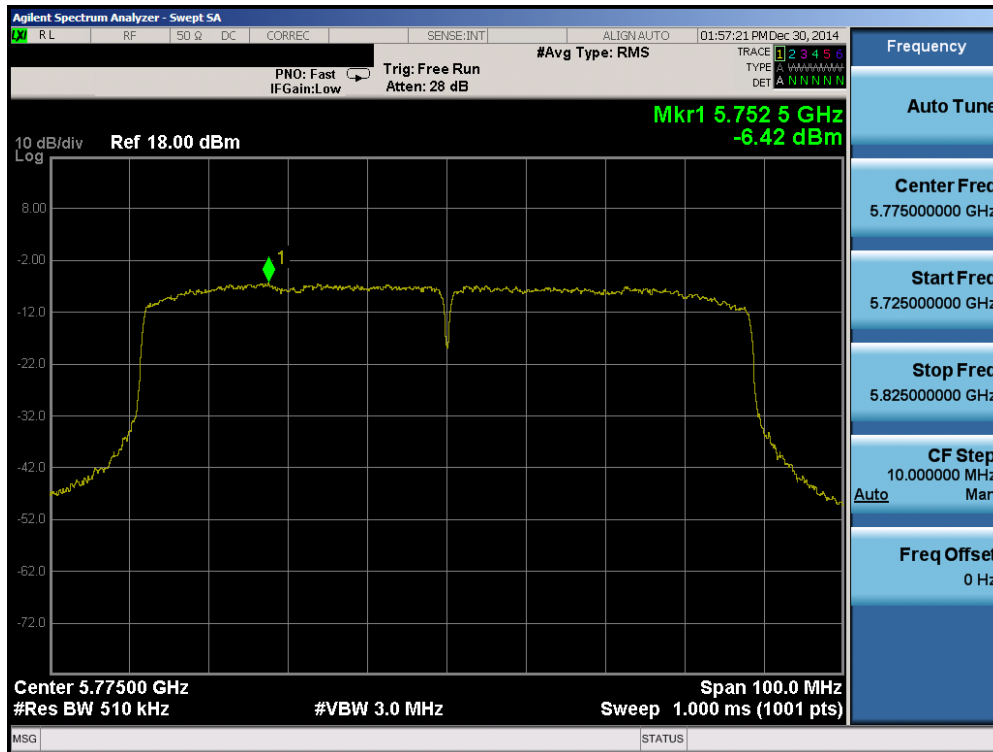
Plot 6-76. Peak Power Spectral Density Plot (80MHz BW 802.11ac (UNII Band 3) – Ch. 155)
