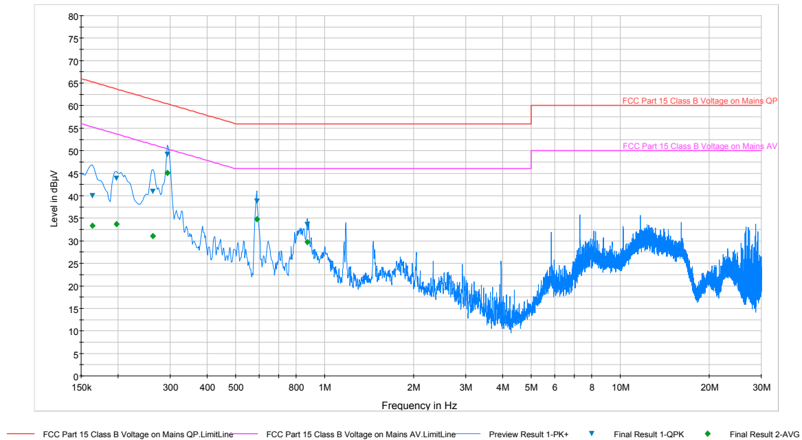
Plot 6-71. Line Conducted Plot with 802.11b (N)
