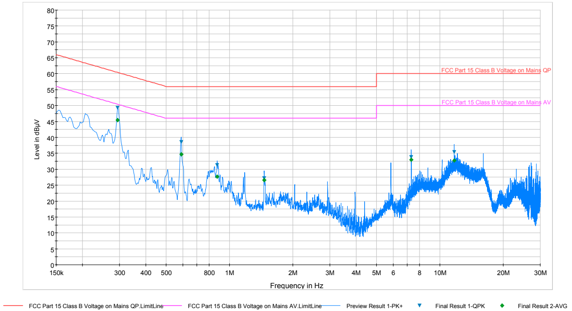
Plot 6-70. Line Conducted Plot with 802.11b (L1)
