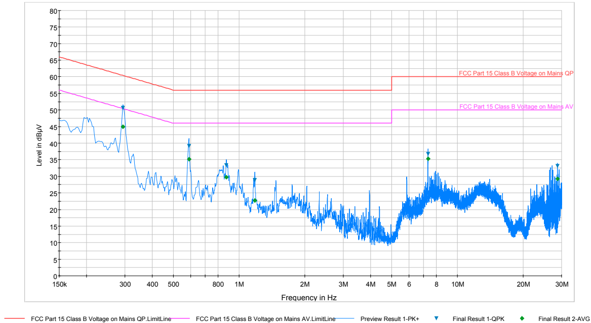
Plot 6-72. Line Conducted Plot with 802.11a (L1)
