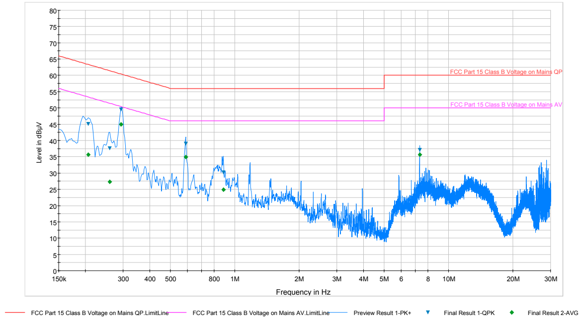
Plot 6-73. Line Conducted Plot with 802.11a (N)
