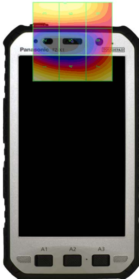
Figure 18-4 E-Field WD Scan overlay
