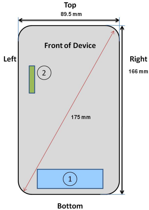
Figure F-1 DUT Antenna Locations
