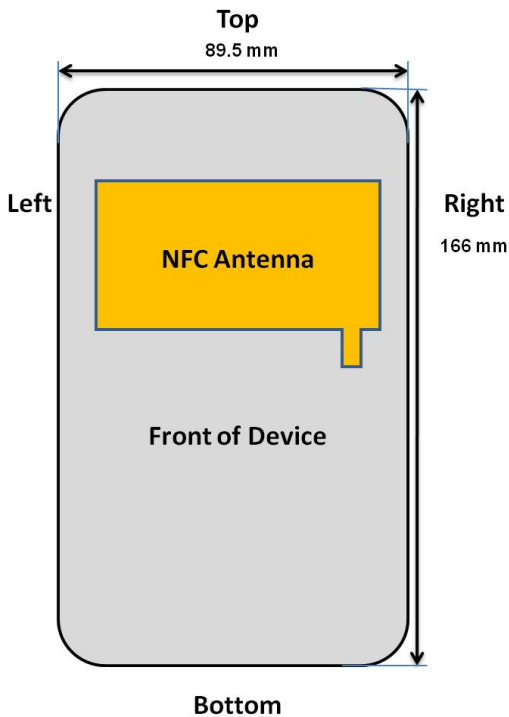
Figure F-2 NFC Antenna Location
