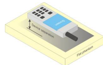
Figure 6-4 Sample Body-Worn Diagram
