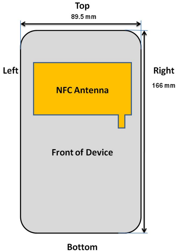
Figure 1-2 NFC Antenna Locations
