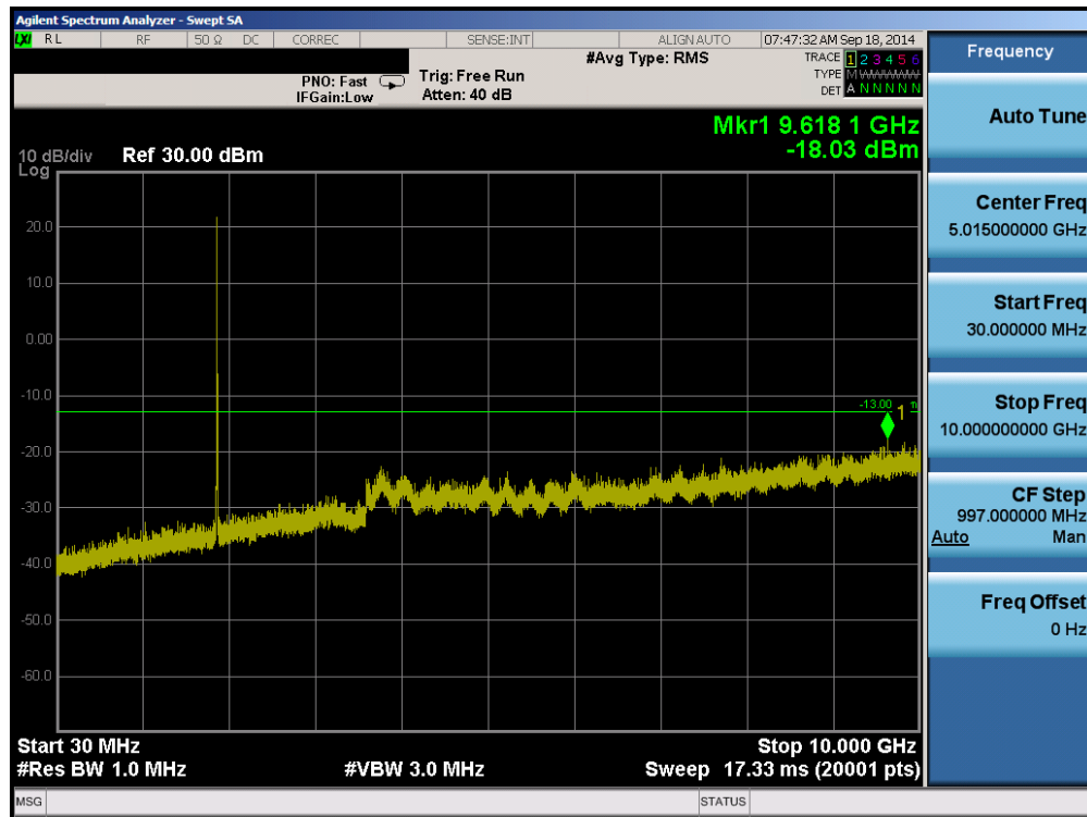
Plot 6-44. Conducted Spurious Plot (PCS WCDMA Mode – Ch. 9400)
