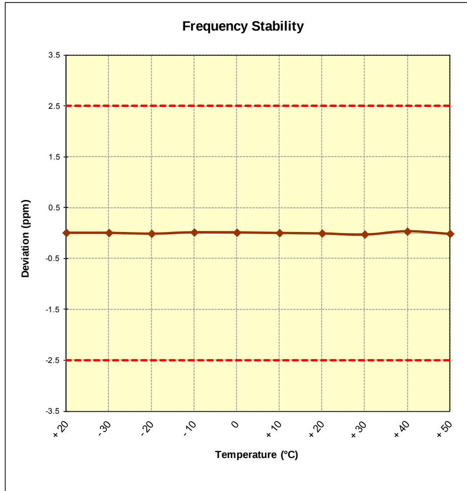
Figure 6-9. Frequency Stability Graph (Cellular WCDMA Mode – Ch. 4183)
