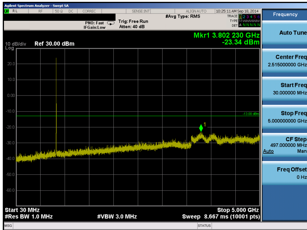
Plot 6-28. Conducted Spurious Plot (Cellular CDMA Mode – Ch. 777)
