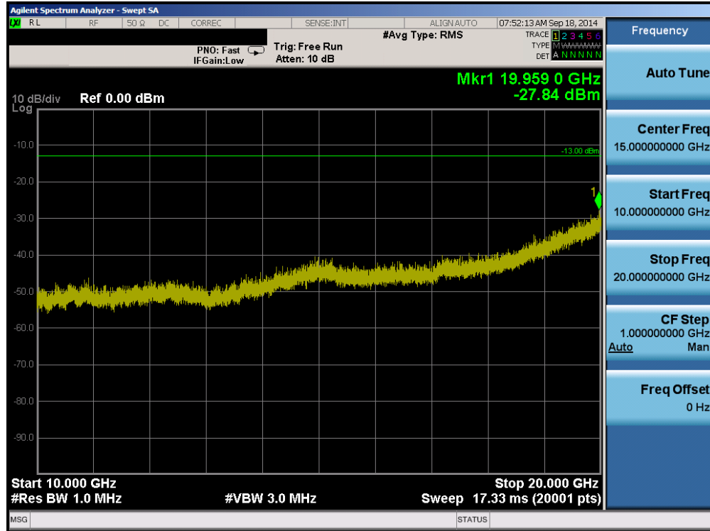
Plot 6-43. Conducted Spurious Plot (PCS WCDMA Mode – Ch. 9262)
