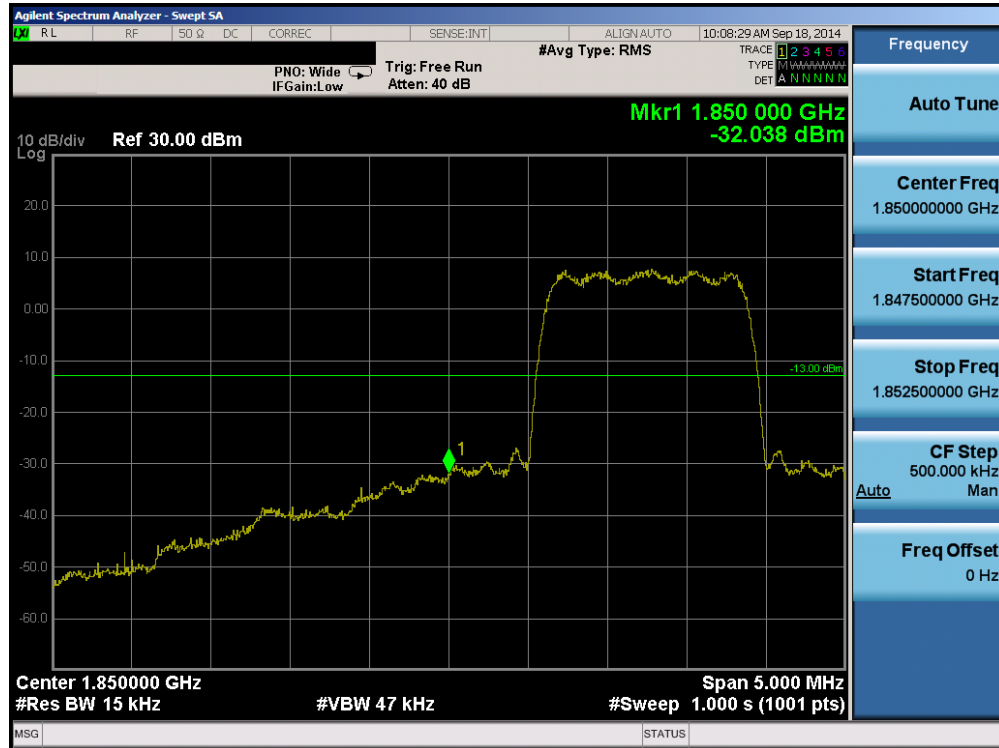
Plot 6-56. Band Edge Plot (PCS CDMA Mode – Ch. 25)
