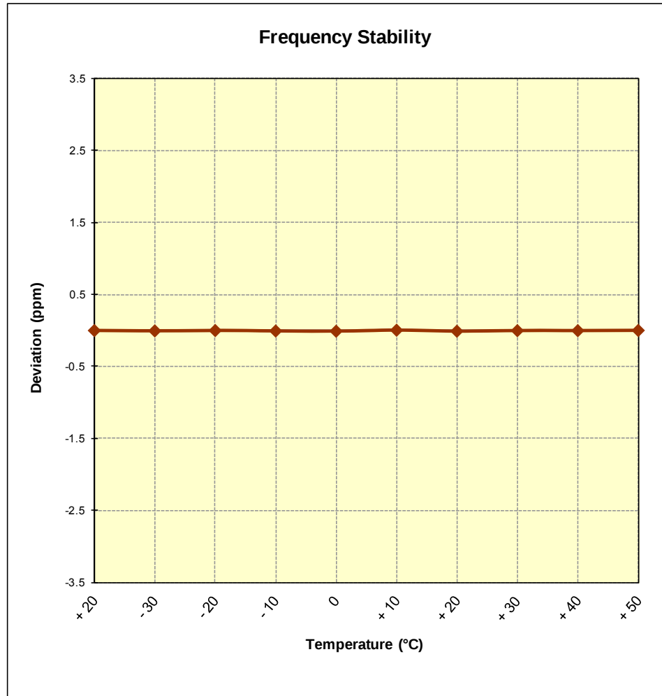
Figure 6-12. Frequency Stability Graph (PCS WCDMA Mode – Ch. 9400)
