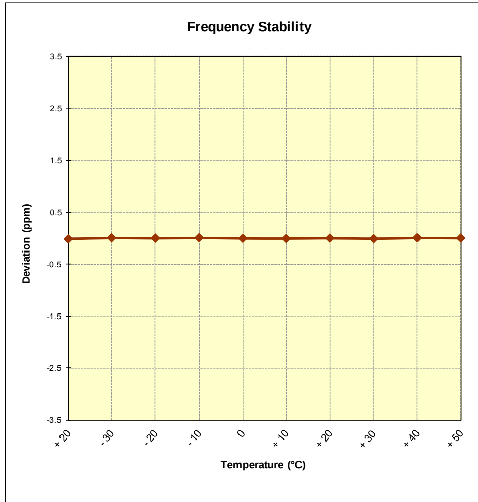
Figure 6-11. Frequency Stability Graph (PCS CDMA Mode – Ch. 600)
