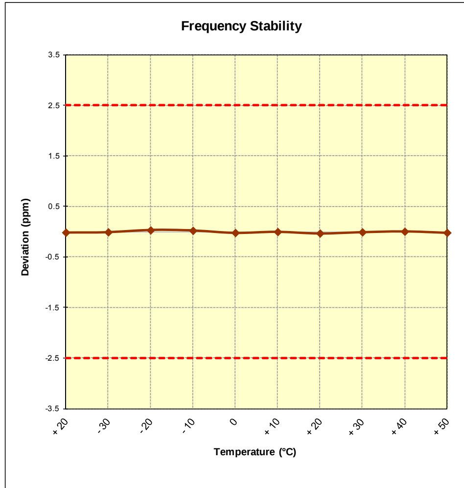
Figure 6-8. Frequency Stability Graph (Cellular CDMA Mode – Ch. 384)
