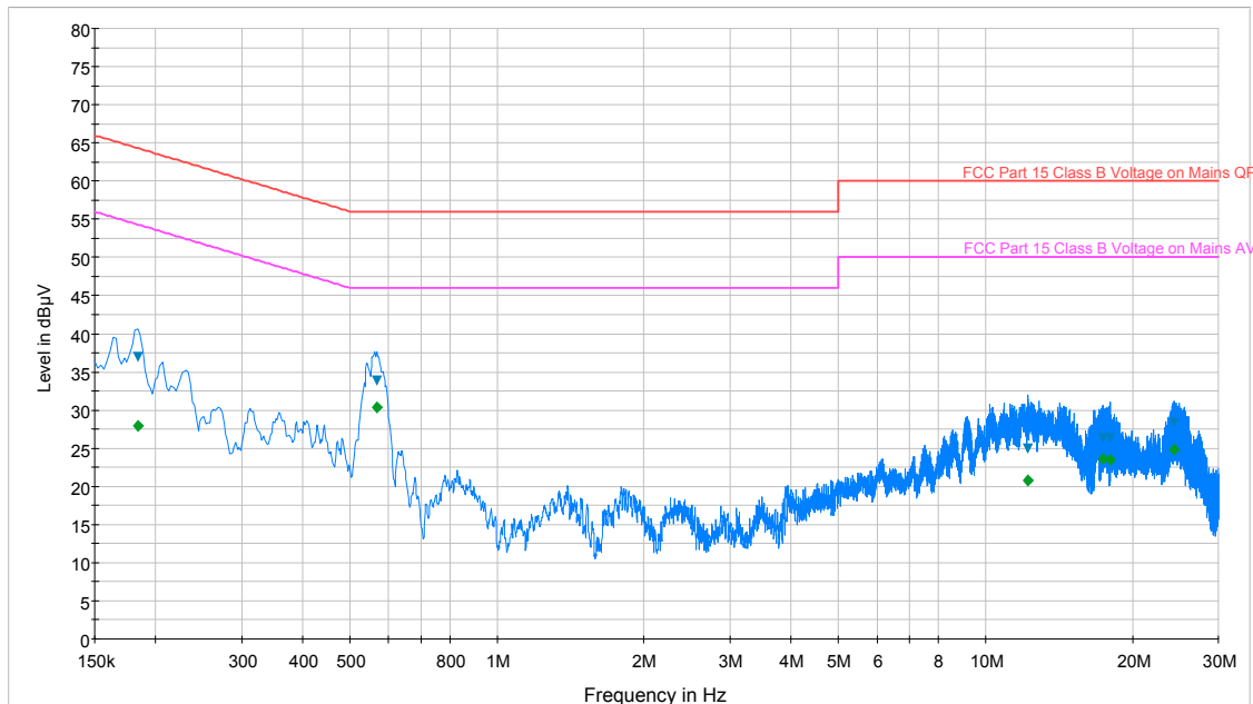
Plot 6-116. Line Conducted Plot with 802.11a UNII Band 2A (L1)
