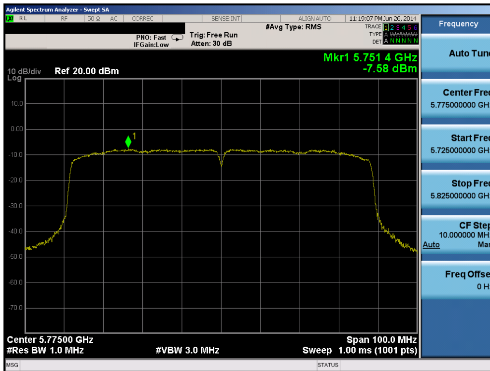
Plot 6-82. Peak Power Spectral Density Plot (80MHz BW 802.11ac (UNII Band 3) – Ch. 155)
