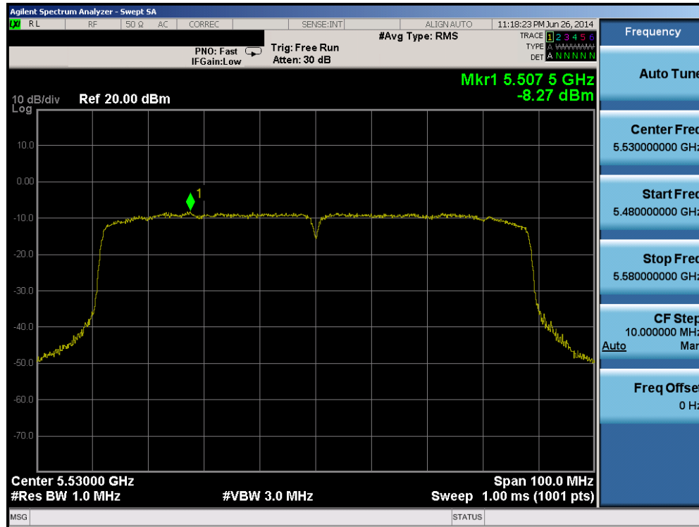
Plot 6-72. Peak Power Spectral Density Plot (80MHz BW 802.11ac (UNII Band 2C) – Ch. 106)
