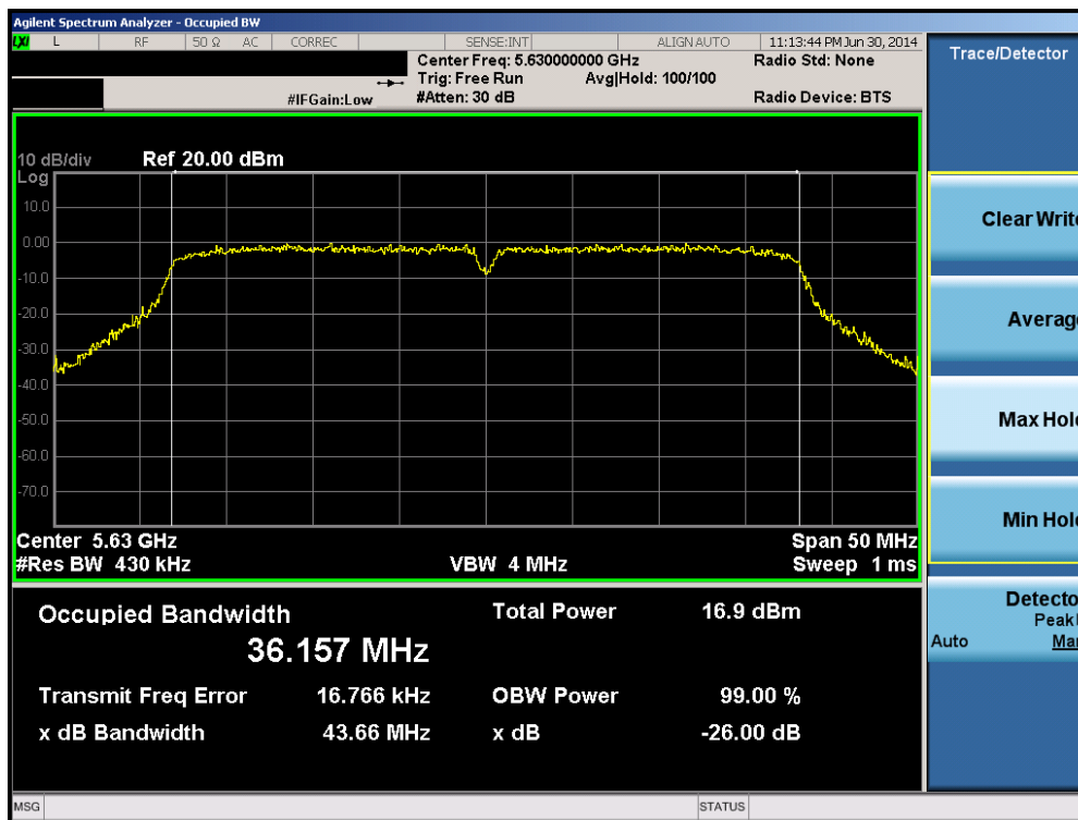
Plot 6-27. 26dB Bandwidth Plot (40MHz BW 802.11n (UNII Band 2C) – Ch. 126)
