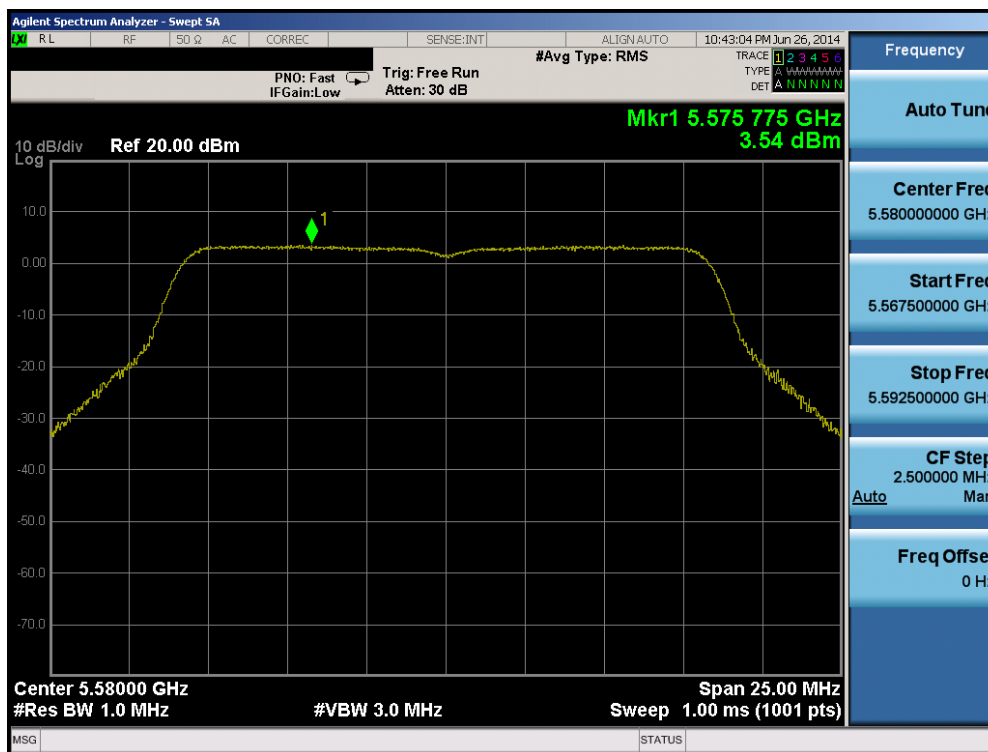
Plot 6-63. Peak Power Spectral Density Plot (802.11a (UNII Band 2C) – Ch. 116)
