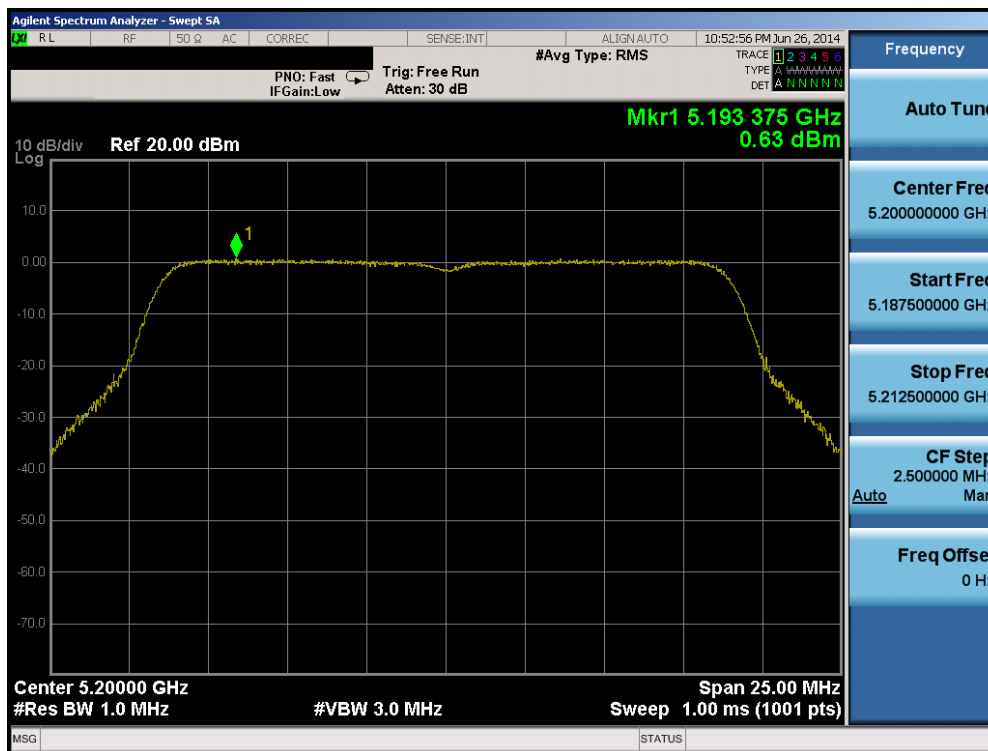
Plot 6-48. Peak Power Spectral Density Plot (20MHz BW 802.11n (UNII Band 1) – Ch. 40)
