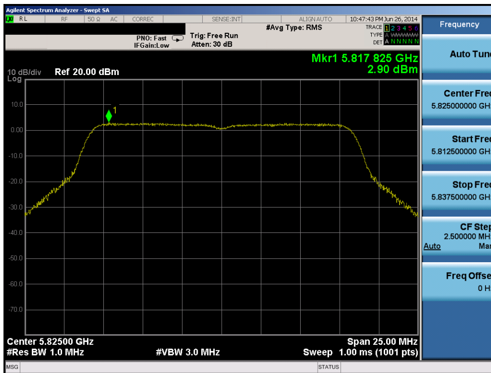
Plot 6-76. Peak Power Spectral Density Plot (802.11a (UNII Band 3) – Ch. 165)
