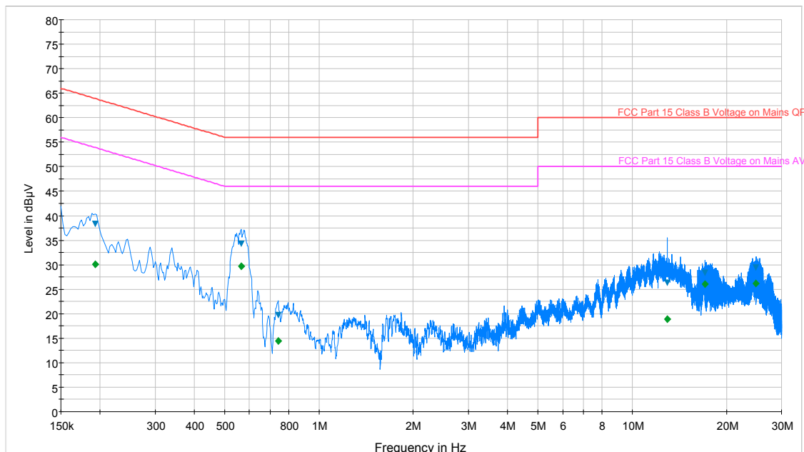
Plot 6-114. Line Conducted Plot with 802.11a UNII Band 1 (L1)
