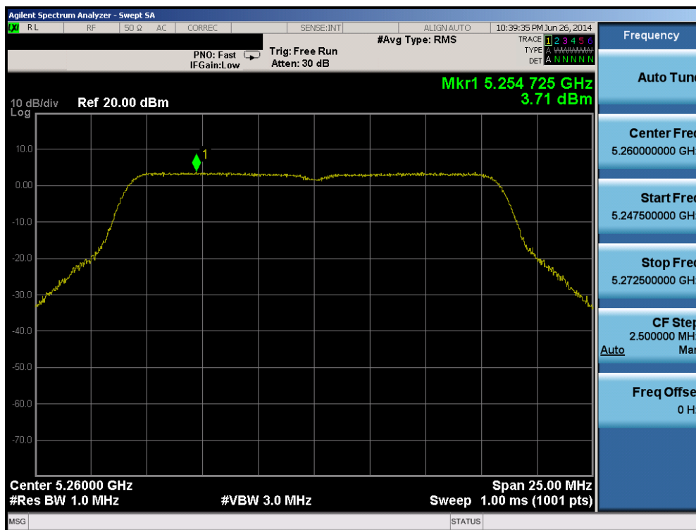
Plot 6-53. Peak Power Spectral Density Plot (802.11a (UNII Band 2A) – Ch. 52)
