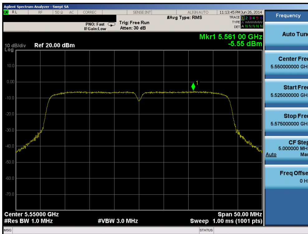
Plot 6-69. Peak Power Spectral Density Plot (40MHz BW 802.11n (UNII Band 2C) – Ch. 110)
