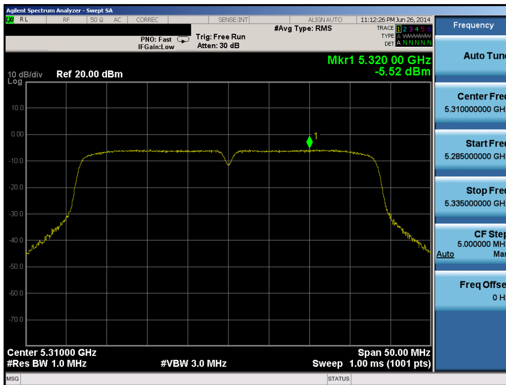
Plot 6-60. Peak Power Spectral Density Plot (40MHz BW 802.11n (UNII Band 2A) – Ch. 62)
