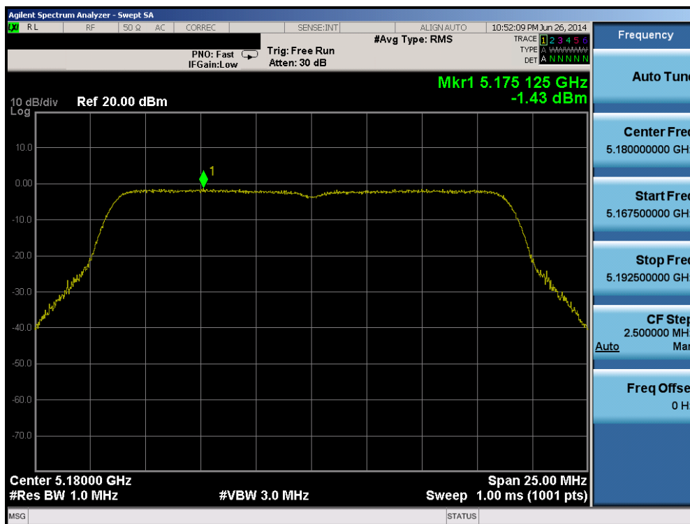
Plot 6-47. Peak Power Spectral Density Plot (20MHz BW 802.11n (UNII Band 1) – Ch. 36)
