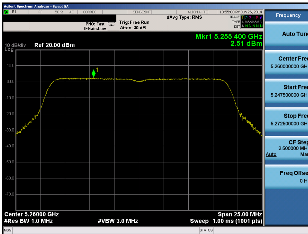
Plot 6-56. Peak Power Spectral Density Plot (20MHz BW 802.11n (UNII Band 2A) – Ch. 52)
