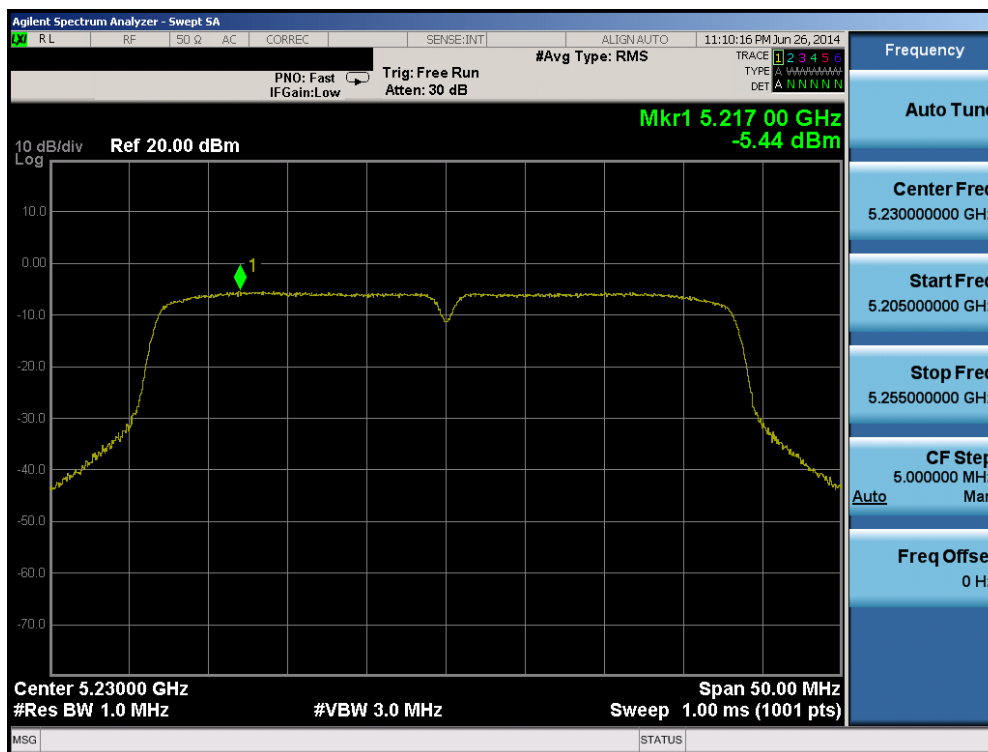
Plot 6-51. Peak Power Spectral Density Plot (40MHz BW 802.11n (UNII Band 1) – Ch. 46)
