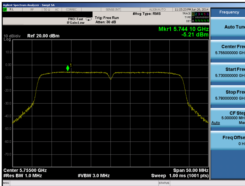
Plot 6-80. Peak Power Spectral Density Plot (40MHz BW 802.11n (UNII Band 3) – Ch. 151)
