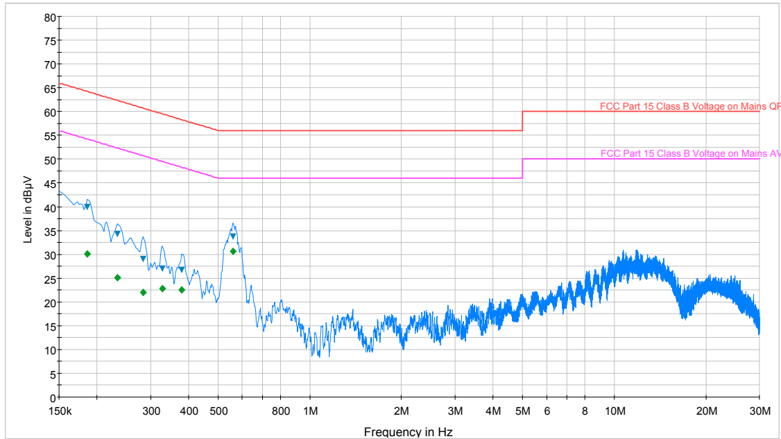
Plot 6-115. Line Conducted Plot with 802.11a UNII Band 1 (N)
