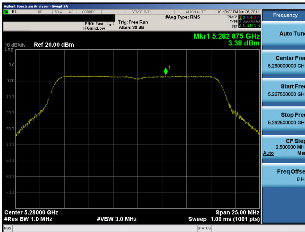
Plot 6-54. Peak Power Spectral Density Plot (802.11a (UNII Band 2A) – Ch. 56)
