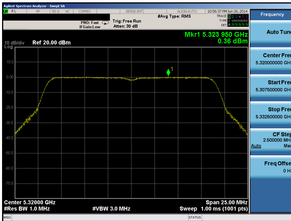
Plot 6-58. Peak Power Spectral Density Plot (20MHz BW 802.11n (UNII Band 2A) – Ch. 64)
