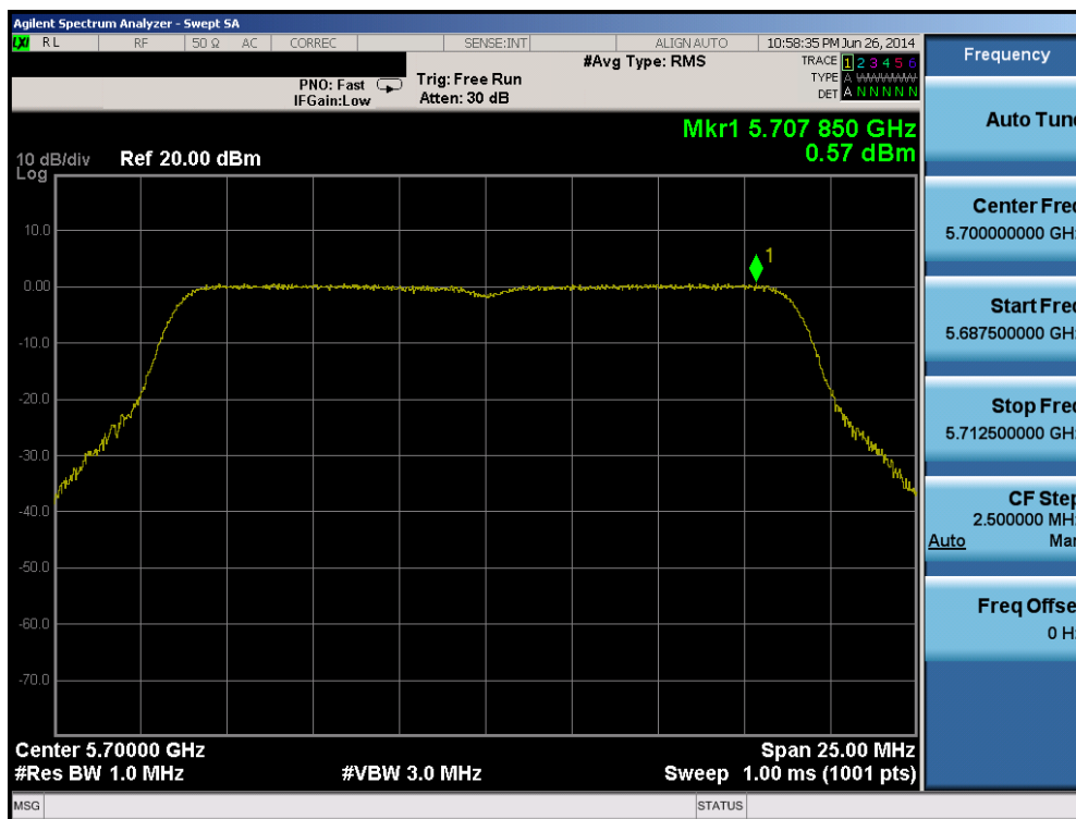
Plot 6-67. Peak Power Spectral Density Plot (20MHz BW 802.11n (UNII Band 2C) – Ch. 140)
