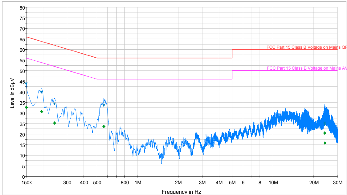
Plot 6-121. Line Conducted Plot with 802.11a UNII Band 3 (N)
