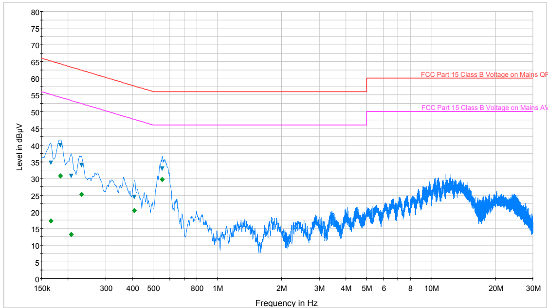
Plot 6-117. Line Conducted Plot with 802.11a UNII Band 2A (N)
