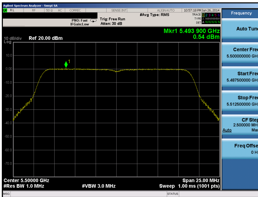
Plot 6-65. Peak Power Spectral Density Plot (20MHz BW 802.11n (UNII Band 2C) – Ch. 100)
