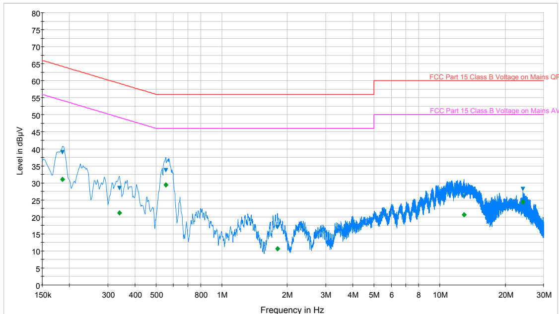
Plot 6-120. Line Conducted Plot with 802.11a UNII Band 3 (L1)
