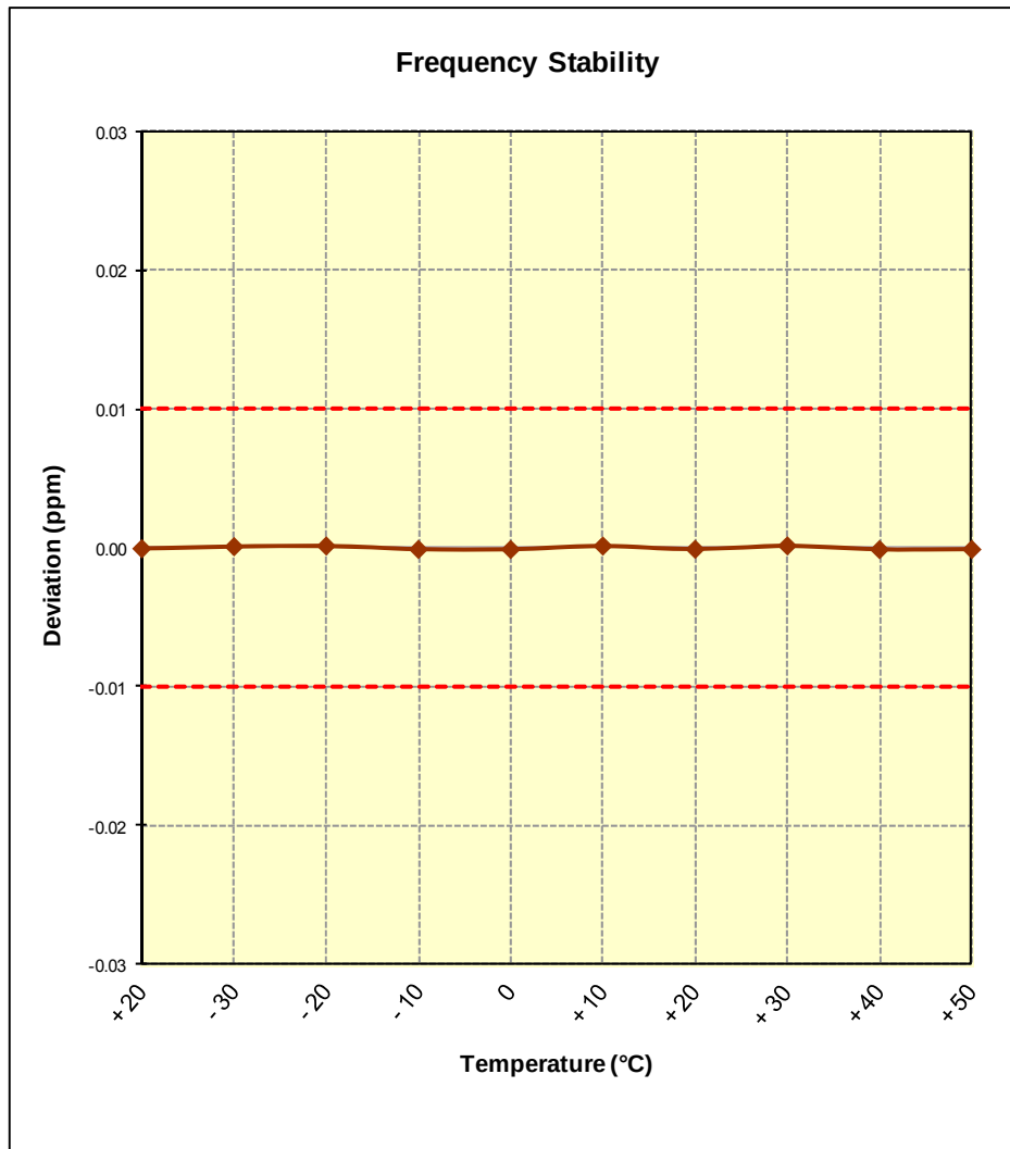
Figure 8-3. Frequency Stability Plot
