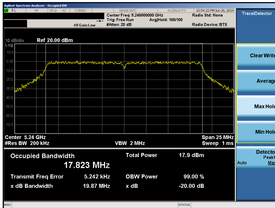
Plot 6-32. 20dB Bandwidth Plot (20MHz BW 802.11n (UNII Band 1) – Ch. 48)
