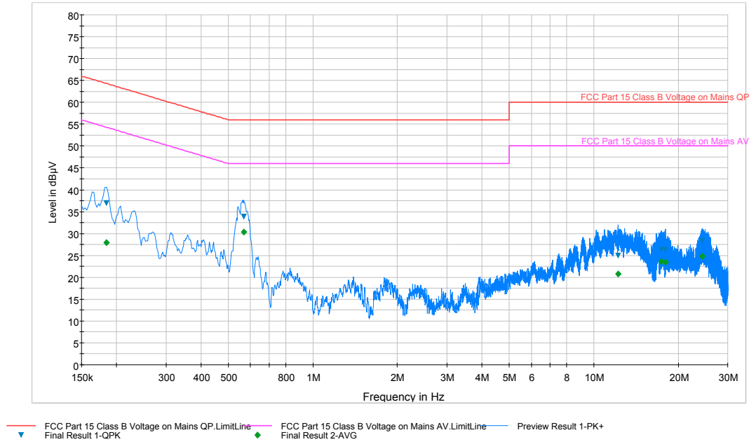
Plot 6-116. Line Conducted Plot with 802.11a UNII Band 2A (L1)
