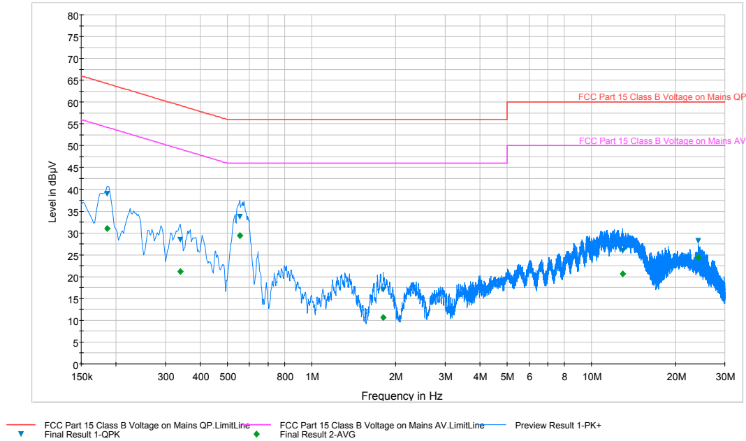
Plot 6-120. Line Conducted Plot with 802.11a UNII Band 3 (L1)
