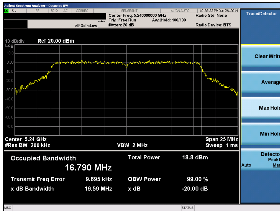
Plot 6-31. 20dB Bandwidth Plot (20MHz BW 802.11a (UNII Band 1) – Ch. 48)
