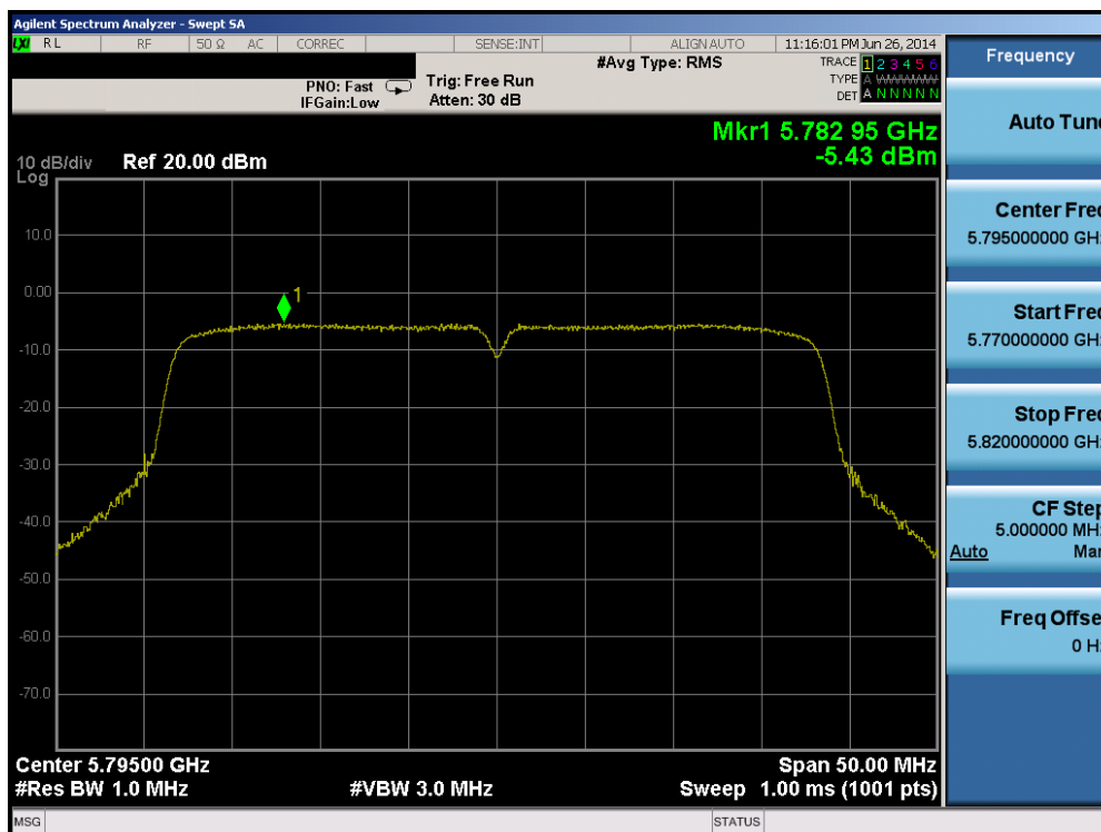
Plot 6-81. Peak Power Spectral Density Plot (40MHz BW 802.11n (UNII Band 3) – Ch. 159)
