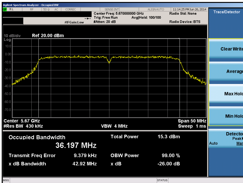
Plot 6-28. 26dB Bandwidth Plot (40MHz BW 802.11n (UNII Band 2C) – Ch. 134)
