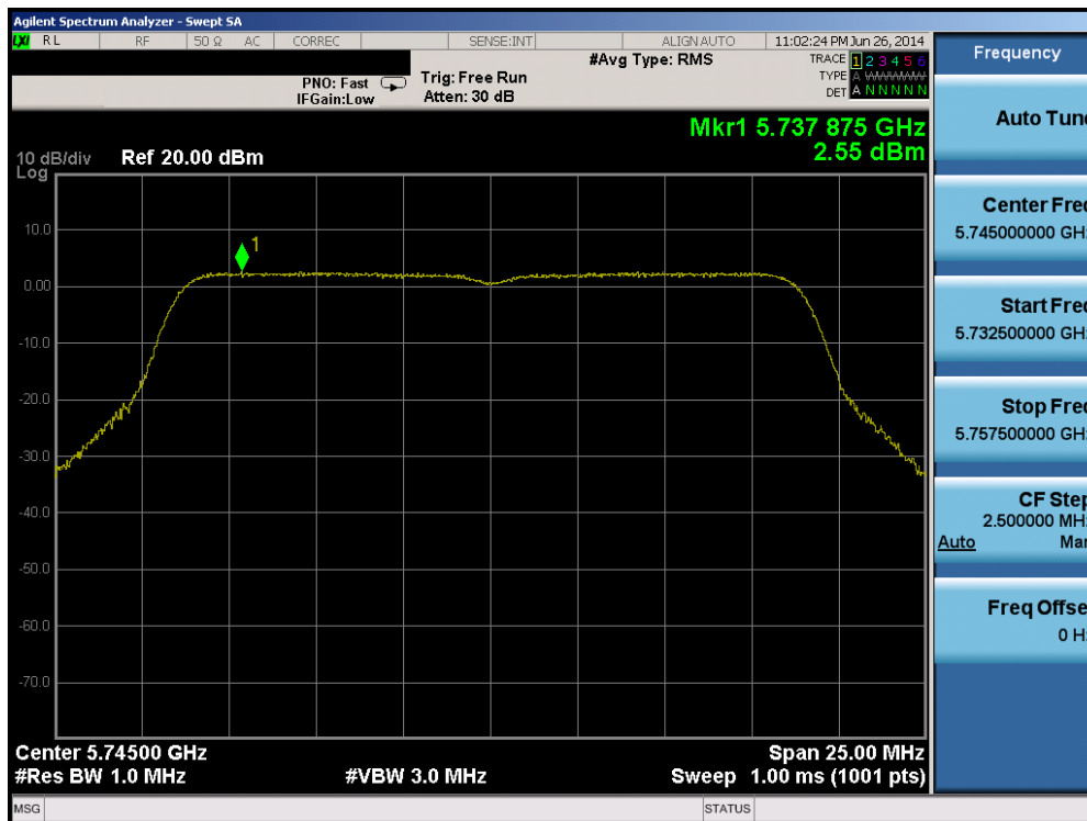
Plot 6-77. Peak Power Spectral Density Plot (20MHz BW 802.11n (UNII Band 3) – Ch. 149)
