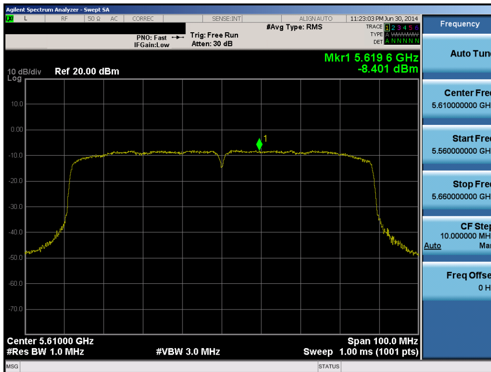
Plot 6-73. Peak Power Spectral Density Plot (80MHz BW 802.11ac (UNII Band 2C) – Ch. 122)
