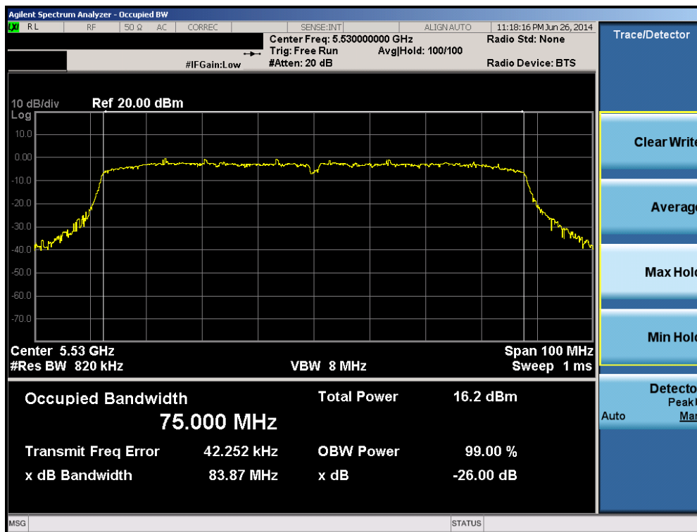
Plot 6-29. 26dB Bandwidth Plot (80MHz BW 802.11ac (UNII Band 2C) – Ch. 106
