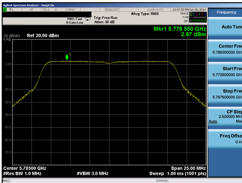
Plot 6-75. Peak Power Spectral Density Plot (802.11a (UNII Band 3) – Ch. 157)
