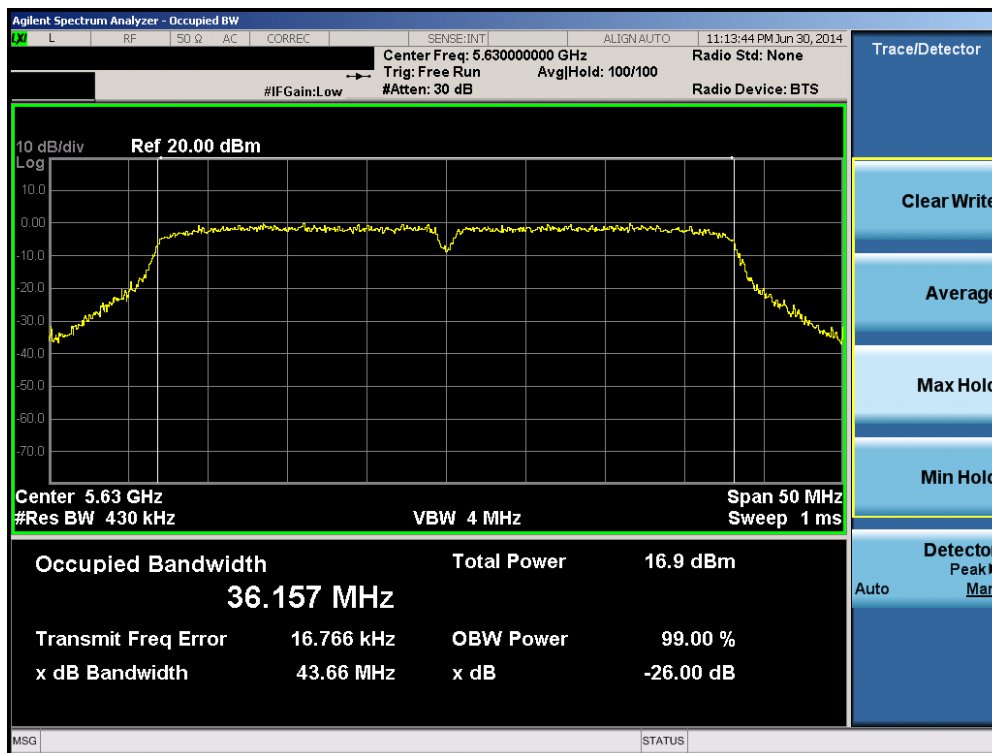
Plot 6-27. 26dB Bandwidth Plot (40MHz BW 802.11n (UNII Band 2C) – Ch. 126)
