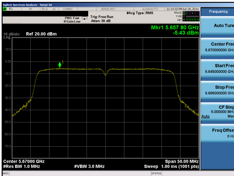
Plot 6-71. Peak Power Spectral Density Plot (40MHz BW 802.11n (UNII Band 2C) – Ch. 134)
