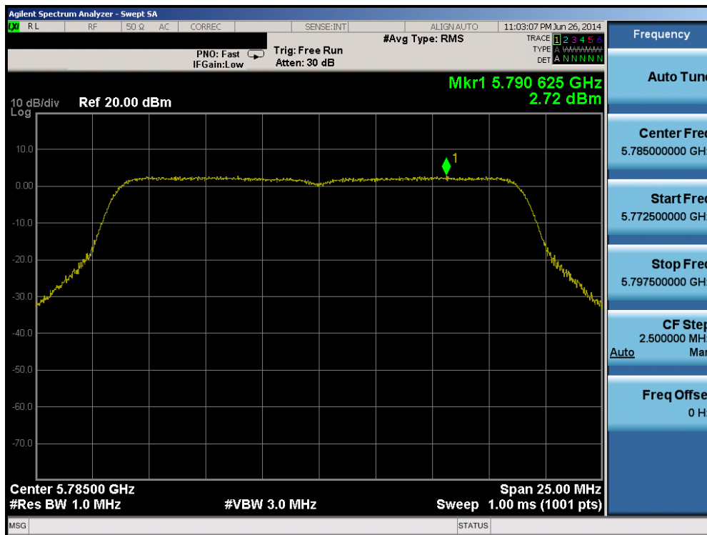
Plot 6-78. Peak Power Spectral Density Plot (20MHz BW 802.11n (UNII Band 3) – Ch. 157)
