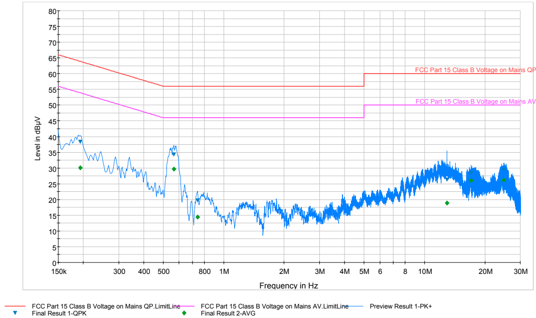
Plot 6-114. Line Conducted Plot with 802.11a UNII Band 1 (L1)
