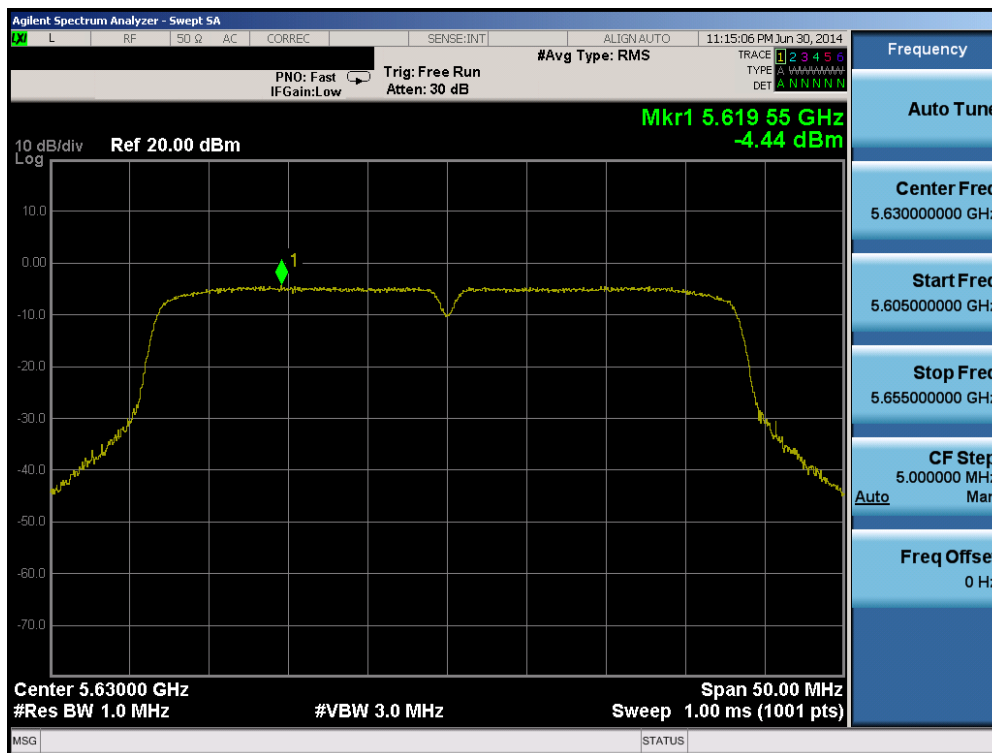
Plot 6-70. Peak Power Spectral Density Plot (40MHz BW 802.11n (UNII Band 2C) – Ch. 126)
