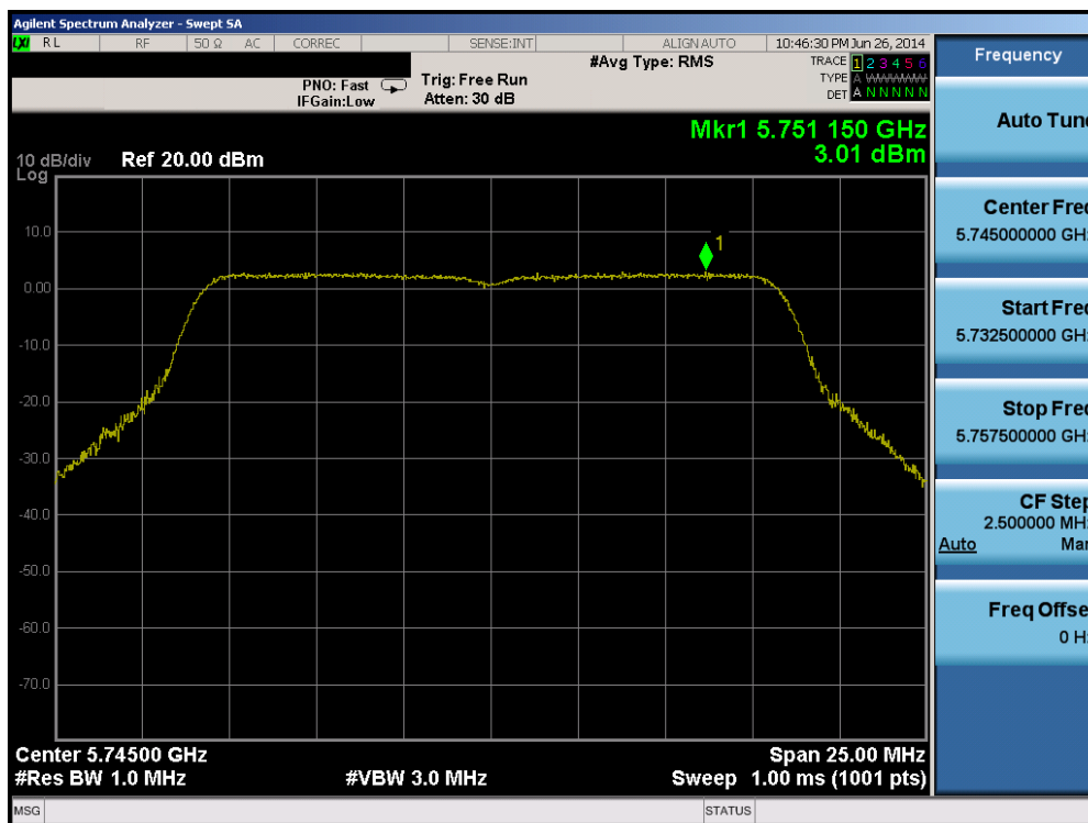
Plot 6-74. Peak Power Spectral Density Plot (802.11a (UNII Band 3) – Ch. 149)
