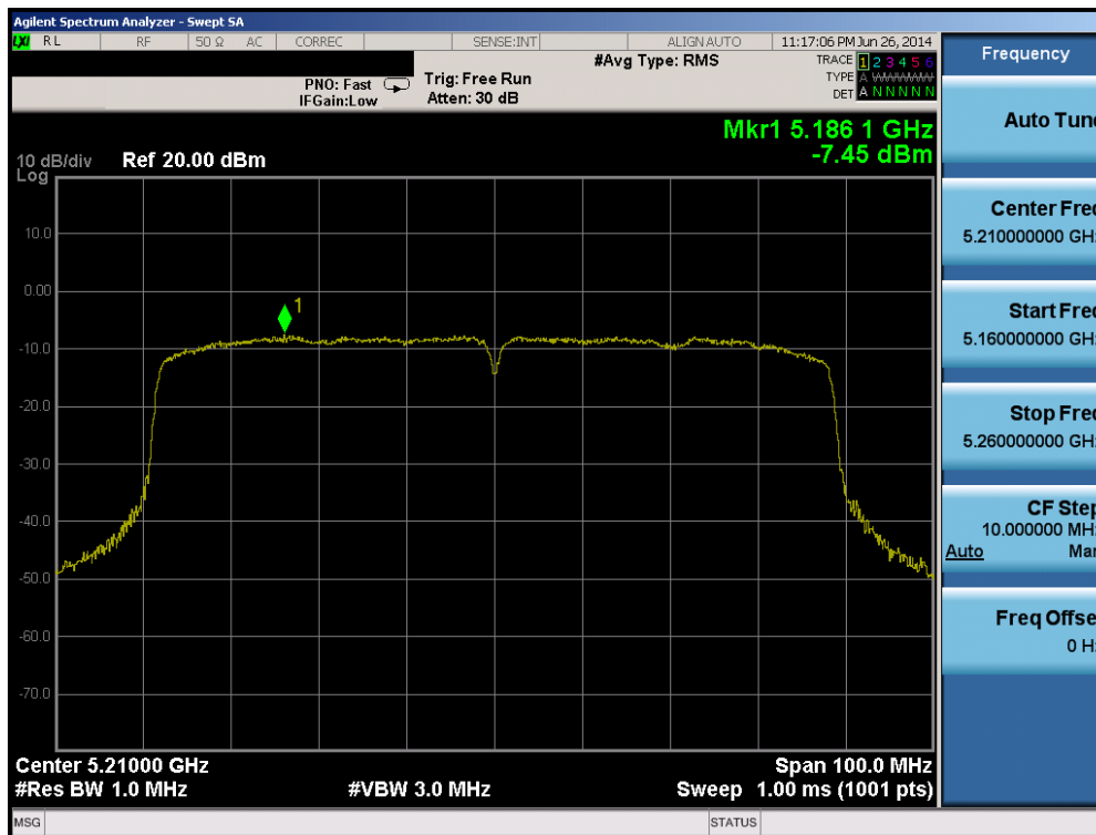
Plot 6-52. Peak Power Spectral Density Plot (80MHz BW 802.11ac (UNII Band 1) – Ch. 42)
