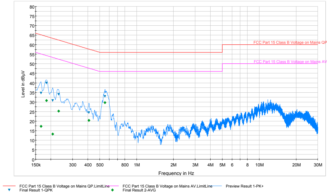
Plot 6-117. Line Conducted Plot with 802.11a UNII Band 2A (N)
