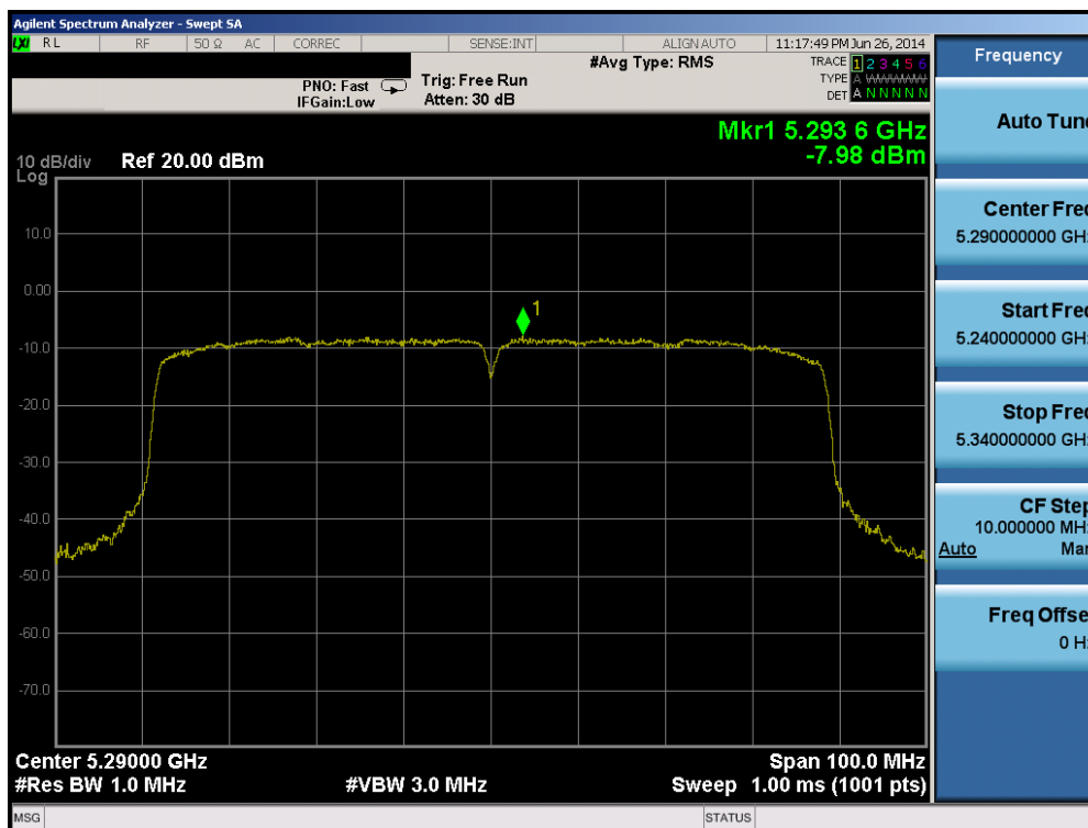
Plot 6-61. Peak Power Spectral Density Plot (80MHz BW 802.11ac (UNII Band 2A) – Ch. 58)
