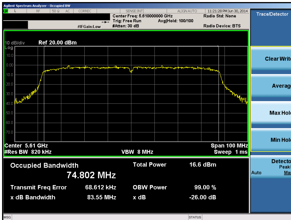
Plot 6-30. 26dB Bandwidth Plot (80MHz BW 802.11ac (UNII Band 2C) – Ch. 122
