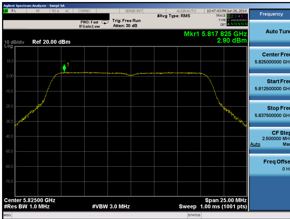
Plot 6-76. Peak Power Spectral Density Plot (802.11a (UNII Band 3) – Ch. 165)
