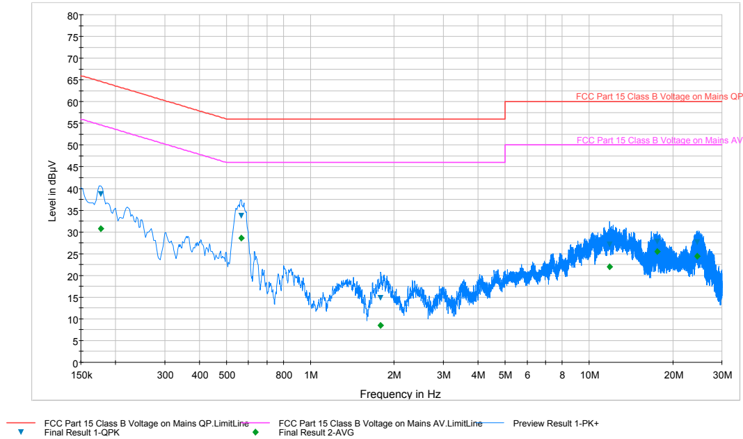
Plot 6-118. Line Conducted Plot with 802.11a UNII Band 2C (L1)
