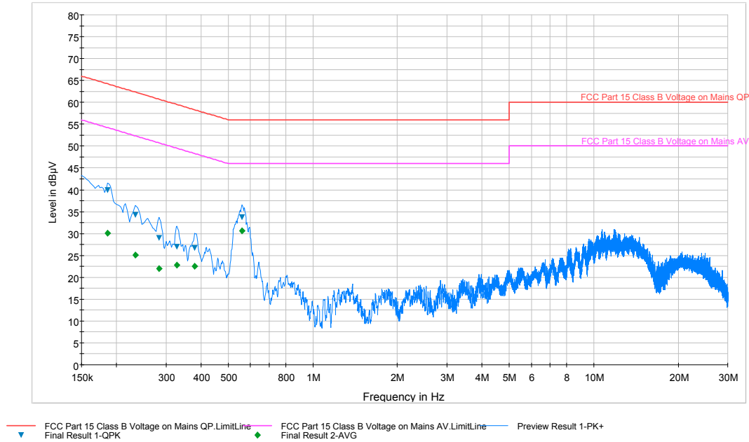
Plot 6-115. Line Conducted Plot with 802.11a UNII Band 1 (N)
