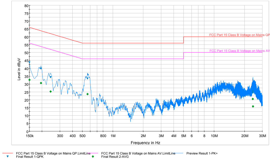
Plot 6-121. Line Conducted Plot with 802.11a UNII Band 3 (N)
