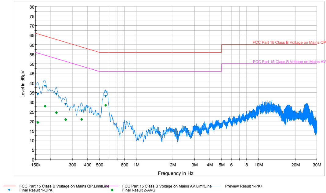
Plot 6-119. Line Conducted Plot with 802.11a UNII Band 2C (N)
