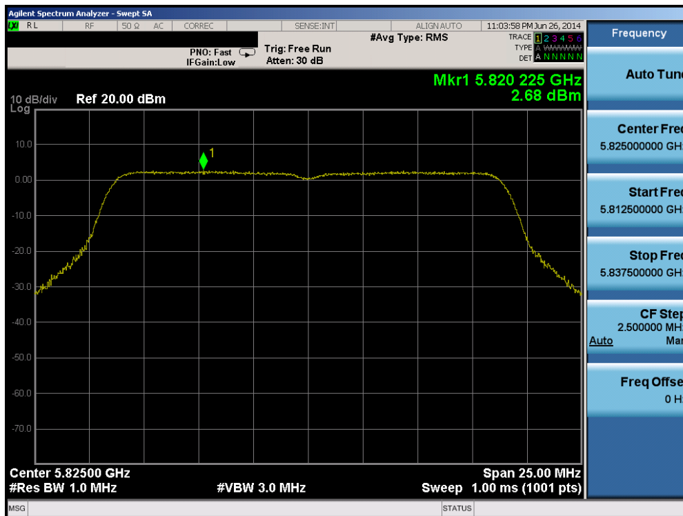
Plot 6-79. Peak Power Spectral Density Plot (20MHz BW 802.11n (UNII Band 3) – Ch. 165)
