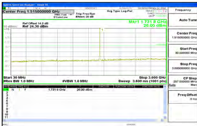
30MHz-3GHz_Band4_3MHz_QPSK_1_0_MidCH20175-1732.5
