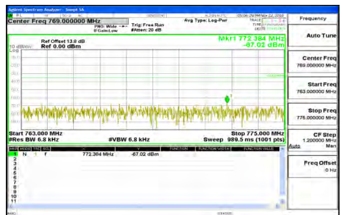
763.3MHz~775MHz_Band13_5MHz_QPSK_1_0_HighCH23255-784.5
