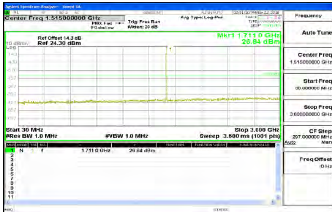
30MHz-3GHz_Band4_3MHz_QPSK_1_0_LowCH19965-1711.5
