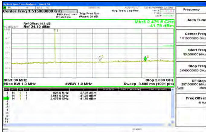
30MHz~3GHz_Band5_3MHz_QPSK_1_0_LowCH20415-825.5
