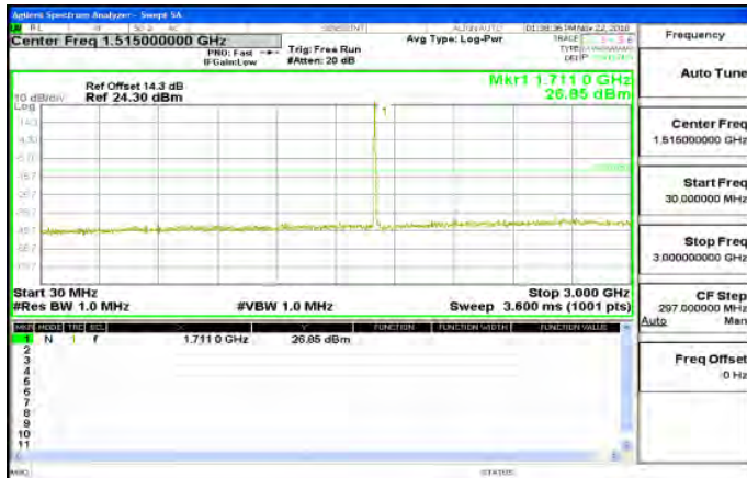
30MHz~3GHz_Band4_10MHz_QPSK_1_0_LowCH20000-1715
