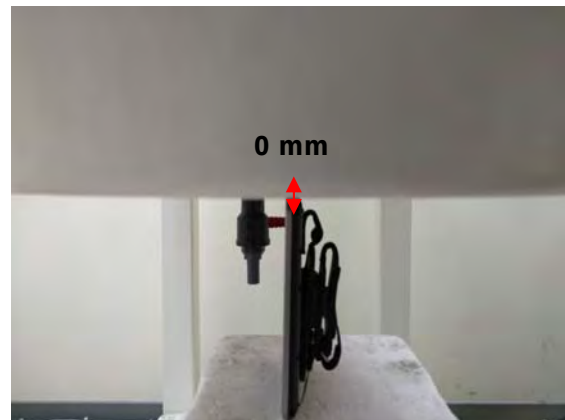
Fig.22 EUT Left side(Hand Strap 13U) to flat phantom
