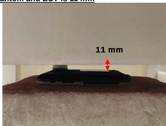
Fig.23 EUT Back side to flat phantom
