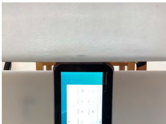
Fig.13 EUT Left side (Portrait scanner) to flat phantom
