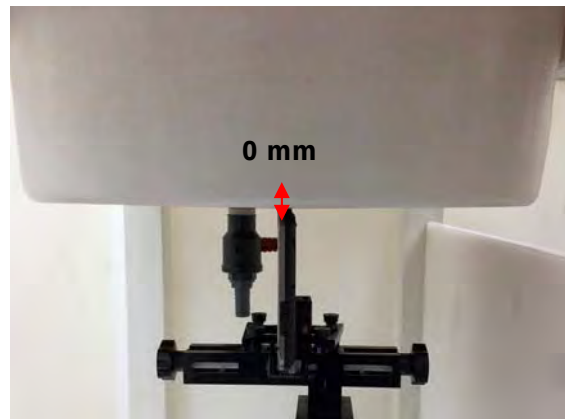
Fig.10 EUT Bottom side (Landscape scanner) to flat phantom
