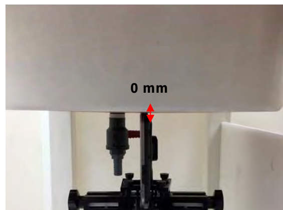
Fig.11 EUT Bottom side (Portrait scanner) to flat phantom
