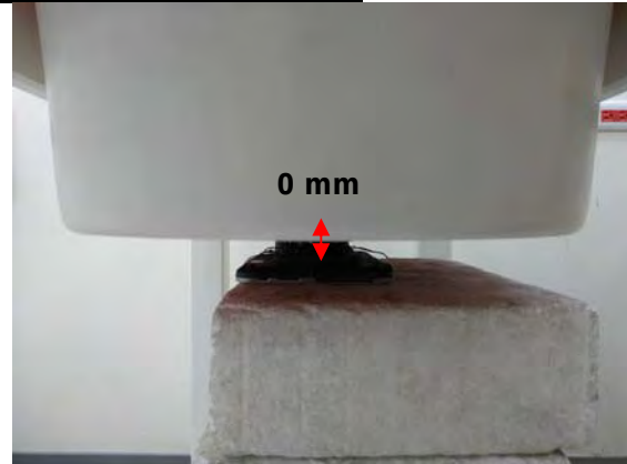
Fig.14 EUT Back side(Hand Strap 11U) to flat phantom
