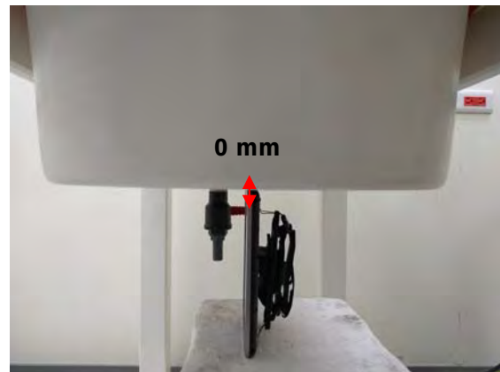
Fig.21 EUT Left side(Hand Strap 12U) to flat phantom
