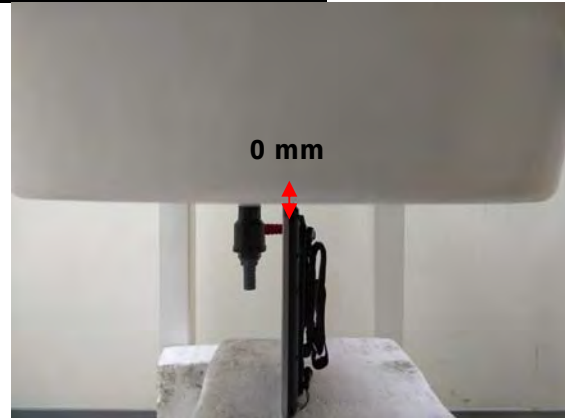
Fig.20 EUT Left side(Hand Strap 11U) to flat phantom
