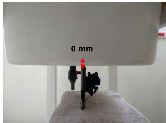
Fig.18 EUT Bottom side(Hand Strap 12U) to flat phantom
