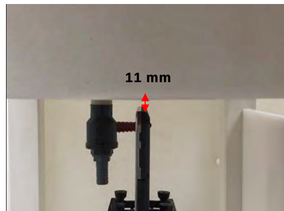
Fig.24 EUT Top side to flat phantom
