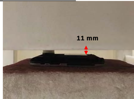
Fig.23 EUT Back side to flat phantom
