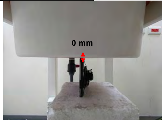
Fig.17 EUT Bottom side(Hand Strap 11U) to flat phantom
