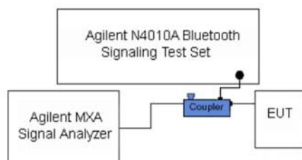
Figure 8-2 Bluetooth Power Measurement Setup
