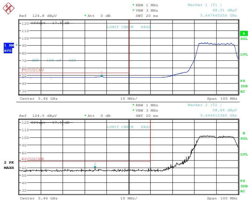
ACJFZN1A C2PC WLAN RSE Measurements
