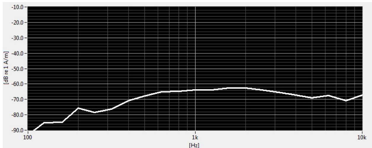
Figure 8-2 Worst-case ABM2 Plot for WLAN
