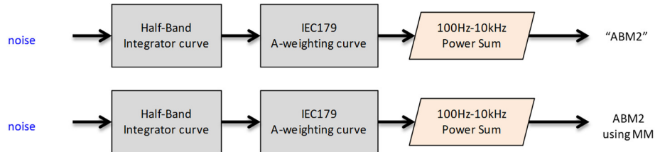
Figure 5-9 ABM2 Validation Block Diagram
