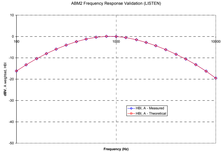
Figure 5-8 ABM2 Frequency Response Validation
