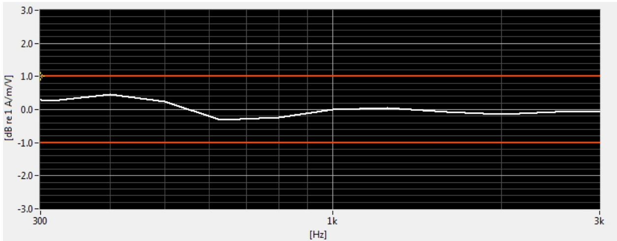
Figure 8-3 Helmholtz Coil Validation for Frequency Response
