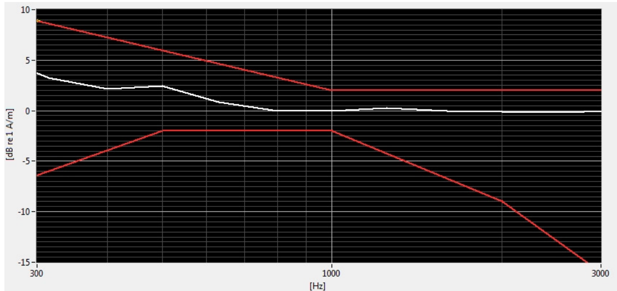
Figure 8-1 Axial Frequency Response
