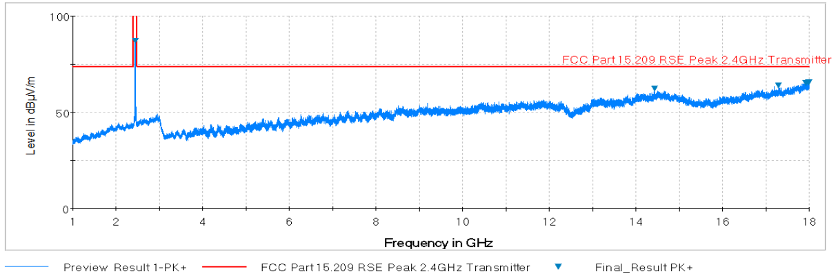
Plot 7-40. Radiated Spurious Plot above 1GHz (802.11b – Ch. 6, Ant. Pol. V)
