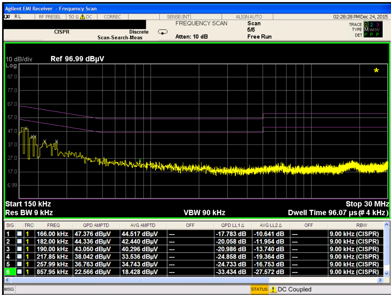
Plot 7-51. Line Conducted Plot with 802.11b (L1)
