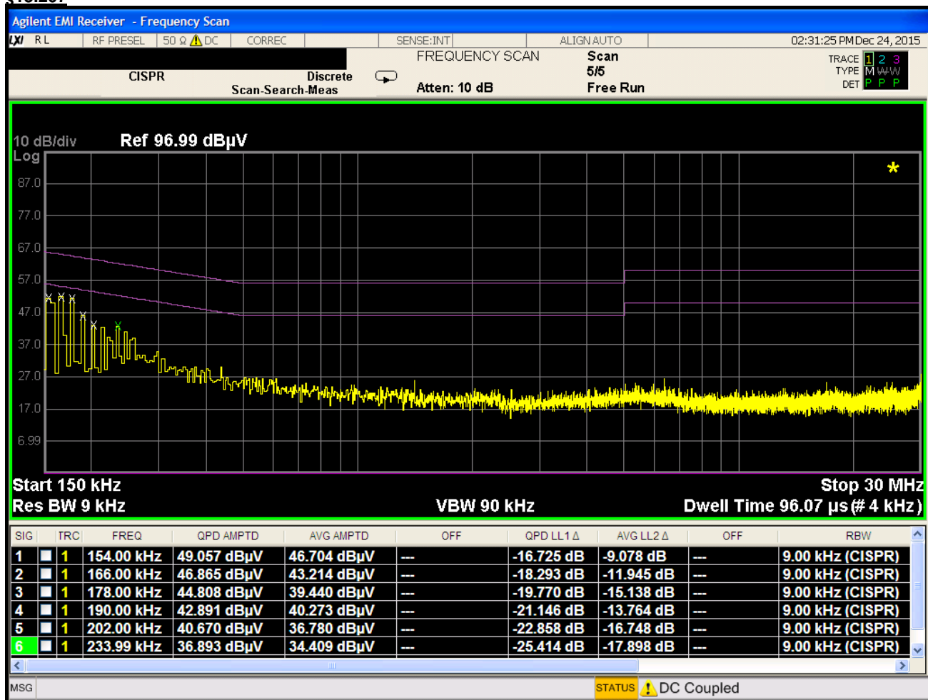
Plot 7-52. Line Conducted Plot with 802.11b (N)
