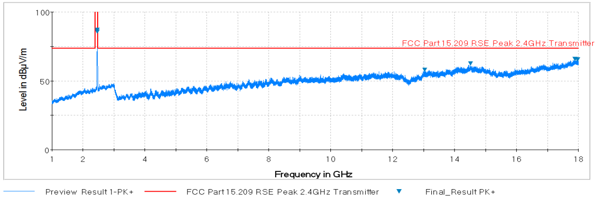
Plot 7-42. Radiated Spurious Plot above 1GHz (802.11b – Ch. 11, Ant. Pol. V)
