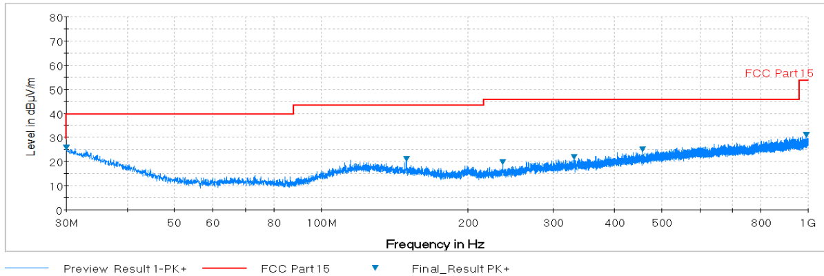
Plot 7-49. Radiated Spurious Plot below 1GHz (Pol. H)
