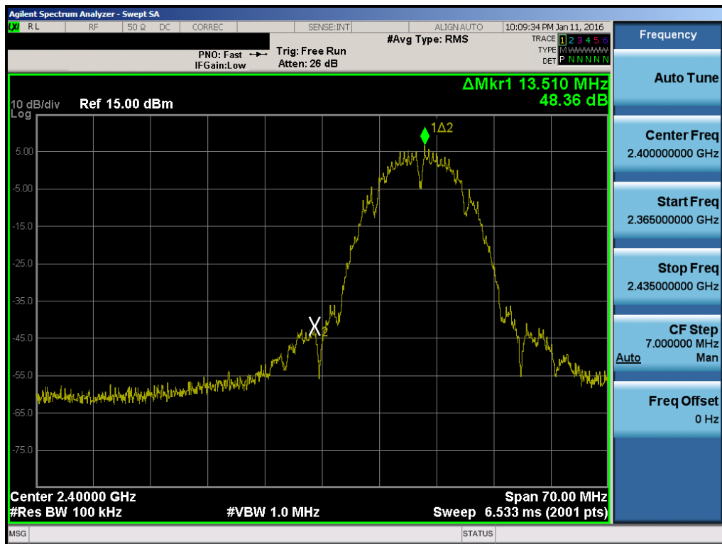
Plot 7-19. Band Edge Plot (802.11b – Ch. 1)
