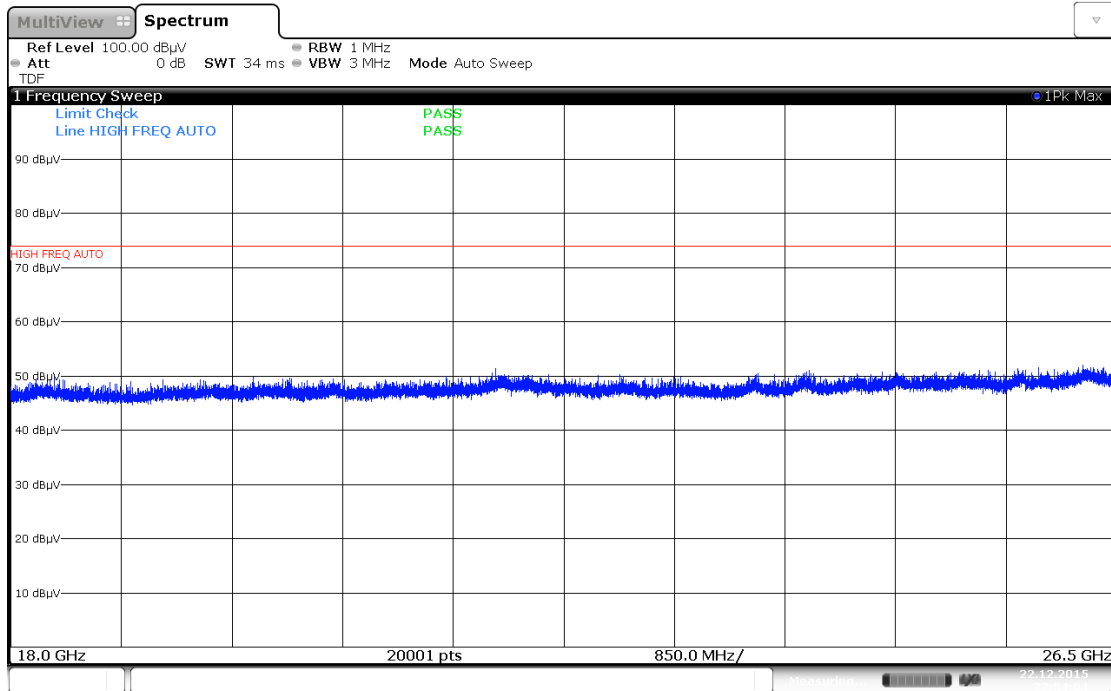
Plot 7-43. Radiated Spurious Plot above 18GHz (Pol. H)
