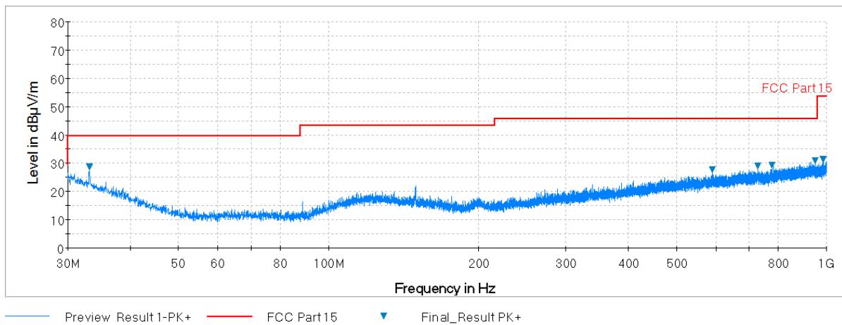
Plot 7-50. Radiated Spurious Plot below 1GHz (Pol. V)
